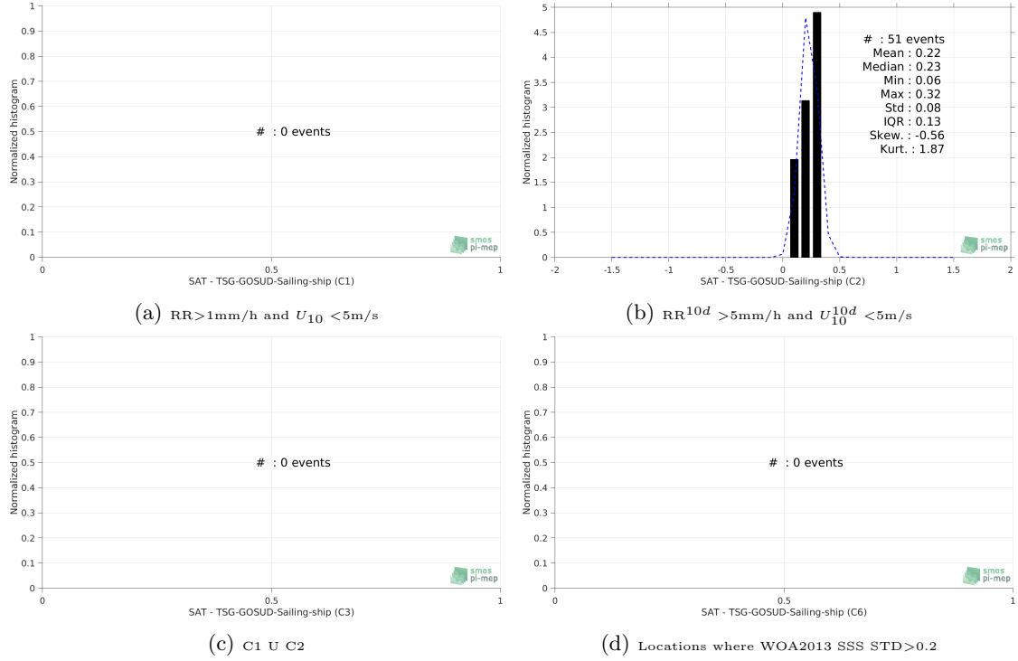
Figure 13: Normalized histogram of \Delta SSS (SMAP-L3-RSS-V3-MONTHLY-70KM - TSG-GOSUD-Sailing-ship) for 6 different subdatasets corresponding to: RR > 1\text{mm/h} and U_{10} < 5\text{m/s} (a), RR^{10d} > 5\text{mm/h} and U_{10}^{10d} < 5\text{m/s} (b), C1 \cup C2 (c), Locations where WOA2013 SSS STD > 0.2 (d).
