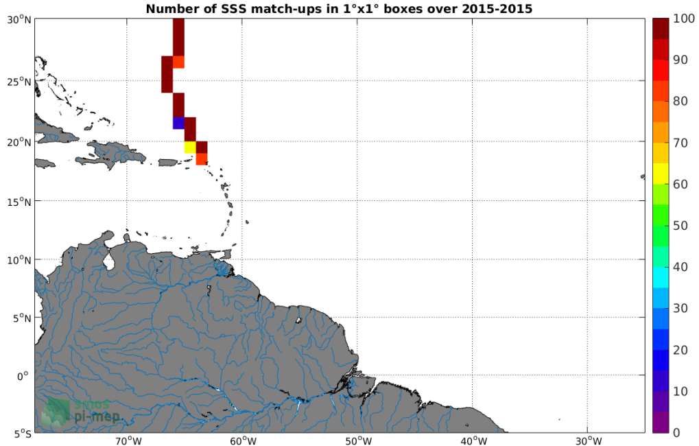
Figure 4: Number of SSS match-ups between TSG-GOSUD-Sailing-ship SSS and the SMAP-L3-RSS-V3-MONTHLY-70KM SSS product for the Amazon and Orinoco river plumes Pi-MEP region over 1^\circ \times 1^\circ boxes and for the full satellite product period.
