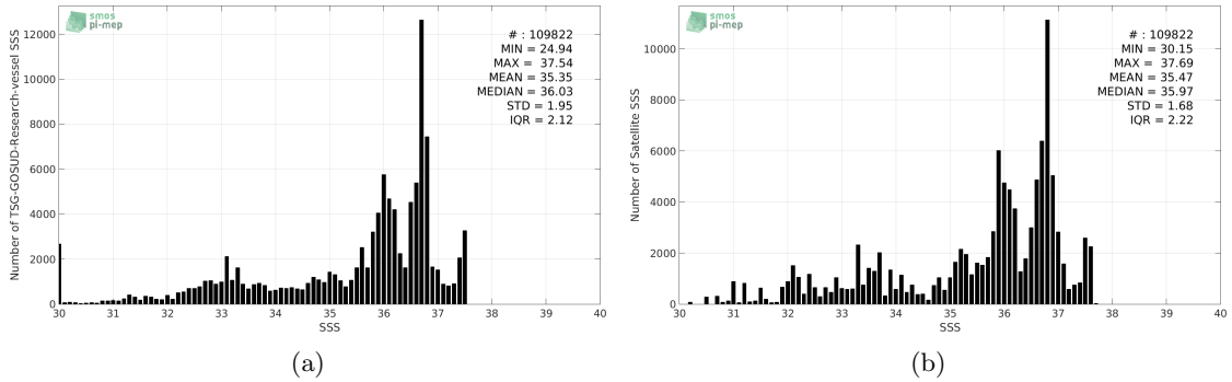
Figure 2: Histograms of SSS from TSG-GOSUD-Research-vessel (a) and SMAP-L3-RSS-V3-MONTHLY-70KM (b) considering all match-up pairs per bins of 0.1 over the Amazon and Orinoco river plumes Pi-MEP region and for the full satellite product period.
