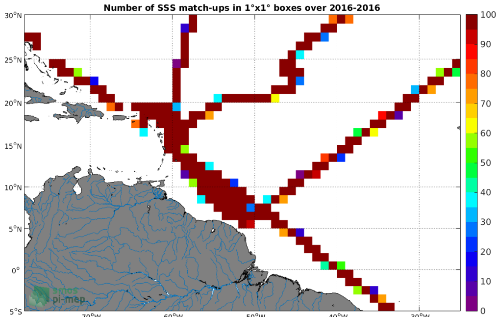
Figure 4: Number of SSS match-ups between TSG-GOSUD-Research-vessel SSS and the SMAP-L3-RSS-V3-MONTHLY-70KM SSS product for the Amazon and Orinoco river plumes Pi-MEP region over 1°x1° boxes and for the full satellite product period.
