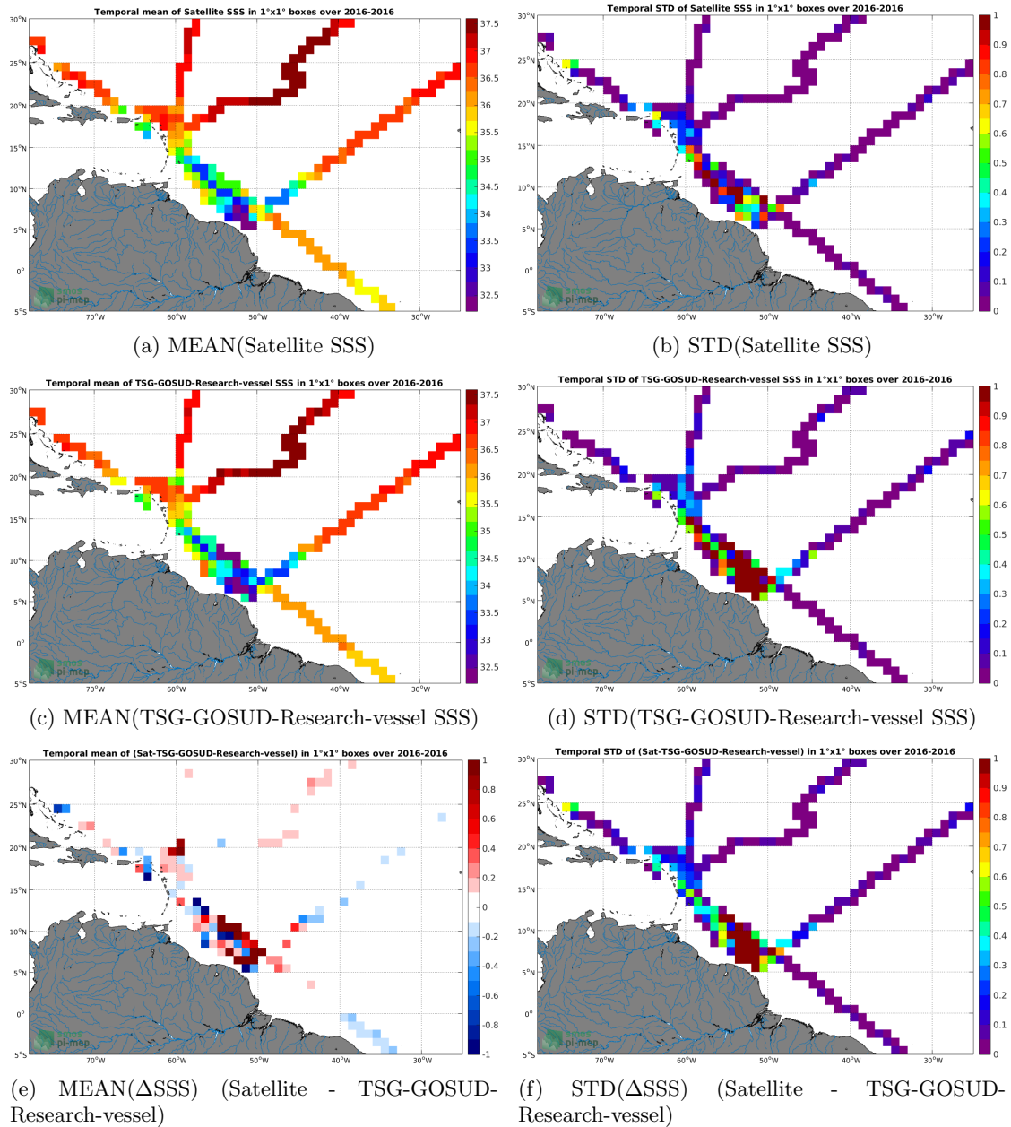
Figure 6: Temporal mean (left) and STD (right) of SSS from SMAP-L3-RSS-V3-MONTHLY-70KM (top), TSG-GOSUD-Research-vessel (middle), and of \Delta SSS (Satellite - TSG-GOSUD-Research-vessel). Only match-up pairs are used to generate these maps.
