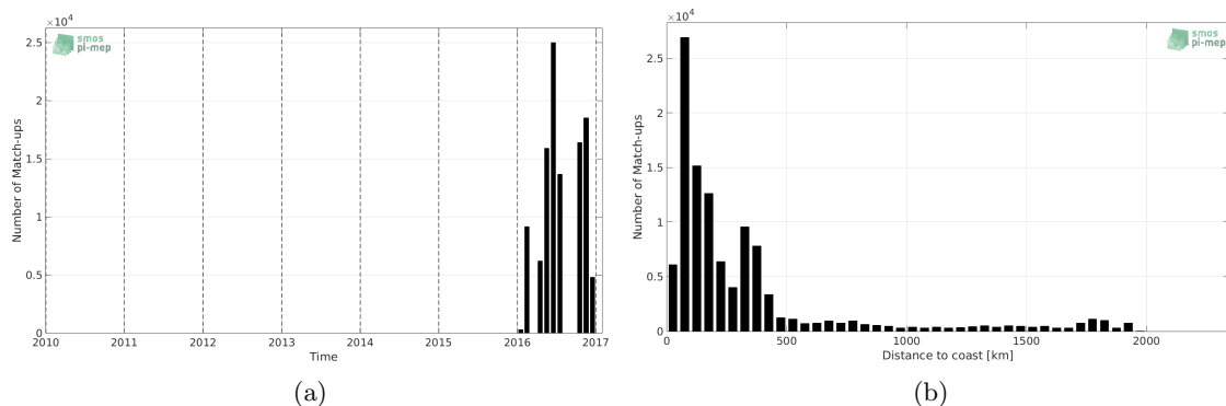
Figure 1: Number of match-ups between TSG-GOSUD-Research-vessel and SMAP-L3-RSS-V3-MONTHLY-70KM SSS as a function of time (a) and as function of the distance to coast (b) over the Amazon and Orinoco river plumes Pi-MEP region and for the full satellite product period.
