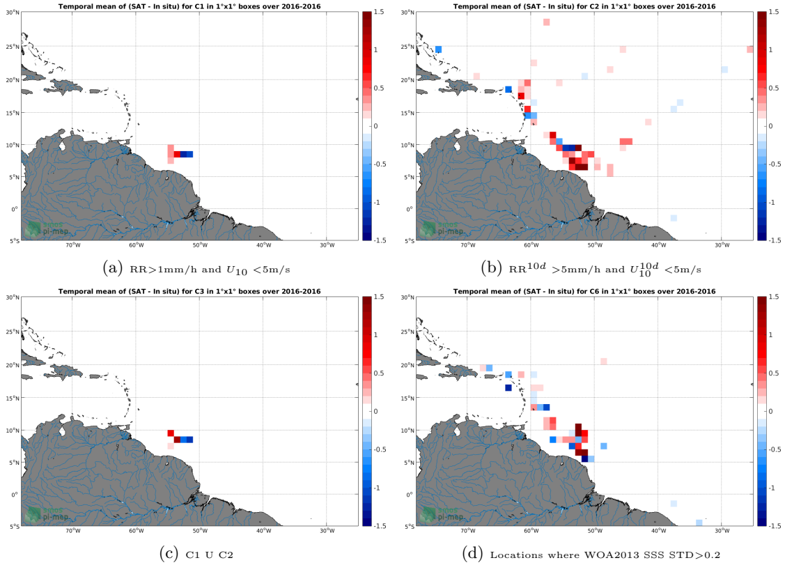
Figure 12: Temporal mean gridded over spatial boxes of size 1^\circ \times 1^\circ of \Delta SSS (SMAP-L3-RSS-V3-MONTHLY-70KM - TSG-GOSUD-Research-vessel) for 4 different subdatasets corresponding to: RR > 1\text{mm/h} and U_{10} < 5\text{m/s} (a), RR^{10d} > 5\text{mm/h} and U_{10}^{10d} < 5\text{m/s} (b), C1 U C2 (c), Locations where WOA2013 SSS STD > 0.2 (d).
