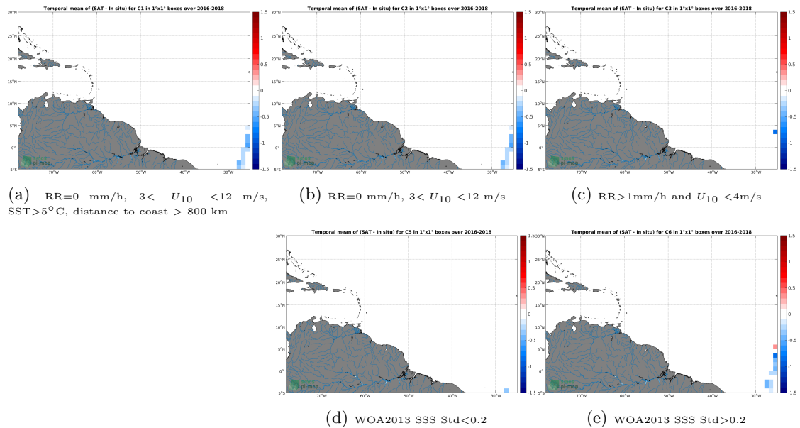
Figure 12: Temporal mean gridded over spatial boxes of size 1^\circ \times 1^\circ of \Delta SSS (SMAP-L3-RSS-V3-MONTHLY-0.25DEG-40KM - TSG-POLARSTERN) for 5 different subdatasets corresponding to:RR=0 mm/h, 3 < U_{10} < 12 m/s, SST >5^\circ\text{C} , distance to coast > 800 km (a), RR=0 mm/h, 3 < U_{10} < 12 m/s (b), RR >1 mm/h and U_{10} < 4 m/s (c), WOA2013 SSS Std <0.2 (d), WOA2013 SSS Std >0.2 (e).
