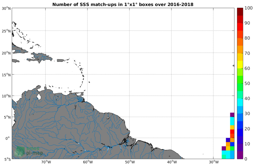
Figure 4: Number of SSS match-ups between TSG-POLARSTERN SSS and the SMAP-L3-RSS-V3-MONTHLY-0.25DEG-40KM SSS product for the Amazon and Orinoco river plumes Pi-MEP region over 1^\circ \times 1^\circ boxes and for the full satellite product period.
