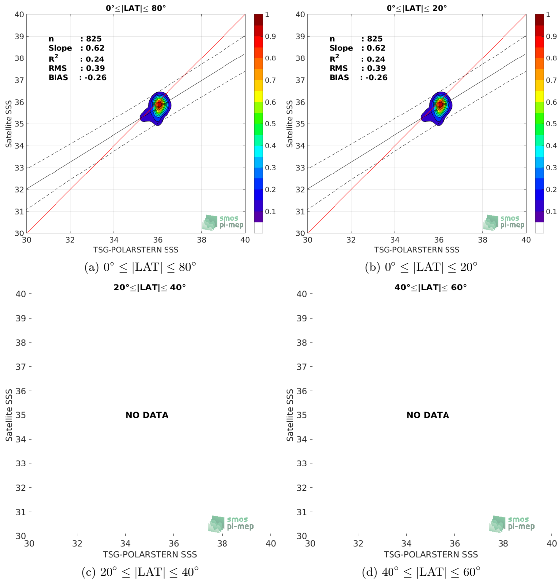
Figure 9: Contour maps of the concentration of SMAP-L3-RSS-V3-MONTHLY-0.25DEG-40KM SSS (y-axis) versus TSG-POLARSTERN SSS (x-axis) at match-up pairs for different latitude bands. For each plot, the red line shows x=y . The black thin and dashed lines indicate a linear fit through the data cloud and the \pm 95\% confidence levels, respectively. The number match-up pairs n , the slope and R^2 coefficient of the linear fit, the root mean square (RMS) and the mean bias between satellite and in situ data are indicated for each latitude band in each plots.
