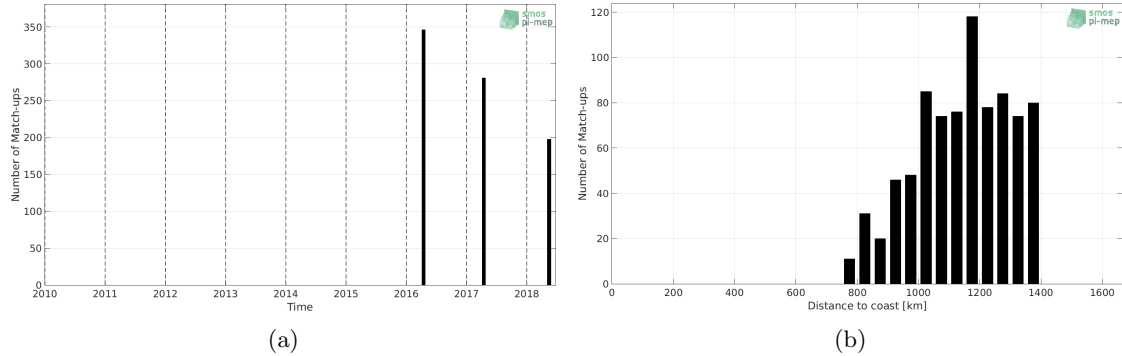
Figure 1: Number of match-ups between TSG-POLARSTERN and SMAP-L3-RSS-V3-MONTHLY-0.25DEG-40KM SSS as a function of time (a) and as function of the distance to coast (b) over the Amazon and Orinoco river plumes Pi-MEP region and for the full satellite product period.
