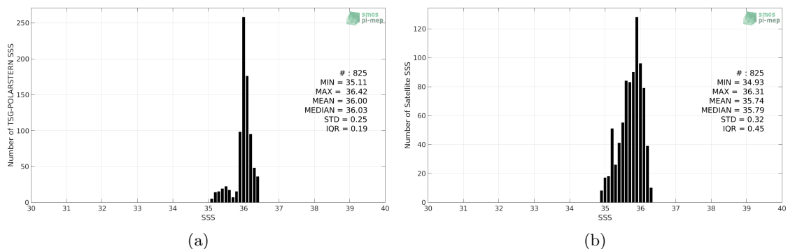
Figure 2: Histograms of SSS from TSG-POLARSTERN (a) and SMAP-L3-RSS-V3-MONTHLY-0.25DEG-40KM (b) considering all match-up pairs per bins of 0.1 over the Amazon and Orinoco river plumes Pi-MEP region and for the full satellite product period.
