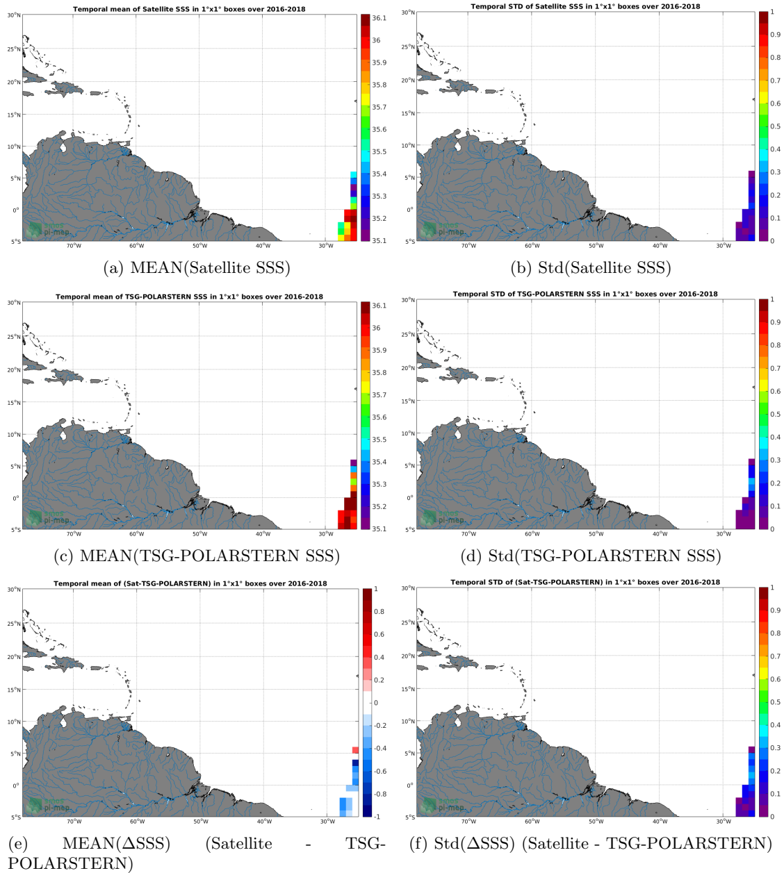
Figure 6: Temporal mean (left) and Std (right) of SSS from SMAP-L3-RSS-V3-MONTHLY-0.25DEG-40KM (top), TSG-POLARSTERN (middle), and of \Delta SSS (Satellite - TSG-POLARSTERN). Only match-up pairs are used to generate these maps.
