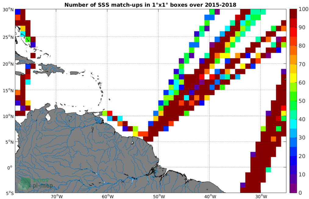
Figure 4: Number of SSS match-ups between TSG-LEGOS-DM SSS and the SMAP-L3-RSS-V3-MONTHLY-0.25DEG-40KM SSS product for the Amazon and Orinoco river plumes Pi-MEP region over 1°x1° boxes and for the full satellite product period.
