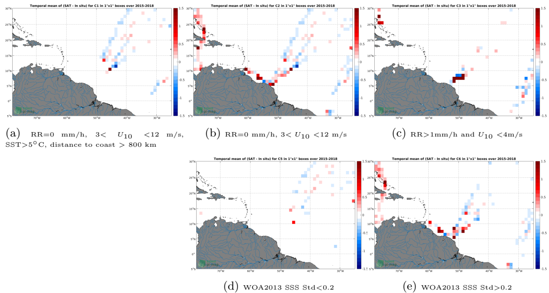
Figure 12: Temporal mean gridded over spatial boxes of size 1^\circ \times 1^\circ of \Delta SSS (SMAP-L3-RSS-V3-MONTHLY-0.25DEG-40KM - TSG-LEGOS-DM) for 5 different subdatasets corresponding to:RR=0 mm/h, 3 < U_{10} < 12 m/s, SST >5^\circ\text{C} , distance to coast > 800 km (a), RR=0 mm/h, 3 < U_{10} < 12 m/s (b), RR >1 mm/h and U_{10} < 4 m/s (c), WOA2013 SSS Std <0.2 (d), WOA2013 SSS Std >0.2 (e).
