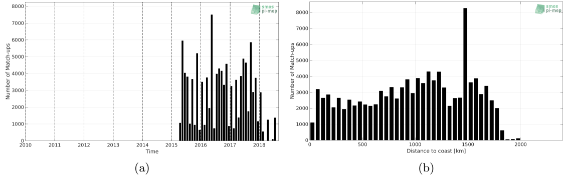
Figure 1: Number of match-ups between TSG-LEGOS-DM and SMAP-L3-RSS-V3-MONTHLY-0.25DEG-40KM SSS as a function of time (a) and as function of the distance to coast (b) over the Amazon and Orinoco river plumes Pi-MEP region and for the full satellite product period.
