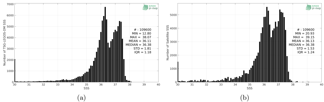
Figure 2: Histograms of SSS from TSG-LEGOS-DM (a) and SMAP-L3-RSS-V3-MONTHLY-0.25DEG-40KM (b) considering all match-up pairs per bins of 0.1 over the Amazon and Orinoco river plumes Pi-MEP region and for the full satellite product period.
