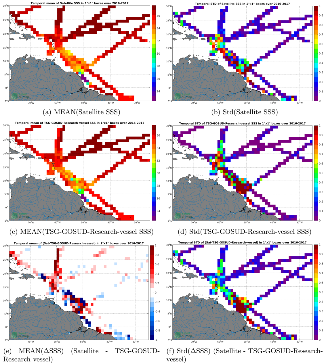
Figure 6: Temporal mean (left) and Std (right) of SSS from SMAP-L3-RSS-V3-MONTHLY-0.25DEG-40KM (top), TSG-GOSUD-Research-vessel (middle), and of \Delta SSS (Satellite - TSG-GOSUD-Research-vessel). Only match-up pairs are used to generate these maps.
