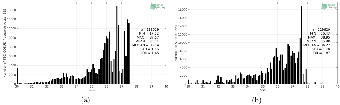
Figure 2: Histograms of SSS from TSG-GOSUD-Research-vessel (a) and SMAP-L3-RSS-V3-MONTHLY-0.25DEG-40KM (b) considering all match-up pairs per bins of 0.1 over the Amazon and Orinoco river plumes Pi-MEP region and for the full satellite product period.
