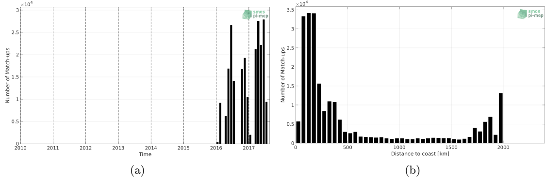
Figure 1: Number of match-ups between TSG-GOSUD-Research-vessel and SMAP-L3-RSS-V3-MONTHLY-0.25DEG-40KM SSS as a function of time (a) and as function of the distance to coast (b) over the Amazon and Orinoco river plumes Pi-MEP region and for the full satellite product period.
