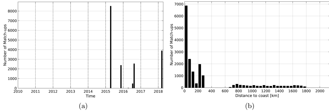
Figure 1: Number of match-ups between TSG-SAMOS and SMAP-L3-RSS-V2-MONTHLY-0.25DEG-40KM SSS as a function of time (a) and as function of the distance to coast (b) over the Amazon and Orinoco river plumes Pi-MEP region and for the full satellite product period.
