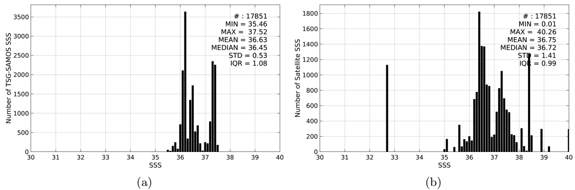
Figure 2: Histograms of SSS from TSG-SAMOS (a) and SMAP-L3-RSS-V2-MONTHLY-0.25DEG-40KM (b) considering all match-up pairs per bins of 0.1 over the Amazon and Orinoco river plumes Pi-MEP region and for the full satellite product period.
