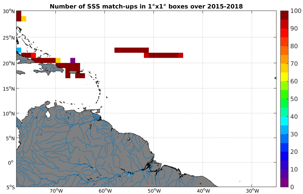
Figure 4: Number of SSS match-ups between TSG-SAMOS SSS and the SMAP-L3-RSS-V2-MONTHLY-0.25DEG-40KM SSS product for the Amazon and Orinoco river plumes Pi-MEP region over 1°x1° boxes and for the full satellite product period.
