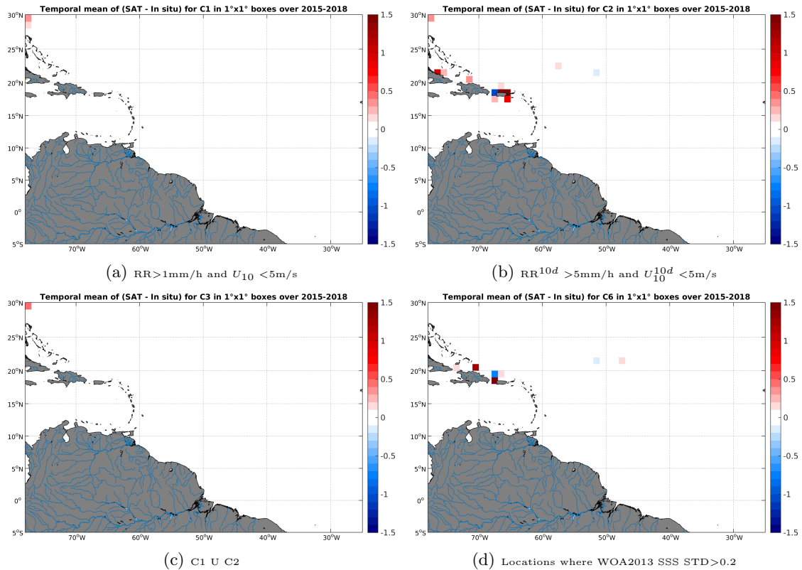
Figure 12: Temporal mean gridded over spatial boxes of size 1^\circ \times 1^\circ of \Delta SSS (SMAP-L3-RSS-V2-MONTHLY-0.25DEG-40KM - TSG-SAMOS) for 4 different subdatasets corresponding to:RR >1 mm/h and U_{10} < 5 m/s (a), RR 10d > 5 mm/h and U_{10}^{10d} < 5 m/s (b), C1 U C2 (c),Locations where WOA2013 SSS STD >0.2 (d).
