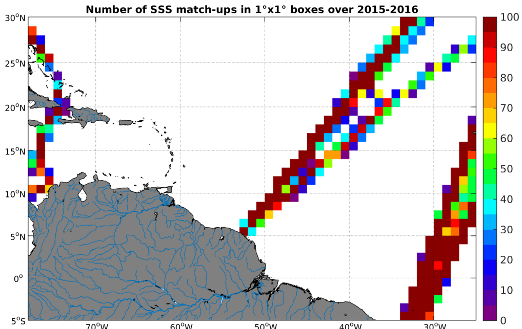
Figure 4: Number of SSS match-ups between TSG-LEGOS-DM SSS and the SMAP-L3-RSS-V2-MONTHLY-0.25DEG-40KM SSS product for the Amazon and Orinoco river plumes Pi-MEP region over 1^\circ \times 1^\circ boxes and for the full satellite product period.
