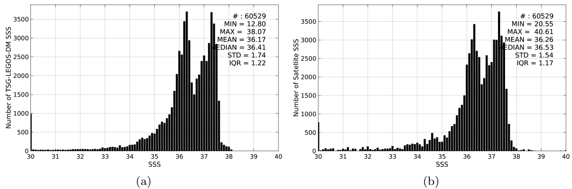
Figure 2: Histograms of SSS from TSG-LEGOS-DM (a) and SMAP-L3-RSS-V2-MONTHLY-0.25DEG-40KM (b) considering all match-up pairs per bins of 0.1 over the Amazon and Orinoco river plumes Pi-MEP region and for the full satellite product period.
