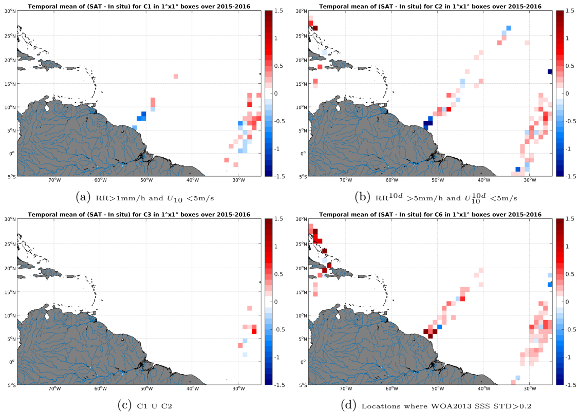
Figure 12: Temporal mean gridded over spatial boxes of size 1^\circ \times 1^\circ of \Delta SSS (SMAP-L3-RSS-V2-MONTHLY-0.25DEG-40KM - TSG-LEGOS-DM) for 4 different subdatasets corresponding to: RR > 1\text{mm/h} and U_{10} < 5\text{m/s} (a), RR^{10d} > 5\text{mm/h} and U_{10}^{10d} < 5\text{m/s} (b), C1 U C2 (c), Locations where WOA2013 SSS STD > 0.2 (d).
