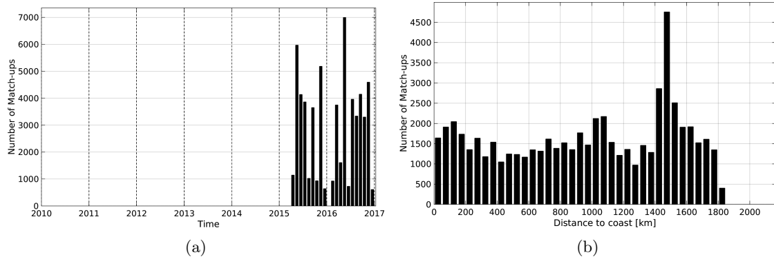
Figure 1: Number of match-ups between TSG-LEGOS-DM and SMAP-L3-RSS-V2-MONTHLY-0.25DEG-40KM SSS as a function of time (a) and as function of the distance to coast (b) over the Amazon and Orinoco river plumes Pi-MEP region and for the full satellite product period.
