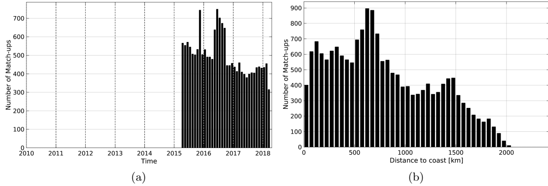
Figure 1: Number of match-ups between Argo and SMAP-L3-RSS-V2-MONTHLY-0.25DEG-40KM SSS as a function of time (a) and as function of the distance to coast (b) over the Amazon and Orinoco river plumes Pi-MEP region and for the full satellite product period.
