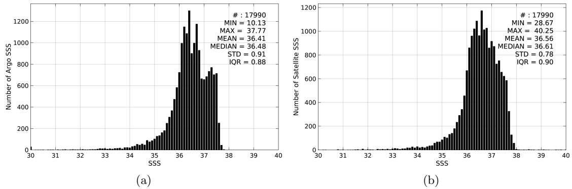
Figure 2: Histograms of SSS from Argo (a) and SMAP-L3-RSS-V2-MONTHLY-0.25DEG-40KM (b) considering all match-up pairs per bins of 0.1 over the Amazon and Orinoco river plumes Pi-MEP region and for the full satellite product period.
