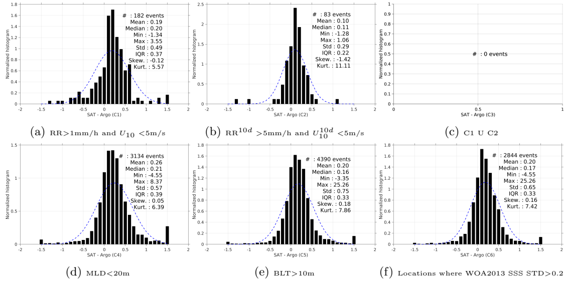
Figure 13: Normalized histogram of \Delta SSS (SMAP-L3-RSS-V2-MONTHLY-0.25DEG-40KM - Argo) for 6 different subdatasets corresponding to: RR>1mm/h and U_{10} < 5 m/s (a), RR^{10d} > 5 mm/h and U_{10}^{10d} < 5 m/s (b), C1 U C2 (c),MLD<20m (d),BLT>10m (e),Locations where WOA2013 SSS STD>0.2 (f).
