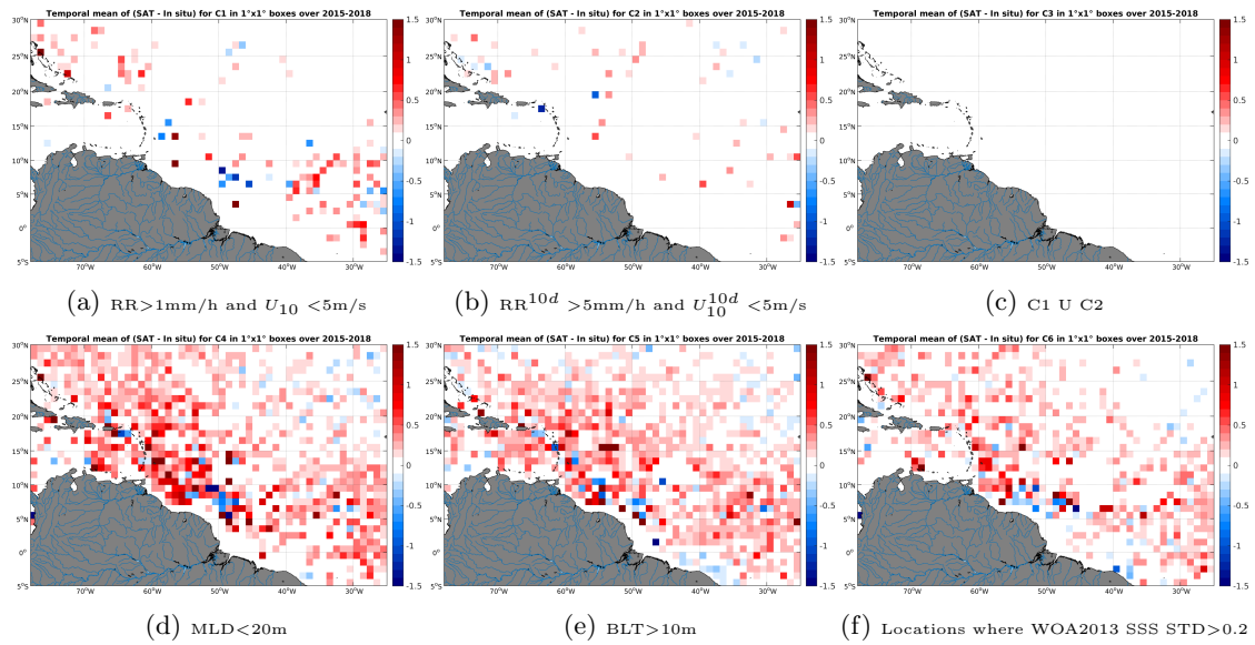
Figure 12: Temporal mean gridded over spatial boxes of size 1^\circ \times 1^\circ of \Delta SSS (SMAP-L3-RSS-V2-MONTHLY-0.25DEG-40KM - Argo) for 6 different subdatasets corresponding to:RR>1mm/h and U_{10} < 5\text{m/s} (a), RR^{10d} > 5\text{mm/h} and U_{10}^{10d} < 5\text{m/s} (b), C1 U C2 (c),MLD<20m (d),BLT>10m (e),Locations where WOA2013 SSS STD>0.2 (f).
