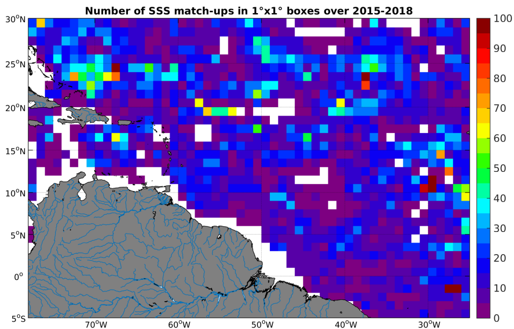
Figure 4: Number of SSS match-ups between Argo SSS and the SMAP-L3-RSS-V2-MONTHLY-0.25DEG-40KM SSS product for the Amazon and Orinoco river plumes Pi-MEP region over 1°x1° boxes and for the full satellite product period.
