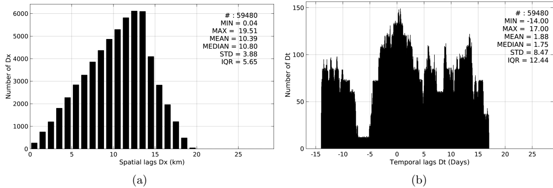
Figure 5: Histograms of the spatial (a) and temporal (b) lags between the time of the TSG-LEGOS-DM measurements and the date of the corresponding SMAP-L3-RSS-V2-MONTHLY-70KM SSS product.
