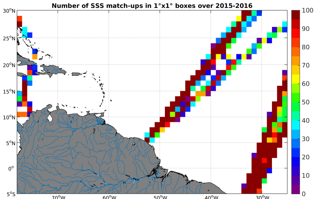
Figure 4: Number of SSS match-ups between TSG-LEGOS-DM SSS and the SMAP-L3-RSS-V2-MONTHLY-70KM SSS product for the Amazon and Orinoco river plumes Pi-MEP region over 1^{\circ} \times 1^{\circ} boxes and for the full satellite product period.
