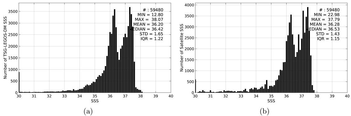
Figure 2: Histograms of SSS from TSG-LEGOS-DM (a) and SMAP-L3-RSS-V2-MONTHLY-70KM (b) considering all match-up pairs per bins of 0.1 over the Amazon and Orinoco river plumes Pi-MEP region and for the full satellite product period.
