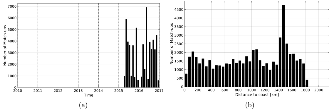
Figure 1: Number of match-ups between TSG-LEGOS-DM and SMAP-L3-RSS-V2-MONTHLY-70KM SSS as a function of time (a) and as function of the distance to coast (b) over the Amazon and Orinoco river plumes Pi-MEP region and for the full satellite product period.
