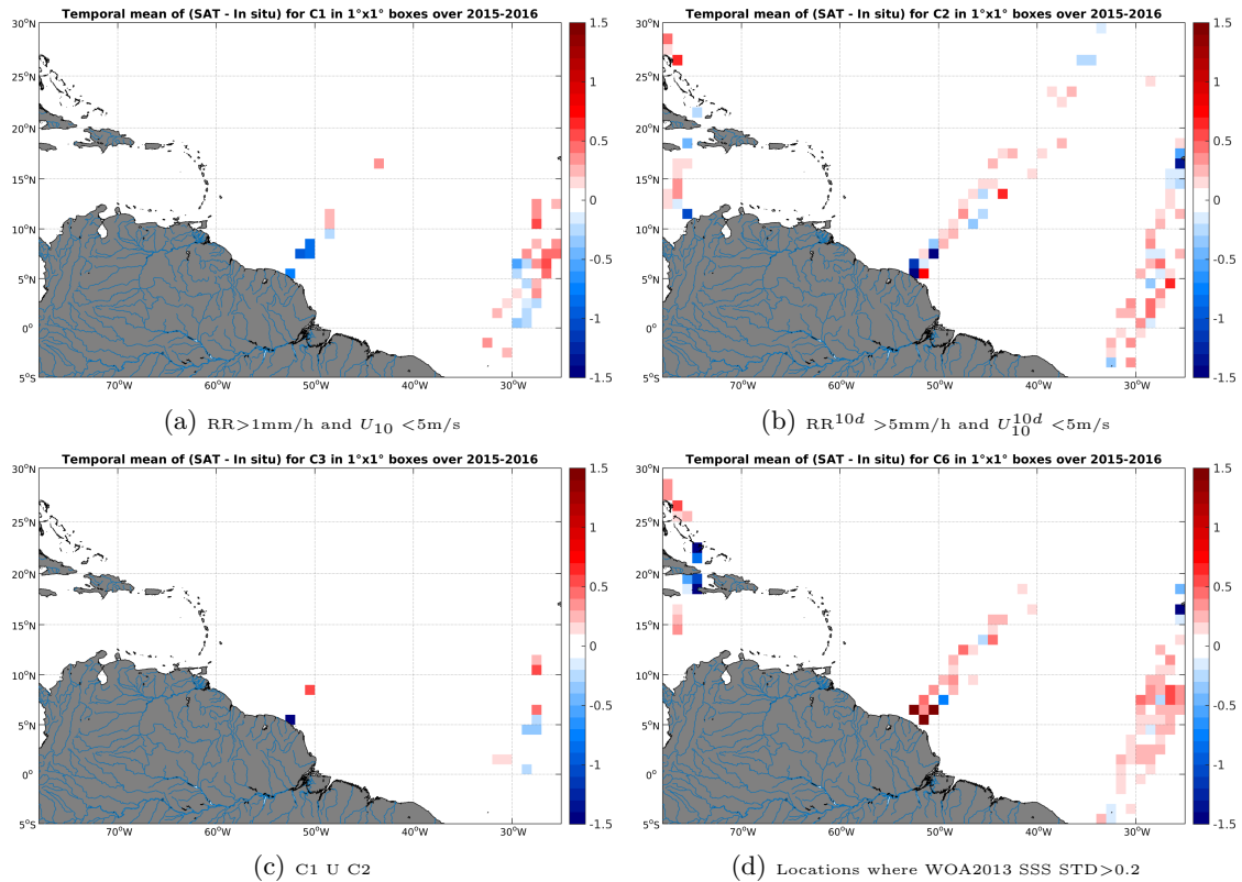
Figure 12: Temporal mean gridded over spatial boxes of size 1^\circ \times 1^\circ of \Delta SSS (SMAP-L3-RSS-V2-MONTHLY-70KM - TSG-LEGOS-DM) for 4 different subdatasets corresponding to:RR > 1 mm/h and U_{10} < 5 m/s (a), RR 10d > 5 mm/h and U_{10}^{10d} < 5 m/s (b), C1 U C2 (c),Locations where WOA2013 SSS STD > 0.2 (d).
