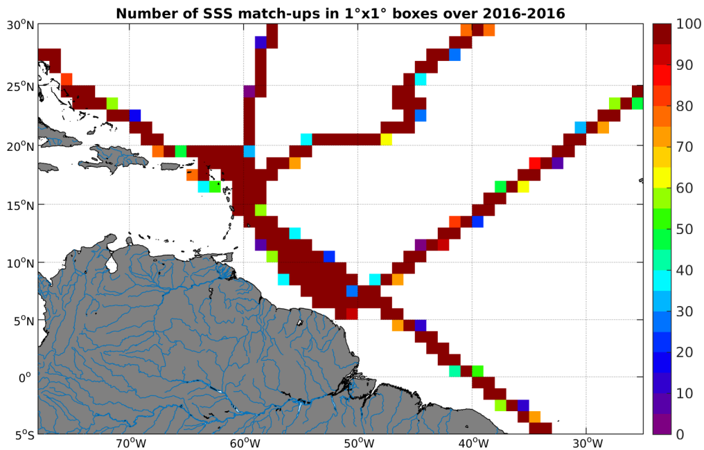
Figure 4: Number of SSS match-ups between TSG-GOSUD-Research-vessel SSS and the SMAP-L3-RSS-V2-MONTHLY-70KM SSS product for the Amazon and Orinoco river plumes Pi-MEP region over 1^\circ \times 1^\circ boxes and for the full satellite product period.
