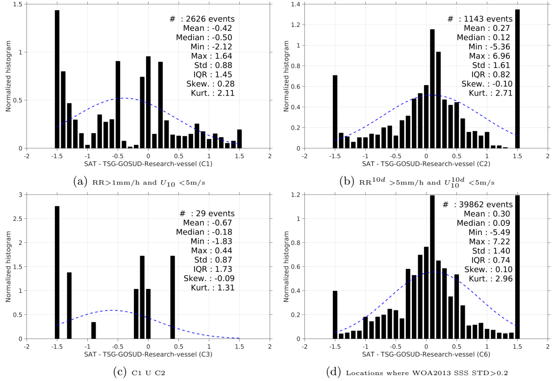
Figure 13: Normalized histogram of \Delta SSS (SMAP-L3-RSS-V2-MONTHLY-70KM - TSG-GOSUD-Research-vessel) for 6 different subdatasets corresponding to: RR > 1\text{mm/h} and U_{10} < 5\text{m/s} (a), RR^{10d} > 5\text{mm/h} and U_{10}^{10d} < 5\text{m/s} (b), C1 \cup C2 (c), Locations where WOA2013 SSS STD > 0.2 (d).
