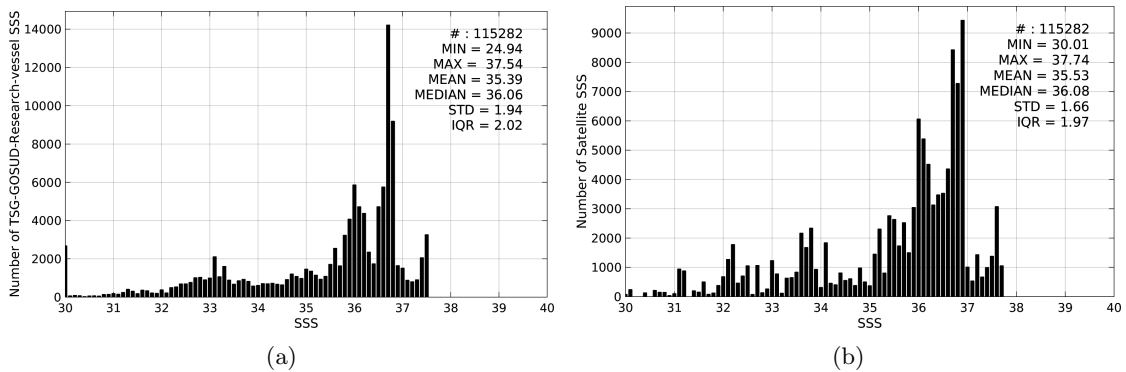
Figure 2: Histograms of SSS from TSG-GOSUD-Research-vessel (a) and SMAP-L3-RSS-V2-MONTHLY-70KM (b) considering all match-up pairs per bins of 0.1 over the Amazon and Orinoco river plumes Pi-MEP region and for the full satellite product period.
