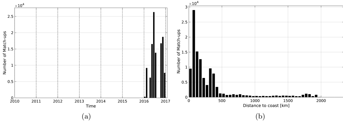
Figure 1: Number of match-ups between TSG-GOSUD-Research-vessel and SMAP-L3-RSS-V2-MONTHLY-70KM SSS as a function of time (a) and as function of the distance to coast (b) over the Amazon and Orinoco river plumes Pi-MEP region and for the full satellite product period.
