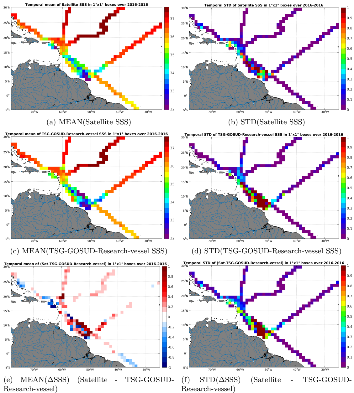
Figure 6: Temporal mean (left) and STD (right) of SSS from SMAP-L3-RSS-V2-MONTHLY-70KM (top), TSG-GOSUD-Research-vessel (middle), and of \Delta SSS (Satellite - TSG-GOSUD-Research-vessel). Only match-up pairs are used to generate these maps.
