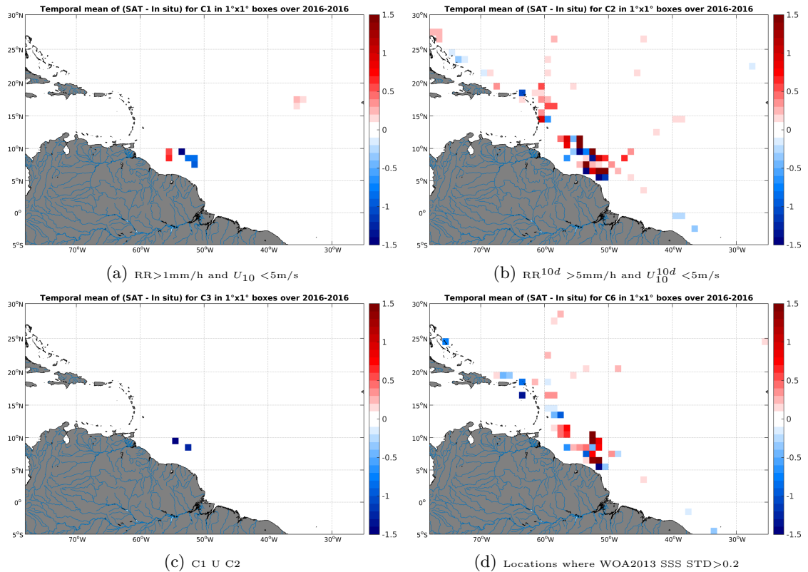
Figure 12: Temporal mean gridded over spatial boxes of size 1^\circ \times 1^\circ of \Delta SSS (SMAP-L3-RSS-V2-MONTHLY-70KM - TSG-GOSUD-Research-vessel) for 4 different subdatasets corresponding to: RR > 1\text{mm/h} and U_{10} < 5\text{m/s} (a), RR^{10d} > 5\text{mm/h} and U_{10}^{10d} < 5\text{m/s} (b), C1 U C2 (c), Locations where WOA2013 SSS STD > 0.2 (d).
