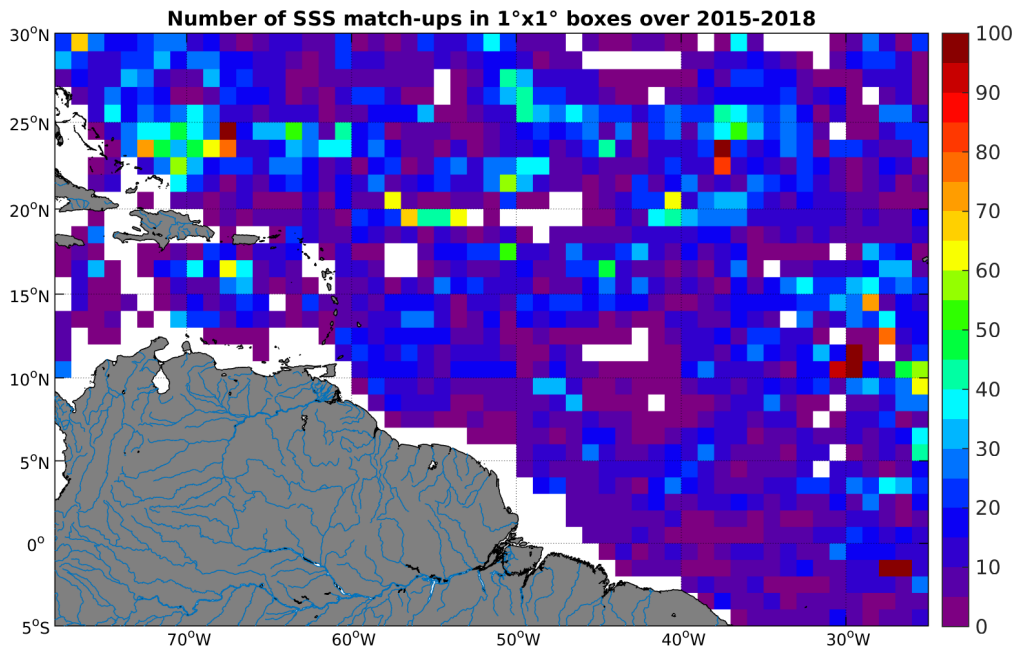
Figure 4: Number of SSS match-ups between Argo SSS and the SMAP-L3-RSS-V2-MONTHLY-70KM SSS product for the Amazon and Orinoco river plumes Pi-MEP region over 1°x1° boxes and for the full satellite product period.
