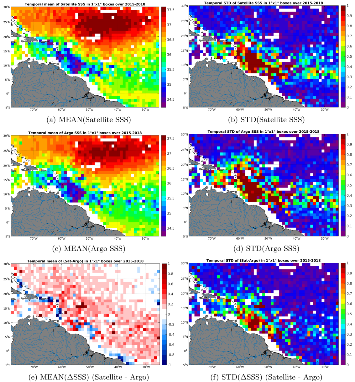
Figure 6: Temporal mean (left) and STD (right) of SSS from SMAP-L3-RSS-V2-MONTHLY-70KM (top), Argo (middle), and of \Delta SSS (Satellite - Argo). Only match-up pairs are used to generate these maps.
