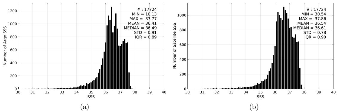
Figure 2: Histograms of SSS from Argo (a) and SMAP-L3-RSS-V2-MONTHLY-70KM (b) considering all match-up pairs per bins of 0.1 over the Amazon and Orinoco river plumes Pi-MEP region and for the full satellite product period.
