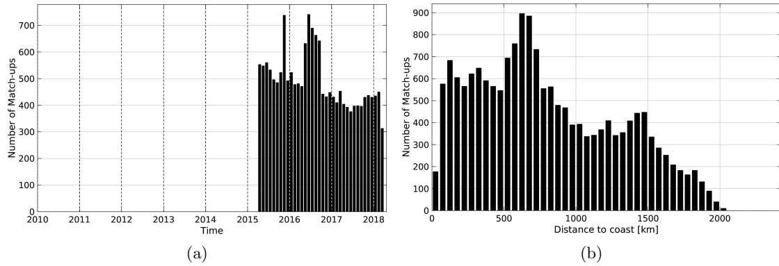
Figure 1: Number of match-ups between Argo and SMAP-L3-RSS-V2-MONTHLY-70KM SSS as a function of time (a) and as function of the distance to coast (b) over the Amazon and Orinoco river plumes Pi-MEP region and for the full satellite product period.
