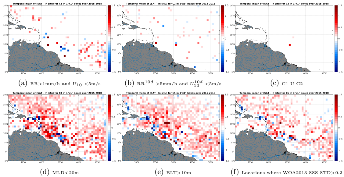
Figure 12: Temporal mean gridded over spatial boxes of size 1^\circ \times 1^\circ of \Delta SSS (SMAP-L3-RSS-V2-MONTHLY-70KM - Argo) for 6 different subdatasets corresponding to:RR>1mm/h and U_{10} < 5\text{m/s} (a), RR^{10d} > 5\text{mm/h} and U_{10}^{10d} < 5\text{m/s} (b), C1 U C2 (c),MLD<20m (d),BLT>10m (e),Locations where WOA2013 SSS STD>0.2 (f).
