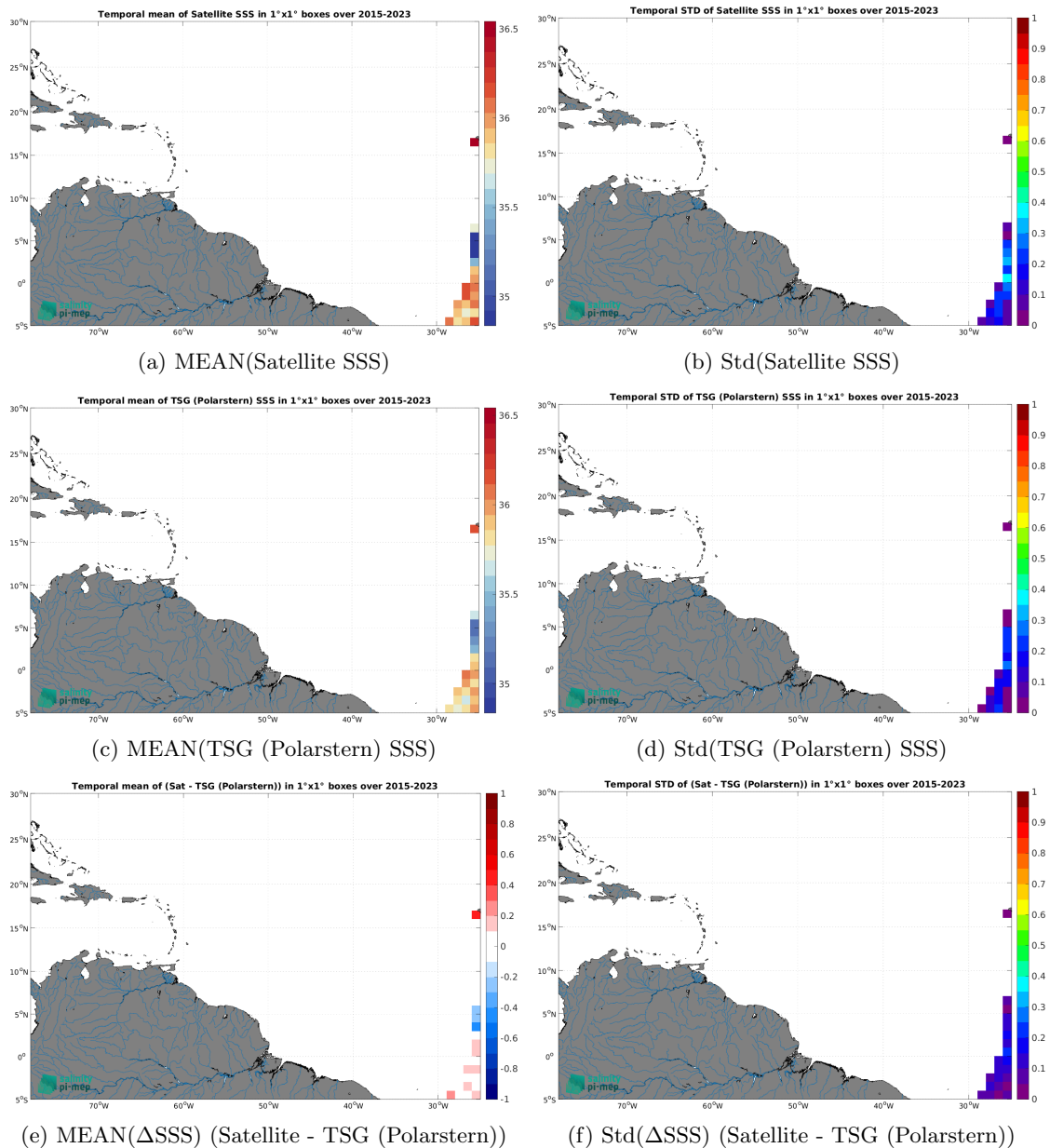
Figure 7: Temporal mean (left) and Std (right) of SSS from SMAP SSS L3 v5.0 - 8-Day running (JPL) (top), TSG (Polarstern) (middle), and of \Delta SSS (Satellite - TSG (Polarstern)). Only match-up pairs are used to generate these maps.
