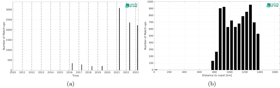
Figure 2: Number of match-ups between TSG (Polarstern) and SMAP SSS L3 v5.0 - 8-Day running (JPL) SSS as a function of time (a) and as function of the distance to coast (b) over the Amazon and Orinoco river plumes Pi-MEP region and for the full satellite product period.
