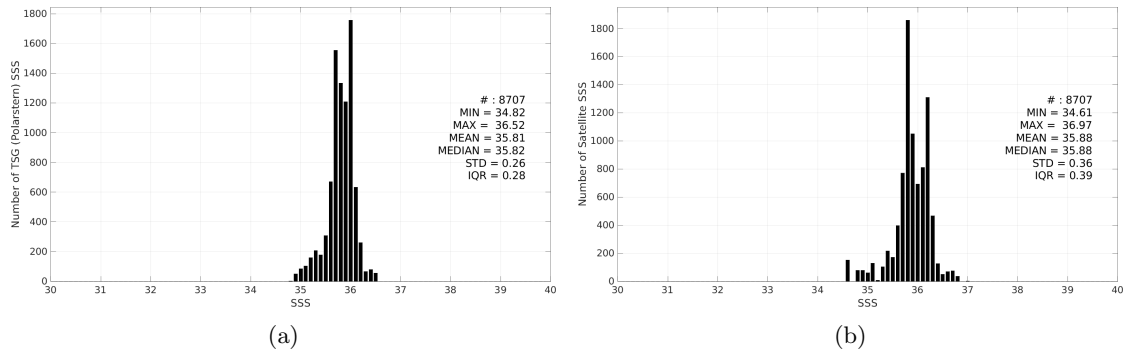
Figure 3: Histograms of SSS from TSG (Polarstern) (a) and SMAP SSS L3 v5.0 - 8-Day running (JPL) (b) considering all match-up pairs per bins of 0.1 over the Amazon and Orinoco river plumes Pi-MEP region and for the full satellite product period.
