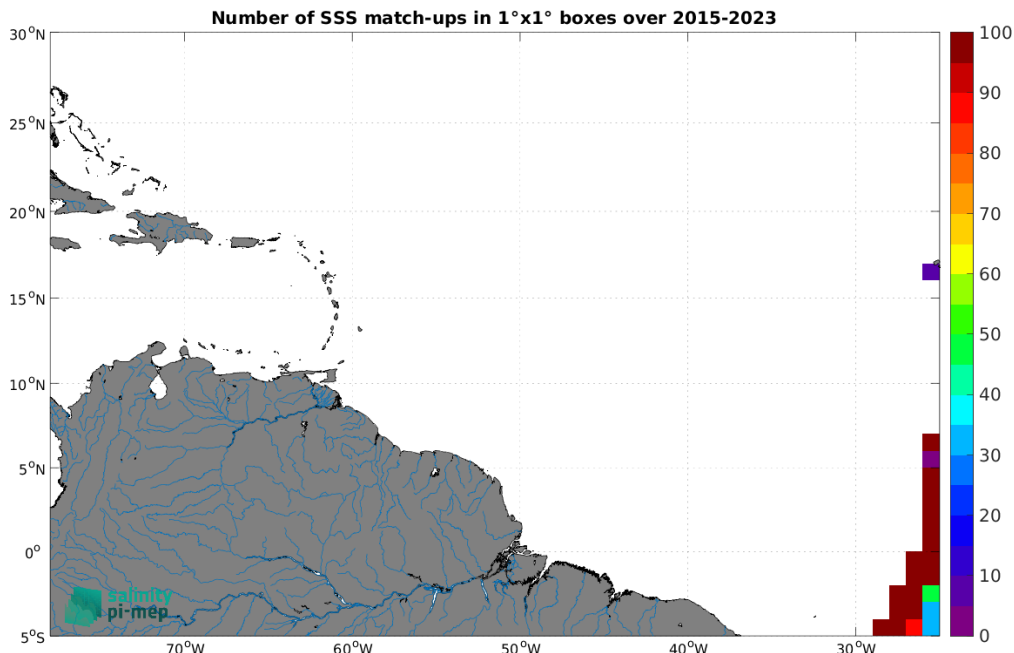
Figure 5: Number of SSS match-ups between TSG (Polarstern) SSS and the SMAP SSS L3 v5.0 - 8-Day running (JPL) SSS product for the Amazon and Orinoco river plumes Pi-MEP region over 1^\circ \times 1^\circ boxes and for the full satellite product period.
