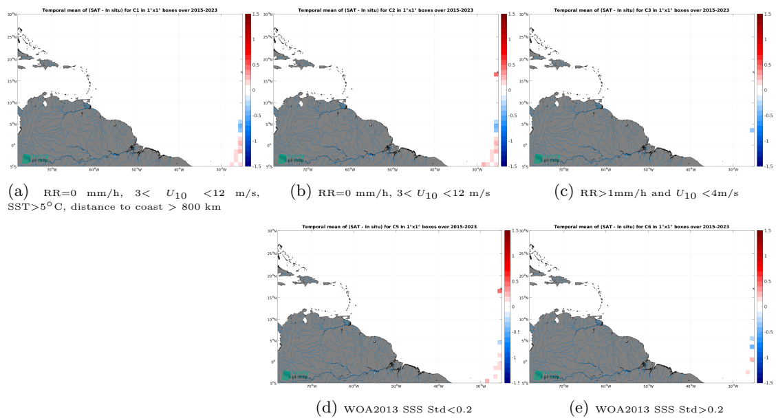
Figure 14: Temporal mean gridded over spatial boxes of size 1^\circ \times 1^\circ of \Delta SSS (SMAP SSS L3 v5.0 - 8-Day running (JPL) - TSG (Polarstern)) for 5 different subdatasets corresponding to:RR=0 mm/h, 3 < U_{10} < 12 m/s, SST >5^\circ\text{C} , distance to coast > 800 km (a), RR=0 mm/h, 3 < U_{10} < 12 m/s (b), RR >1 mm/h and U_{10} < 4 m/s (c), WOA2013 SSS Std <0.2 (d), WOA2013 SSS Std >0.2 (e).
