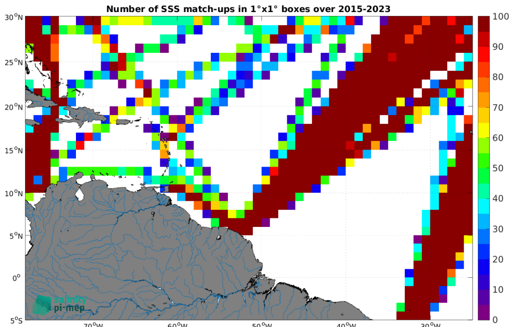
Figure 5: Number of SSS match-ups between TSG (LEGOS-DM) SSS and the SMAP SSS L3 v5.0 - 8-Day running (JPL) SSS product for the Amazon and Orinoco river plumes Pi-MEP region over 1^\circ \times 1^\circ boxes and for the full satellite product period.
