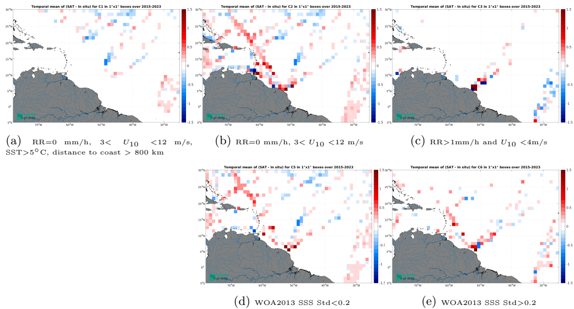
Figure 14: Temporal mean gridded over spatial boxes of size 1^\circ \times 1^\circ of \Delta SSS (SMAP SSS L3 v5.0 - 8-Day running (JPL) - TSG (LEGOS-DM)) for 5 different subdatasets corresponding to:RR=0 mm/h, 3 < U_{10} < 12 m/s, SST >5^\circ\text{C} , distance to coast > 800 km (a), RR=0 mm/h, 3 < U_{10} < 12 m/s (b), RR >1 mm/h and U_{10} < 4 m/s (c), WOA2013 SSS Std <0.2 (d), WOA2013 SSS Std >0.2 (e).
