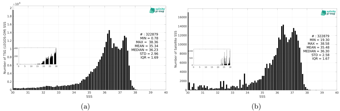
Figure 3: Histograms of SSS from TSG (LEGOS-DM) (a) and SMAP SSS L3 v5.0 - 8-Day running (JPL) (b) considering all match-up pairs per bins of 0.1 over the Amazon and Orinoco river plumes Pi-MEP region and for the full satellite product period.
