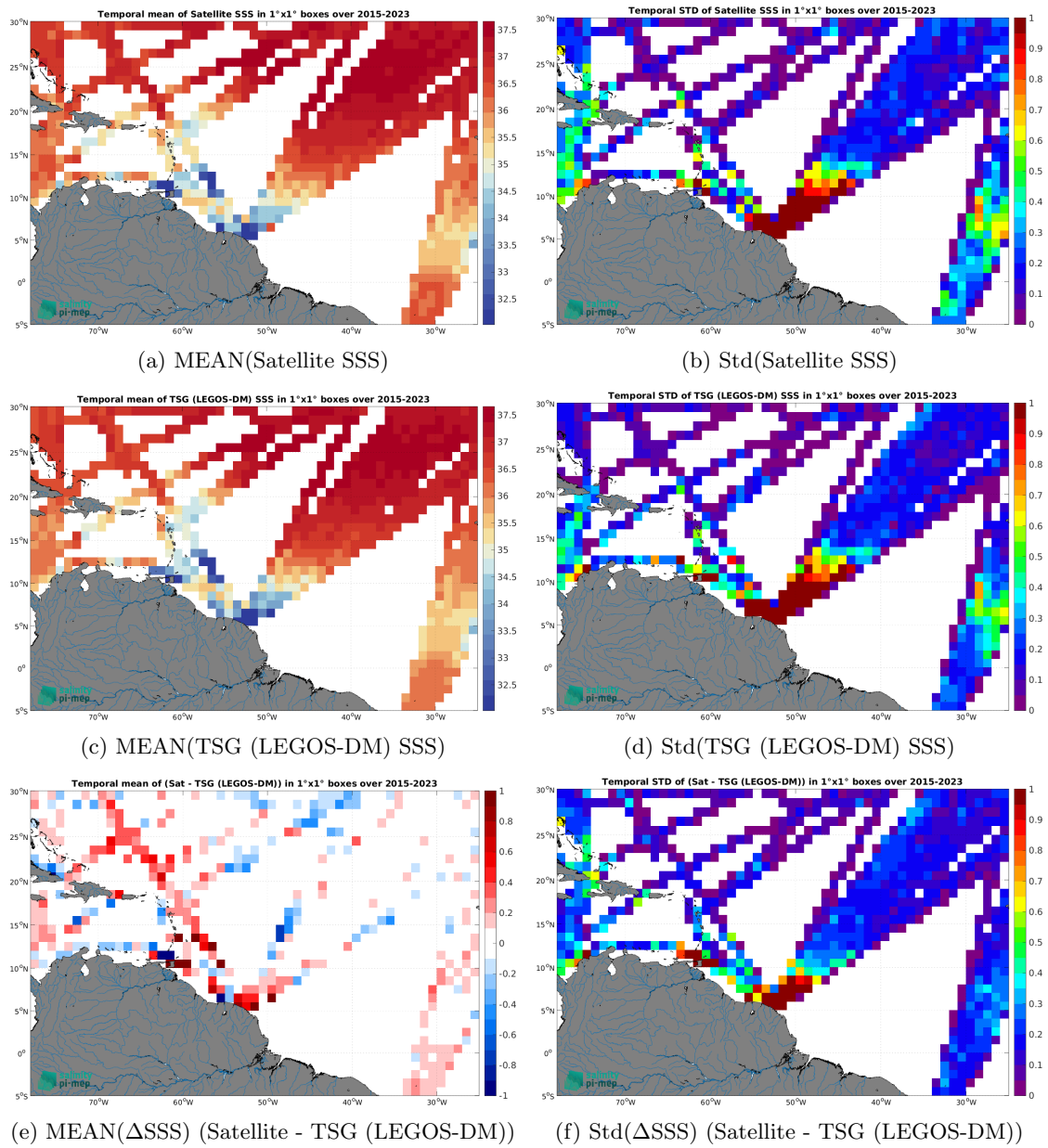
Figure 7: Temporal mean (left) and Std (right) of SSS from SMAP SSS L3 v5.0 - 8-Day running (JPL) (top), TSG (LEGOS-DM) (middle), and of \Delta SSS (Satellite - TSG (LEGOS-DM)). Only match-up pairs are used to generate these maps.
