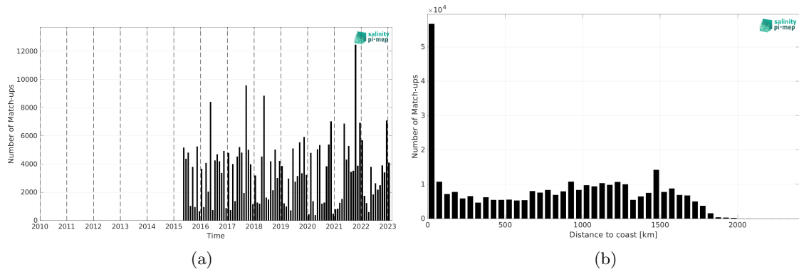
Figure 2: Number of match-ups between TSG (LEGOS-DM) and SMAP SSS L3 v5.0 - 8-Day running (JPL) SSS as a function of time (a) and as function of the distance to coast (b) over the Amazon and Orinoco river plumes Pi-MEP region and for the full satellite product period.
