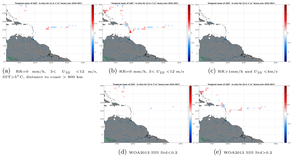
Figure 12: Temporal mean gridded over spatial boxes of size 1°x1° of \Delta SSS (SMAP SSS L3 v5.0 - 8-Day running (JPL) - TSG (GOSUD-Sailing-ship)) for 5 different subdatasets corresponding to:RR=0 mm/h, 3 < U_{10} < 12 m/s, SST>5°C, distance to coast > 800 km (a), RR=0 mm/h, 3 < U_{10} < 12 m/s (b), RR>1mm/h and U_{10} < 4 m/s (c), WOA2013 SSS Std<0.2 (d), WOA2013 SSS Std>0.2 (e).
