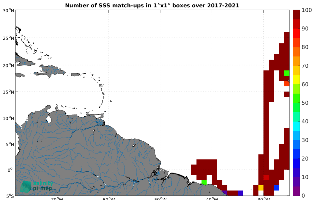
Figure 5: Number of SSS match-ups between TSG (CSIC-UTM) SSS and the SMAP SSS L3 v5.0 - 8-Day running (JPL) SSS product for the Amazon and Orinoco river plumes Pi-MEP region over 1^\circ \times 1^\circ boxes and for the full satellite product period.
