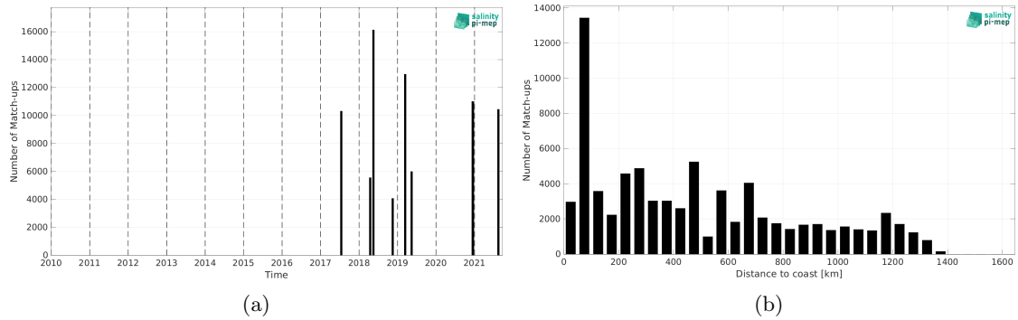
Figure 2: Number of match-ups between TSG (CSIC-UTM) and SMAP SSS L3 v5.0 - 8-Day running (JPL) SSS as a function of time (a) and as function of the distance to coast (b) over the Amazon and Orinoco river plumes Pi-MEP region and for the full satellite product period.
