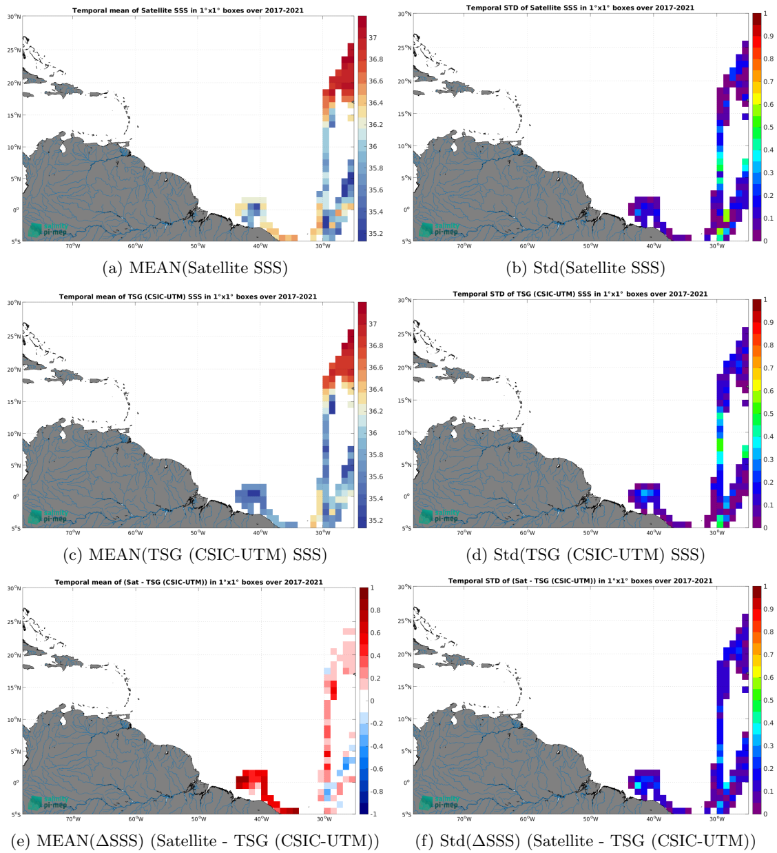
Figure 7: Temporal mean (left) and Std (right) of SSS from SMAP SSS L3 v5.0 - 8-Day running (JPL) (top), TSG (CSIC-UTM) (middle), and of \Delta SSS (Satellite - TSG (CSIC-UTM)). Only match-up pairs are used to generate these maps.
