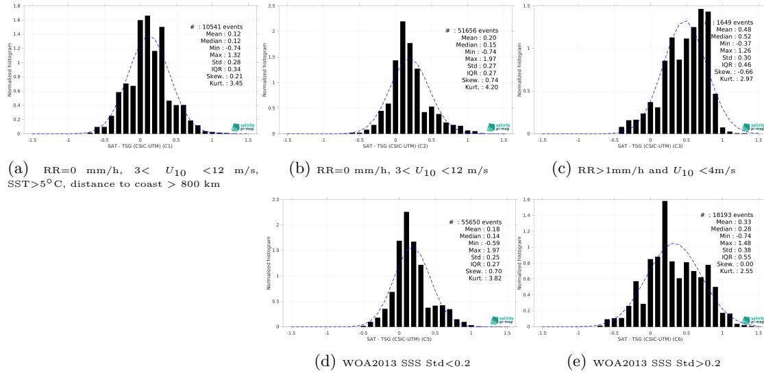
Figure 15: Normalized histogram of \Delta SSS (SMAP SSS L3 v5.0 - 8-Day running (JPL) - TSG (CSIC-UTM)) for 5 different subdatasets corresponding to: RR=0 mm/h, 3 < U_{10} < 12 m/s, SST>5°C, distance to coast > 800 km (a), RR=0 mm/h, 3 < U_{10} < 12 m/s (b), RR>1mm/h and U_{10} < 4 m/s (c), WOA2013 SSS Std<0.2 (d), WOA2013 SSS Std>0.2 (e).
