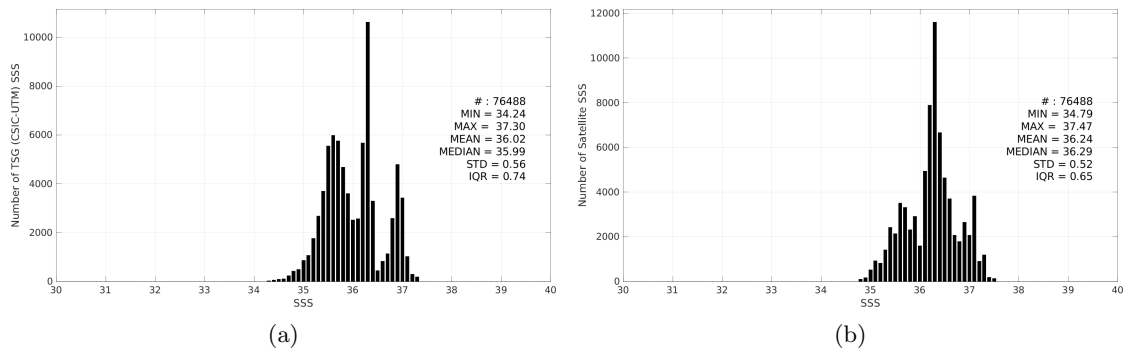
Figure 3: Histograms of SSS from TSG (CSIC-UTM) (a) and SMAP SSS L3 v5.0 - 8-Day running (JPL) (b) considering all match-up pairs per bins of 0.1 over the Amazon and Orinoco river plumes Pi-MEP region and for the full satellite product period.
