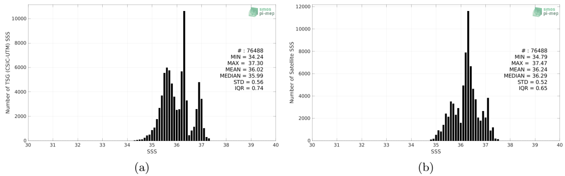
Figure 2: Histograms of SSS from TSG (CSIC-UTM) (a) and SMAP SSS L3 v5.0 - 8-Day running (JPL) (b) considering all match-up pairs per bins of 0.1 over the Amazon and Orinoco river plumes Pi-MEP region and for the full satellite product period.
