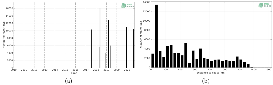
Figure 1: Number of match-ups between TSG (CSIC-UTM) and SMAP SSS L3 v5.0 - 8-Day running (JPL) SSS as a function of time (a) and as function of the distance to coast (b) over the Amazon and Orinoco river plumes Pi-MEP region and for the full satellite product period.
