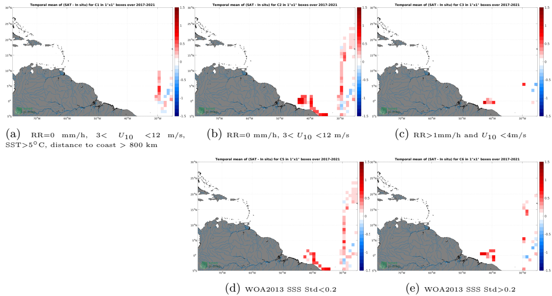
Figure 12: Temporal mean gridded over spatial boxes of size 1^\circ \times 1^\circ of \Delta SSS (SMAP SSS L3 v5.0 - 8-Day running (JPL) - TSG (CSIC-UTM)) for 5 different subdatasets corresponding to:RR=0 mm/h, 3 < U_{10} < 12 m/s, SST >5^\circ\text{C} , distance to coast > 800 km (a), RR=0 mm/h, 3 < U_{10} < 12 m/s (b), RR >1 mm/h and U_{10} < 4 m/s (c), WOA2013 SSS Std <0.2 (d), WOA2013 SSS Std >0.2 (e).
