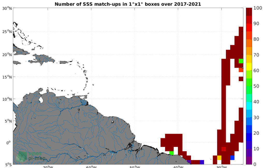
Figure 4: Number of SSS match-ups between TSG (CSIC-UTM) SSS and the SMAP SSS L3 v5.0 - 8-Day running (JPL) SSS product for the Amazon and Orinoco river plumes Pi-MEP region over 1^\circ \times 1^\circ boxes and for the full satellite product period.
