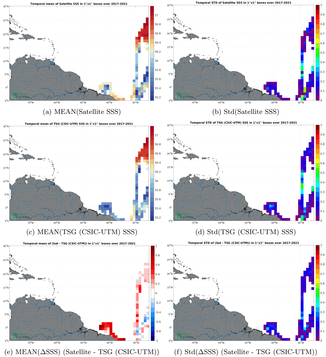
Figure 6: Temporal mean (left) and Std (right) of SSS from SMAP SSS L3 v5.0 - 8-Day running (JPL) (top), TSG (CSIC-UTM) (middle), and of \Delta SSS (Satellite - TSG (CSIC-UTM)). Only match-up pairs are used to generate these maps.
