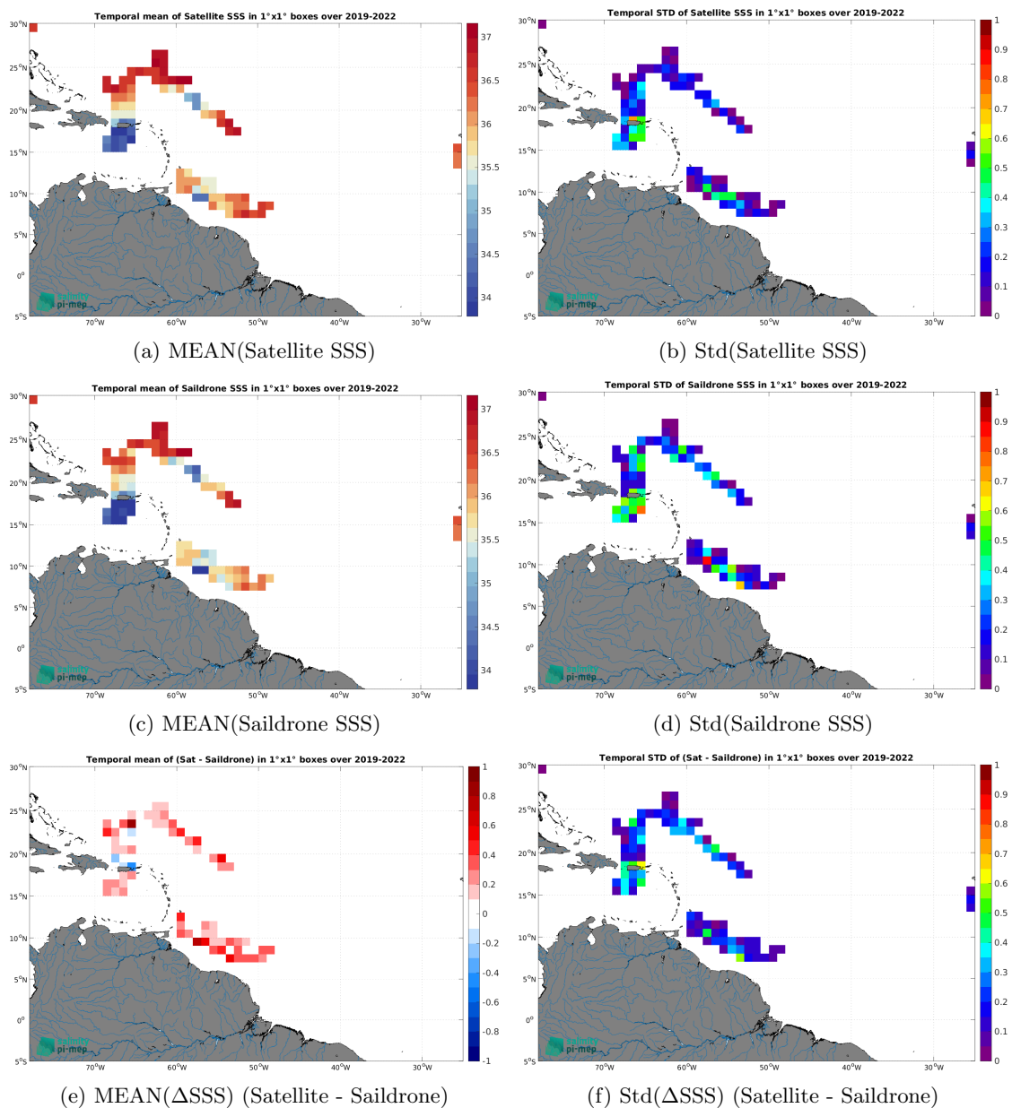
Figure 6: Temporal mean (left) and Std (right) of SSS from SMAP SSS L3 v5.0 - 8-Day running (JPL) (top), Saildrone (middle), and of \Delta SSS (Satellite - Saildrone). Only match-up pairs are used to generate these maps.
