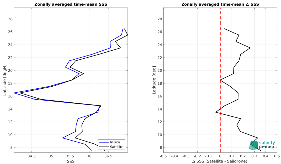
Figure 8: Left panel: Zonal mean SSS from SMAP SSS L3 v5.0 - 8-Day running (JPL) satellite product (black) and from Saildrone (blue). Right panel: Zonal mean of \Delta SSS (Satellite - Saildrone) for all the collected Pi-MEP match-up pairs estimated over the full satellite product period.
