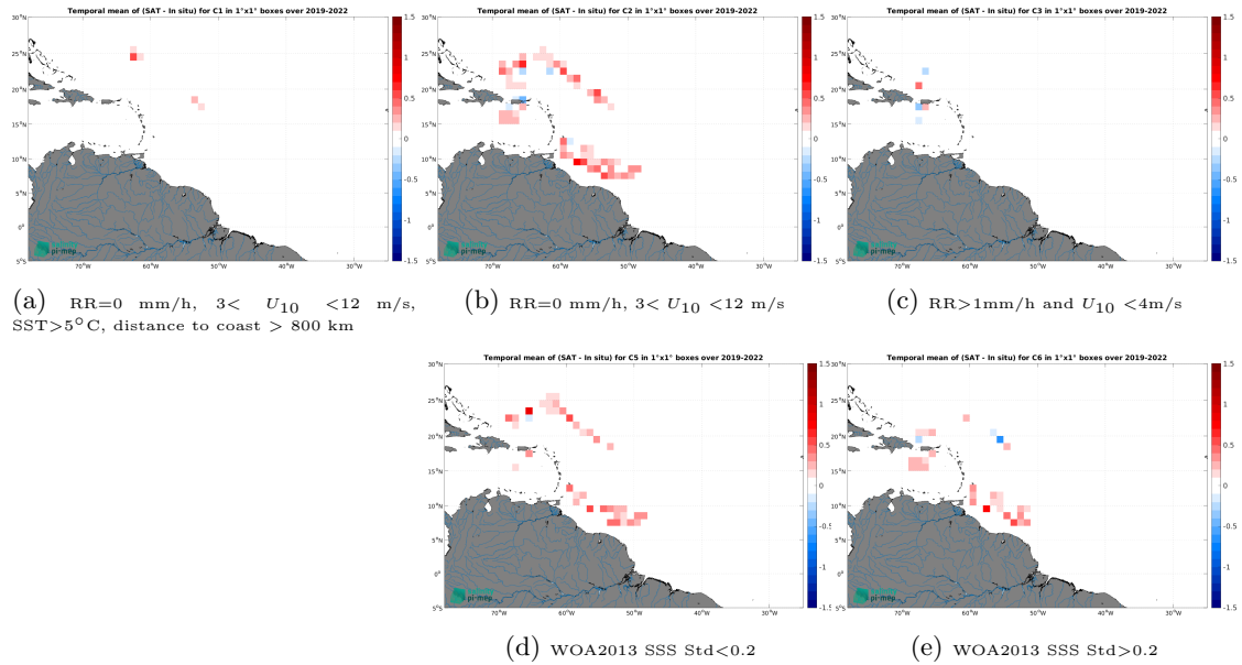
Figure 12: Temporal mean gridded over spatial boxes of size 1^\circ \times 1^\circ of \Delta SSS (SMAP SSS L3 v5.0 - 8-Day running (JPL) - Saildrone) for 5 different subdatasets corresponding to:RR=0 mm/h, 3 < U_{10} < 12 m/s, SST >5^\circ\text{C} , distance to coast > 800 km (a), RR=0 mm/h, 3 < U_{10} < 12 m/s (b), RR >1 mm/h and U_{10} < 4 m/s (c), WOA2013 SSS Std <0.2 (d), WOA2013 SSS Std >0.2 (e).
