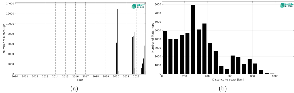
Figure 1: Number of match-ups between Saildrone and SMAP SSS L3 v5.0 - 8-Day running (JPL) SSS as a function of time (a) and as function of the distance to coast (b) over the Amazon and Orinoco river plumes Pi-MEP region and for the full satellite product period.
