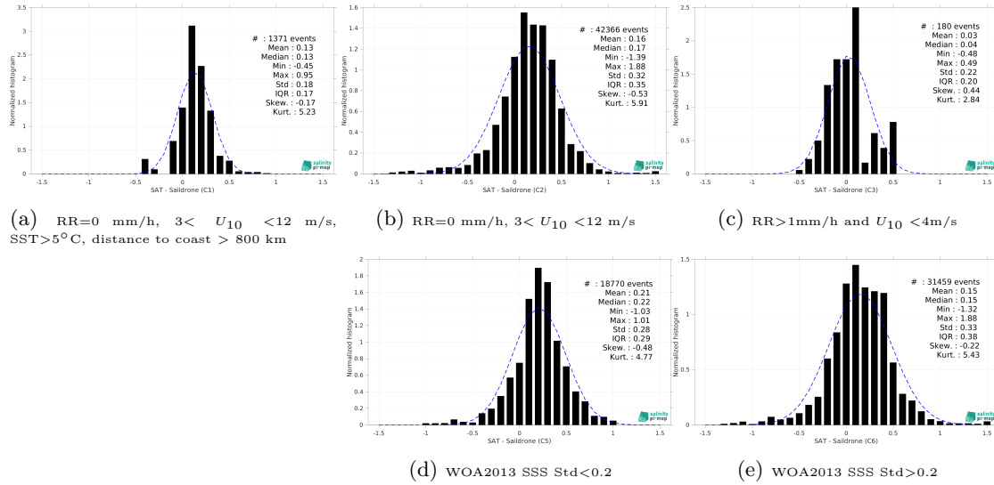
Figure 13: Normalized histogram of \Delta SSS (SMAP SSS L3 v5.0 - 8-Day running (JPL) - Saildrone) for 5 different subdatasets corresponding to: RR=0 mm/h, 3 < U_{10} < 12 m/s, SST>5°C, distance to coast > 800 km (a), RR=0 mm/h, 3 < U_{10} < 12 m/s (b), RR>1mm/h and U_{10} < 4 m/s (c), WOA2013 SSS Std<0.2 (d), WOA2013 SSS Std>0.2 (e).
