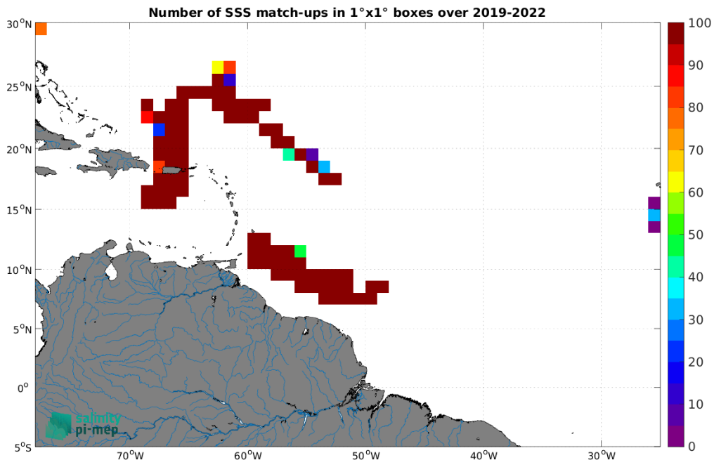
Figure 4: Number of SSS match-ups between Saildrone SSS and the SMAP SSS L3 v5.0 - 8-Day running (JPL) SSS product for the Amazon and Orinoco river plumes Pi-MEP region over 1^\circ \times 1^\circ boxes and for the full satellite product period.
