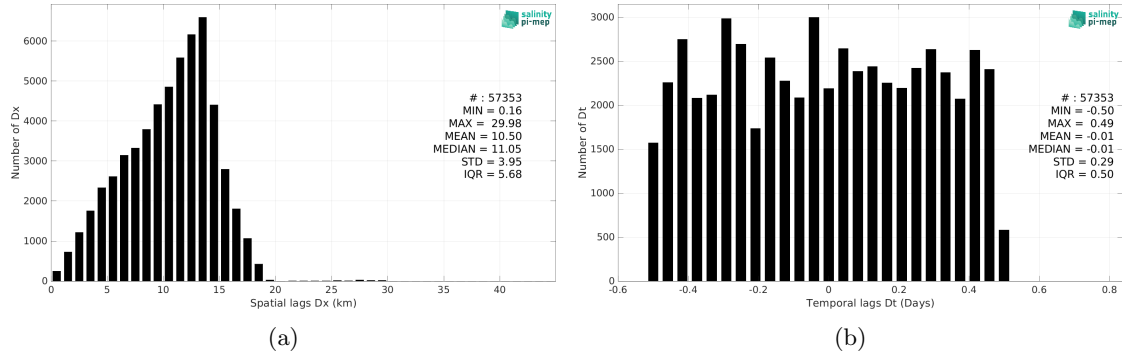
Figure 5: Histograms of the spatial (a) and temporal (b) lags between the location/time of the Saildrone measurement and the date of the corresponding SMAP SSS L3 v5.0 - 8-Day running (JPL) SSS pixel.
