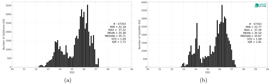
Figure 2: Histograms of SSS from Saildrone (a) and SMAP SSS L3 v5.0 - 8-Day running (JPL) (b) considering all match-up pairs per bins of 0.1 over the Amazon and Orinoco river plumes Pi-MEP region and for the full satellite product period.
