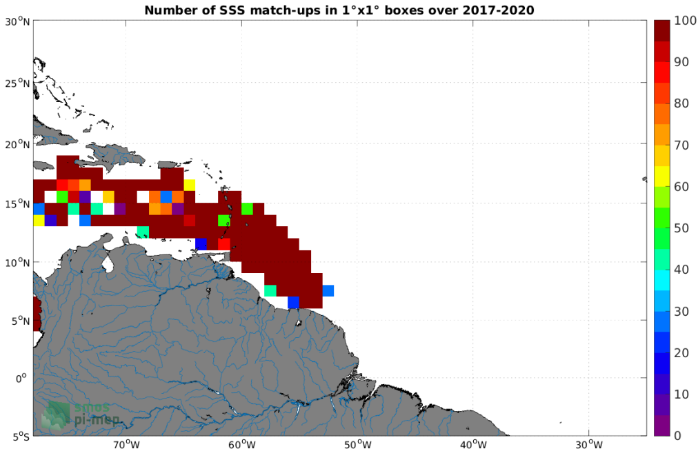
Figure 3: Number of SSS match-ups between Surface drifters SSS and the SMAP SSS L3 v5.0 - 8-Day running (JPL) SSS product for the Amazon and Orinoco river plumes Pi-MEP region over 1^\circ \times 1^\circ boxes and for the full satellite product period.
