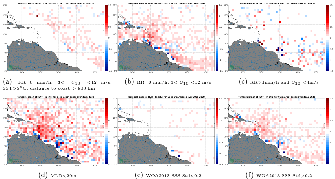
Figure 12: Temporal mean gridded over spatial boxes of size 1°x1° of \Delta SSS (SMAP SSS L3 v5.0 - 8-Day running (JPL) - Argo) for 6 different subdatasets corresponding to:RR=0 mm/h, 3 < U_{10} < 12 m/s, SST>5°C, distance to coast > 800 km (a), RR=0 mm/h, 3 < U_{10} < 12 m/s (b), RR>1mm/h and U_{10} < 4 m/s (c),MLD<20m (d),WOA2013 SSS Std<0.2 (e),WOA2013 SSS Std>0.2 (f).
