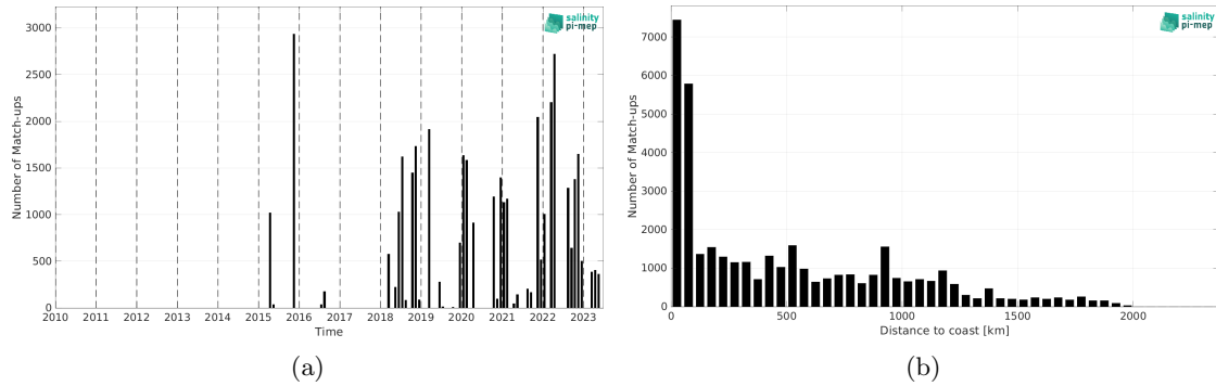
Figure 2: Number of match-ups between TSG (SAMOS) and SMAP SSS L3 v5.0 - Monthly (JPL) SSS as a function of time (a) and as function of the distance to coast (b) over the Amazon and Orinoco river plumes Pi-MEP region and for the full satellite product period.
