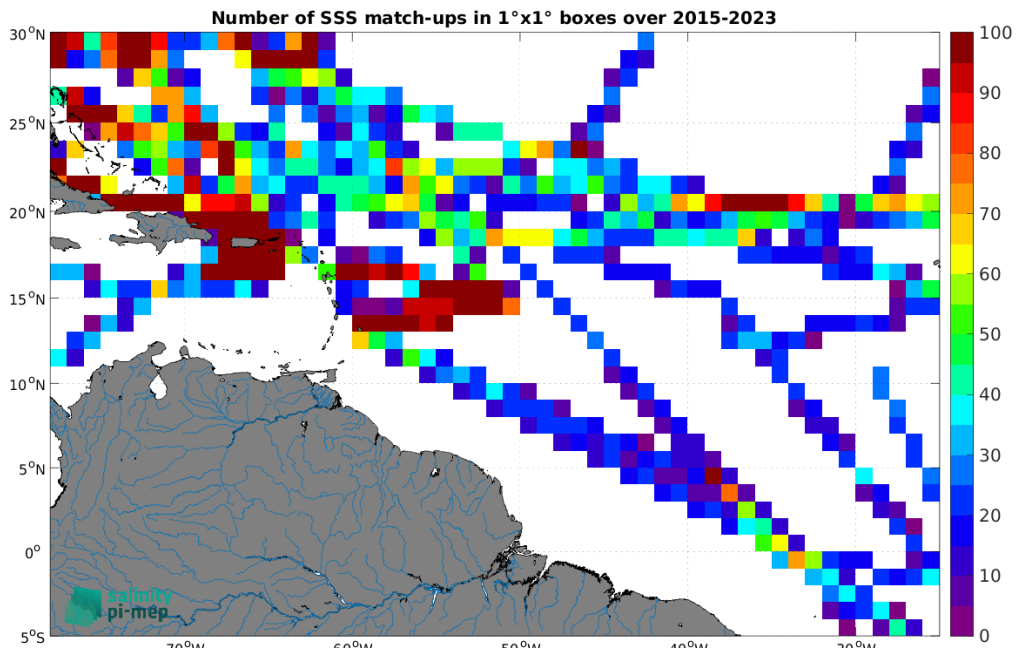
Figure 5: Number of SSS match-ups between TSG (SAMOS) SSS and the SMAP SSS L3 v5.0 - Monthly (JPL) SSS product for the Amazon and Orinoco river plumes Pi-MEP region over 1^\circ \times 1^\circ boxes and for the full satellite product period.
