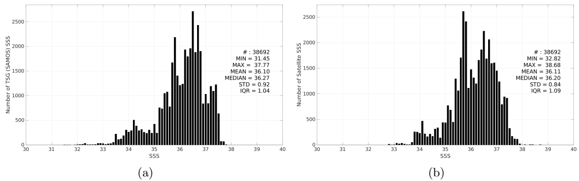
Figure 3: Histograms of SSS from TSG (SAMOS) (a) and SMAP SSS L3 v5.0 - Monthly (JPL) (b) considering all match-up pairs per bins of 0.1 over the Amazon and Orinoco river plumes Pi-MEP region and for the full satellite product period.
