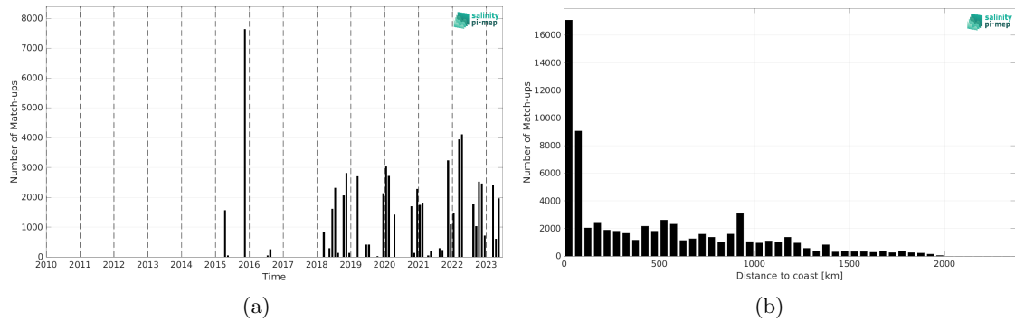
Figure 1: Number of match-ups between TSG (SAMOS) and SMAP SSS L3 v5.0 - Monthly (JPL) SSS as a function of time (a) and as function of the distance to coast (b) over the Amazon and Orinoco river plumes Pi-MEP region and for the full satellite product period.
