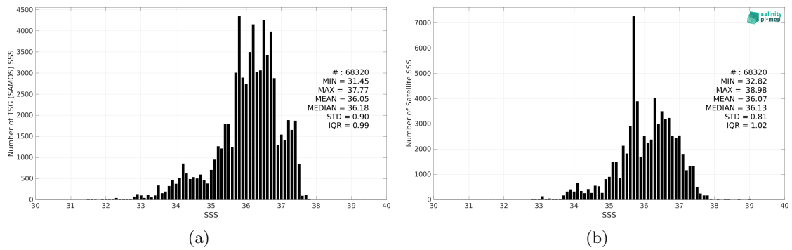
Figure 2: Histograms of SSS from TSG (SAMOS) (a) and SMAP SSS L3 v5.0 - Monthly (JPL) (b) considering all match-up pairs per bins of 0.1 over the Amazon and Orinoco river plumes Pi-MEP region and for the full satellite product period.
