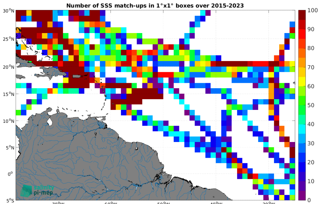
Figure 4: Number of SSS match-ups between TSG (SAMOS) SSS and the SMAP SSS L3 v5.0 - Monthly (JPL) SSS product for the Amazon and Orinoco river plumes Pi-MEP region over 1^\circ \times 1^\circ boxes and for the full satellite product period.
