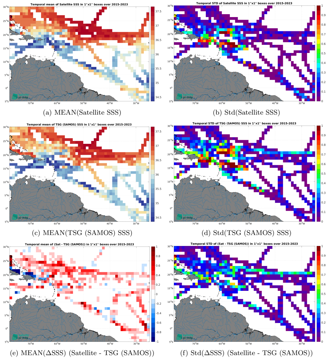
Figure 6: Temporal mean (left) and Std (right) of SSS from SMAP SSS L3 v5.0 - Monthly (JPL) (top), TSG (SAMOS) (middle), and of \Delta SSS (Satellite - TSG (SAMOS)). Only match-up pairs are used to generate these maps.
