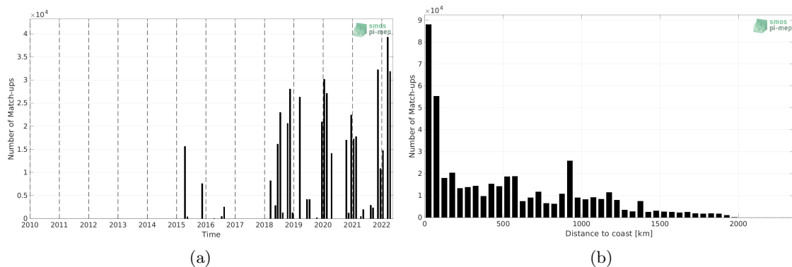
Figure 1: Number of match-ups between TSG (SAMOS) and SMAP SSS L3 v5.0 - Monthly (JPL) SSS as a function of time (a) and as function of the distance to coast (b) over the Amazon and Orinoco river plumes Pi-MEP region and for the full satellite product period.
