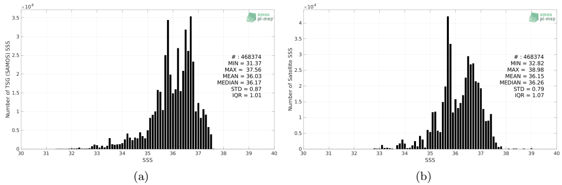
Figure 2: Histograms of SSS from TSG (SAMOS) (a) and SMAP SSS L3 v5.0 - Monthly (JPL) (b) considering all match-up pairs per bins of 0.1 over the Amazon and Orinoco river plumes Pi-MEP region and for the full satellite product period.
