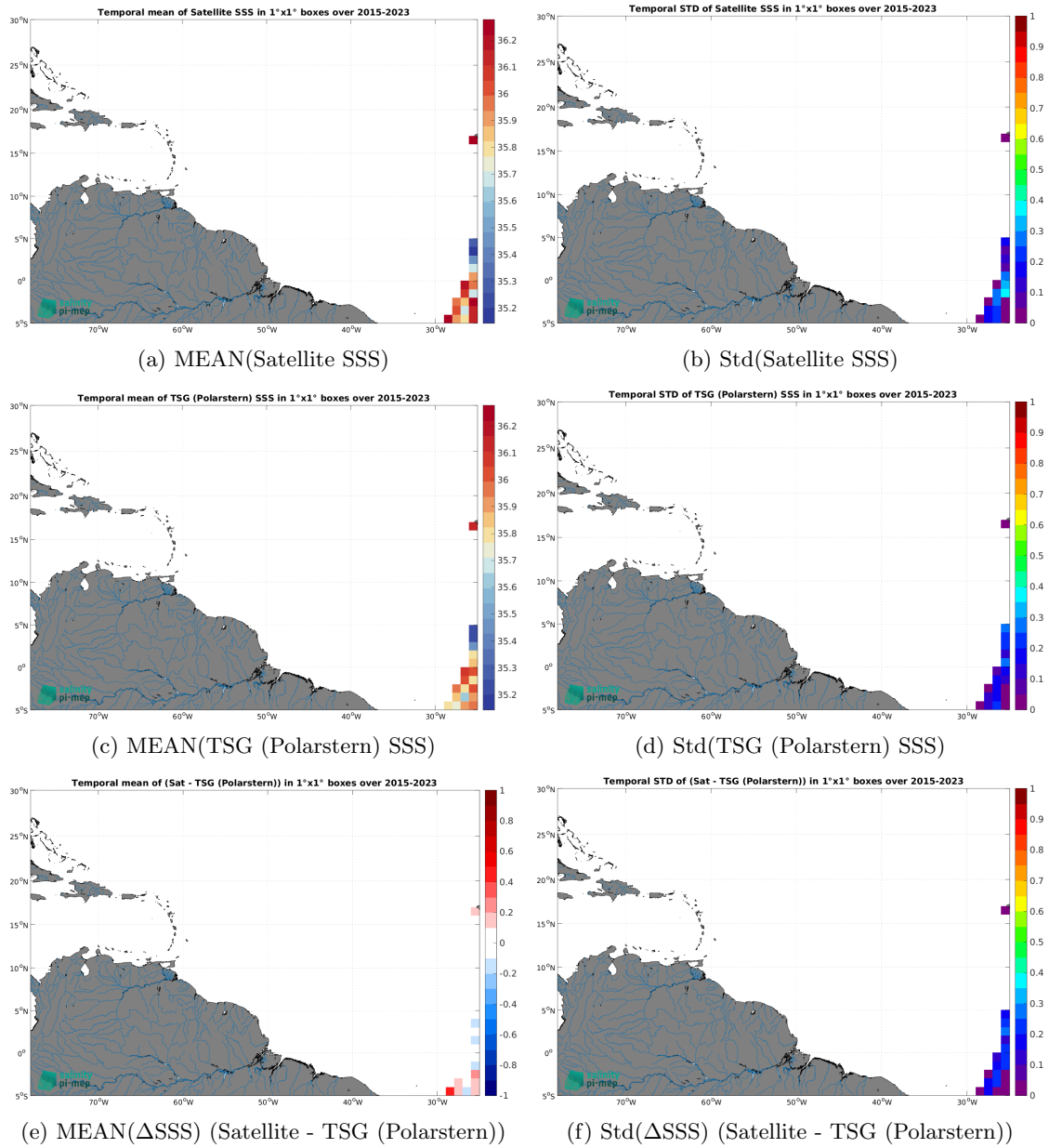
Figure 7: Temporal mean (left) and Std (right) of SSS from SMAP SSS L3 v5.0 - Monthly (JPL) (top), TSG (Polarstern) (middle), and of \Delta SSS (Satellite - TSG (Polarstern)). Only match-up pairs are used to generate these maps.
