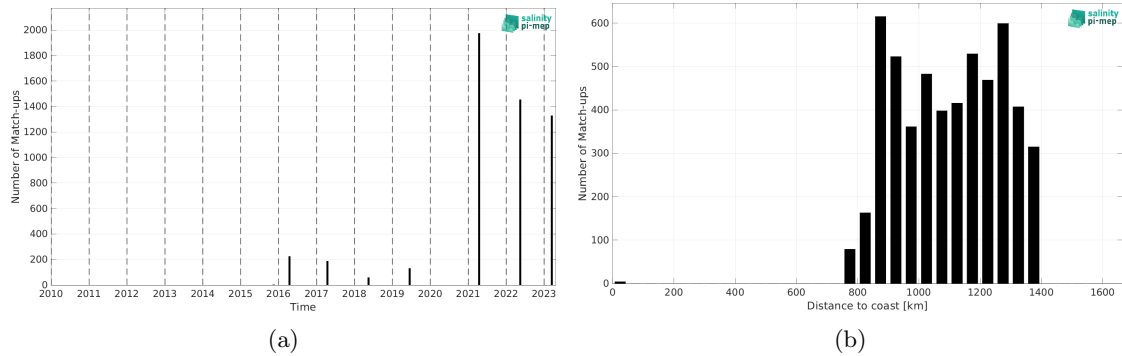
Figure 2: Number of match-ups between TSG (Polarstern) and SMAP SSS L3 v5.0 - Monthly (JPL) SSS as a function of time (a) and as function of the distance to coast (b) over the Amazon and Orinoco river plumes Pi-MEP region and for the full satellite product period.
