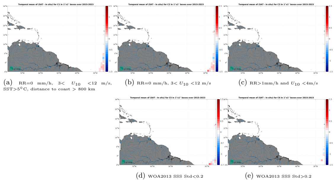
Figure 14: Temporal mean gridded over spatial boxes of size 1^\circ \times 1^\circ of \Delta SSS (SMAP SSS L3 v5.0 - Monthly (JPL) - TSG (Polarstern)) for 5 different subdatasets corresponding to:RR=0 mm/h, 3 < U_{10} < 12 m/s, SST > 5^\circ\text{C} , distance to coast > 800 km (a), RR=0 mm/h, 3 < U_{10} < 12 m/s (b), RR > 1 mm/h and U_{10} < 4 m/s (c), WOA2013 SSS Std < 0.2 (d), WOA2013 SSS Std > 0.2 (e).
