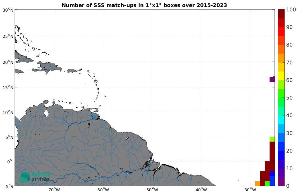
Figure 5: Number of SSS match-ups between TSG (Polarstern) SSS and the SMAP SSS L3 v5.0 - Monthly (JPL) SSS product for the Amazon and Orinoco river plumes Pi-MEP region over 1^\circ \times 1^\circ boxes and for the full satellite product period.
