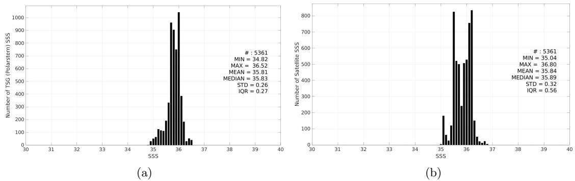
Figure 3: Histograms of SSS from TSG (Polarstern) (a) and SMAP SSS L3 v5.0 - Monthly (JPL) (b) considering all match-up pairs per bins of 0.1 over the Amazon and Orinoco river plumes Pi-MEP region and for the full satellite product period.
