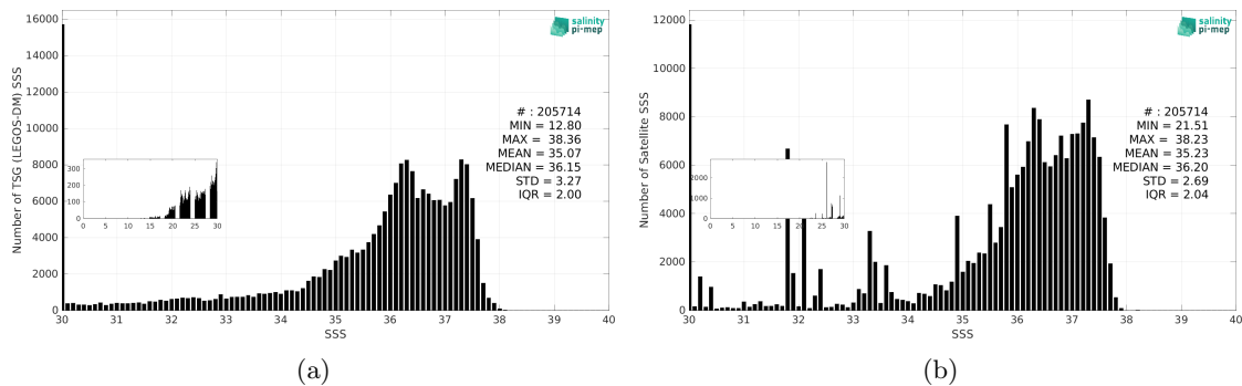
Figure 3: Histograms of SSS from TSG (LEGOS-DM) (a) and SMAP SSS L3 v5.0 - Monthly (JPL) (b) considering all match-up pairs per bins of 0.1 over the Amazon and Orinoco river plumes Pi-MEP region and for the full satellite product period.
