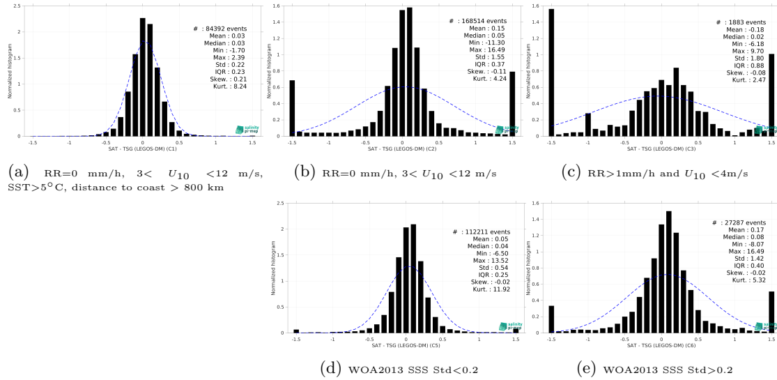
Figure 15: Normalized histogram of \Delta\text{SSS} (SMAP SSS L3 v5.0 - Monthly (JPL) - TSG (LEGOS-DM)) for 5 different subdatasets corresponding to: RR=0 mm/h, 3 < U_{10} < 12 m/s, SST>5°C, distance to coast > 800 km (a), RR=0 mm/h, 3 < U_{10} < 12 m/s (b), RR>1mm/h and U_{10} < 4 m/s (c), WOA2013 SSS Std<0.2 (d), WOA2013 SSS Std>0.2 (e).
