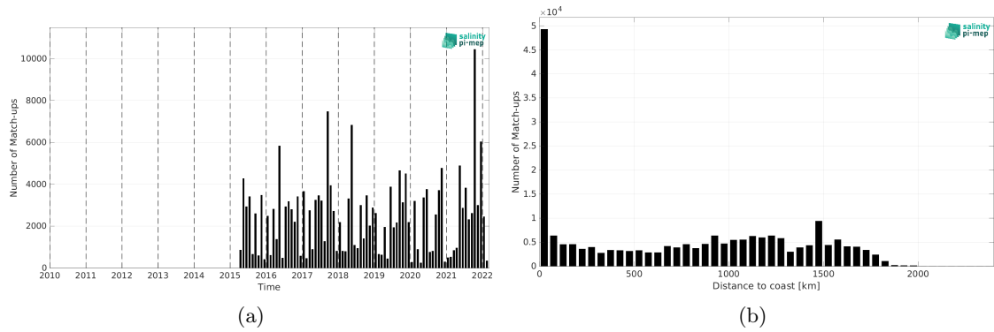
Figure 2: Number of match-ups between TSG (LEGOS-DM) and SMAP SSS L3 v5.0 - Monthly (JPL) SSS as a function of time (a) and as function of the distance to coast (b) over the Amazon and Orinoco river plumes Pi-MEP region and for the full satellite product period.
