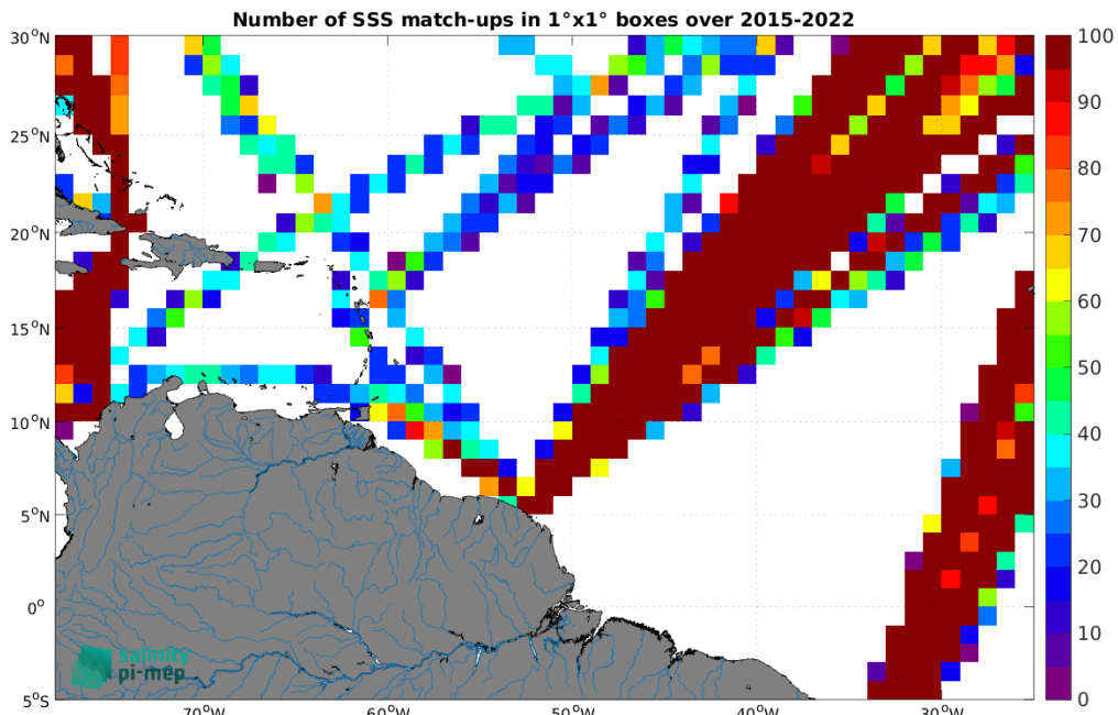
Figure 5: Number of SSS match-ups between TSG (LEGOS-DM) SSS and the SMAP SSS L3 v5.0 - Monthly (JPL) SSS product for the Amazon and Orinoco river plumes Pi-MEP region over 1^\circ \times 1^\circ boxes and for the full satellite product period.
