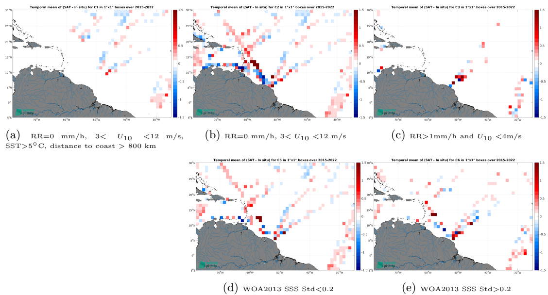
Figure 14: Temporal mean gridded over spatial boxes of size 1^\circ \times 1^\circ of \Delta SSS (SMAP SSS L3 v5.0 - Monthly (JPL) - TSG (LEGOS-DM)) for 5 different subdatasets corresponding to:RR=0 mm/h, 3 < U_{10} < 12 m/s, SST >5^\circ\text{C} , distance to coast > 800 km (a), RR=0 mm/h, 3 < U_{10} < 12 m/s (b), RR >1 mm/h and U_{10} < 4 m/s (c), WOA2013 SSS Std <0.2 (d), WOA2013 SSS Std >0.2 (e).
