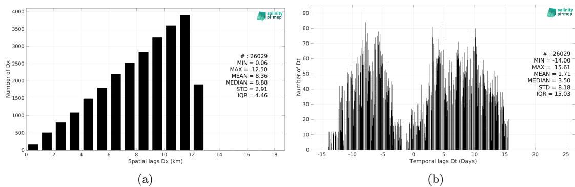
Figure 6: Histograms of the spatial (a) and temporal (b) lags between the location/time of the TSG (GOSUD-Sailing-ship) measurement and the date of the corresponding SMAP SSS L3 v5.0 - Monthly (JPL) SSS pixel.
