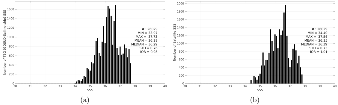
Figure 3: Histograms of SSS from TSG (GOSUD-Sailing-ship) (a) and SMAP SSS L3 v5.0 - Monthly (JPL) (b) considering all match-up pairs per bins of 0.1 over the Amazon and Orinoco river plumes Pi-MEP region and for the full satellite product period.
