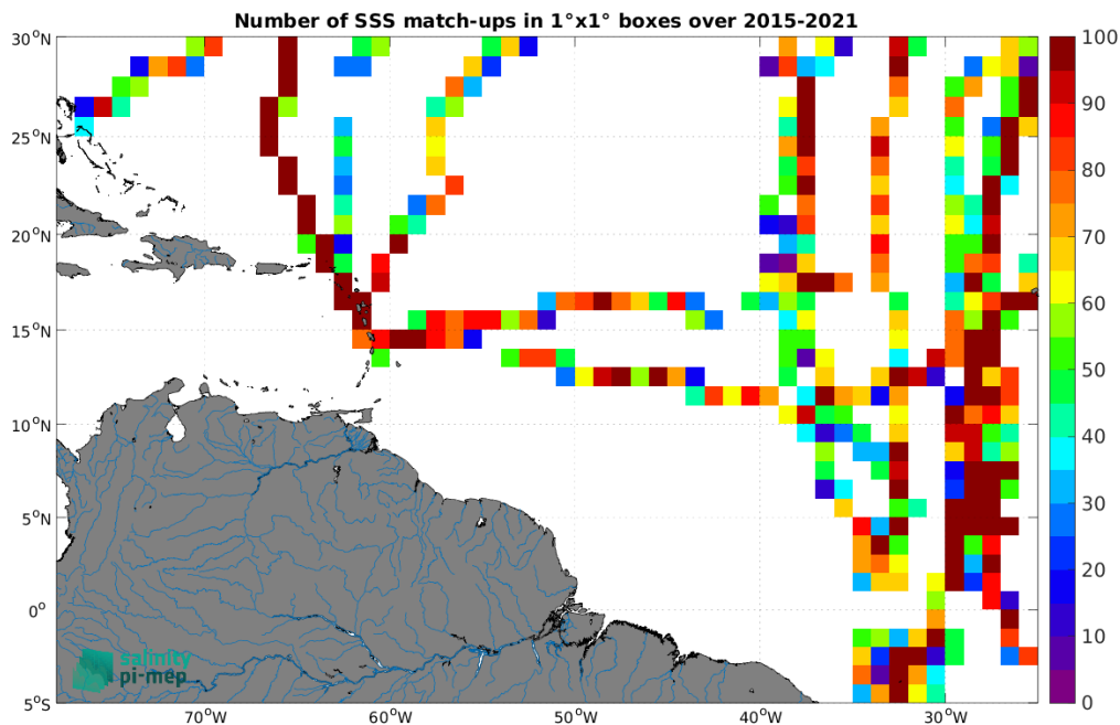
Figure 5: Number of SSS match-ups between TSG (GOSUD-Sailing-ship) SSS and the SMAP SSS L3 v5.0 - Monthly (JPL) SSS product for the Amazon and Orinoco river plumes Pi-MEP region over 1^\circ \times 1^\circ boxes and for the full satellite product period.
