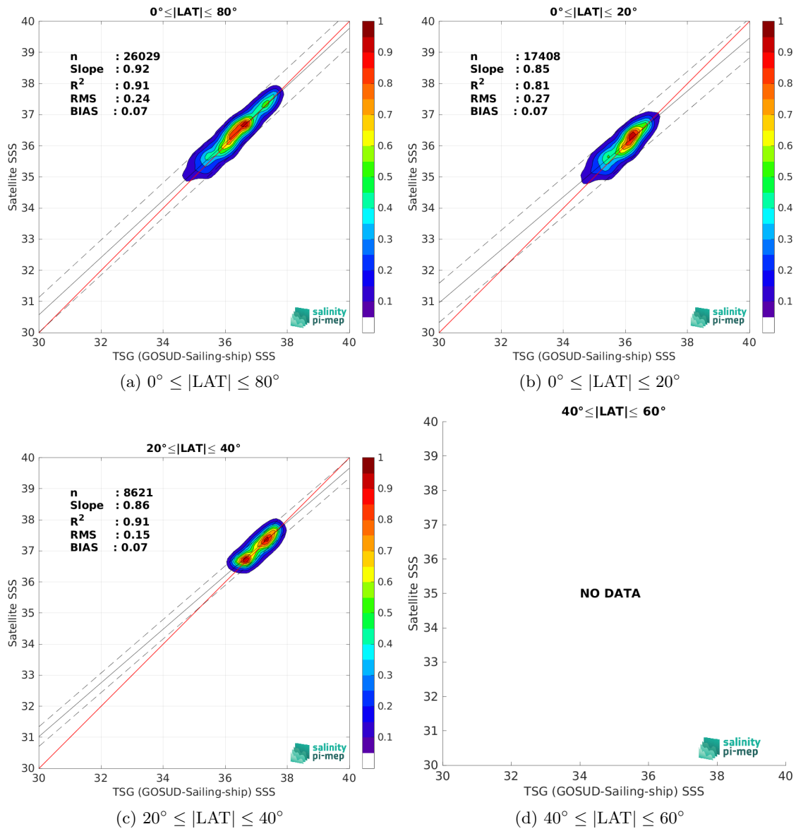
Figure 10: Contour maps of the concentration of SMAP SSS L3 v5.0 - Monthly (JPL) SSS (y-axis) versus TSG (GOSUD-Sailing-ship) SSS (x-axis) at match-up pairs for different latitude bands. For each plot, the red line shows x=y . The black thin and dashed lines indicate a linear fit through the data cloud and the \pm 95\% confidence levels, respectively. The number match-up pairs n , the slope and R^2 coefficient of the linear fit, the root mean square (RMS) and the mean bias between satellite and in situ data are indicated for each latitude band in each plots.
