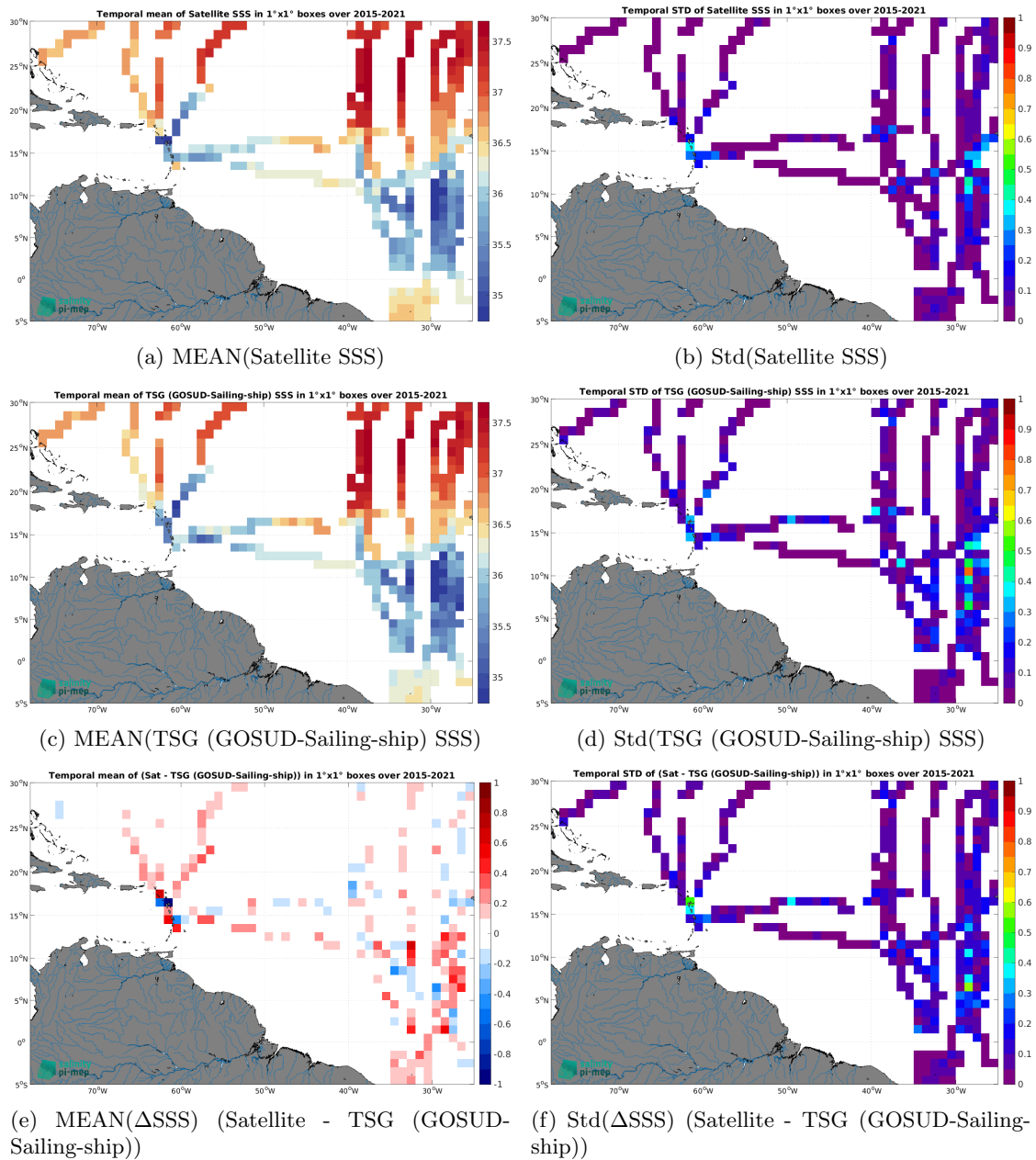
Figure 7: Temporal mean (left) and Std (right) of SSS from SMAP SSS L3 v5.0 - Monthly (JPL) (top), TSG (GOSUD-Sailing-ship) (middle), and of \Delta SSS (Satellite - TSG (GOSUD-Sailing-ship)). Only match-up pairs are used to generate these maps.
