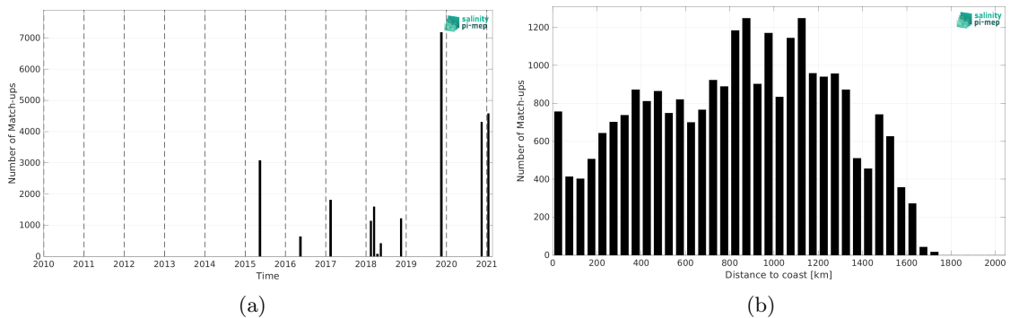
Figure 2: Number of match-ups between TSG (GOSUD-Sailing-ship) and SMAP SSS L3 v5.0 - Monthly (JPL) SSS as a function of time (a) and as function of the distance to coast (b) over the Amazon and Orinoco river plumes Pi-MEP region and for the full satellite product period.
