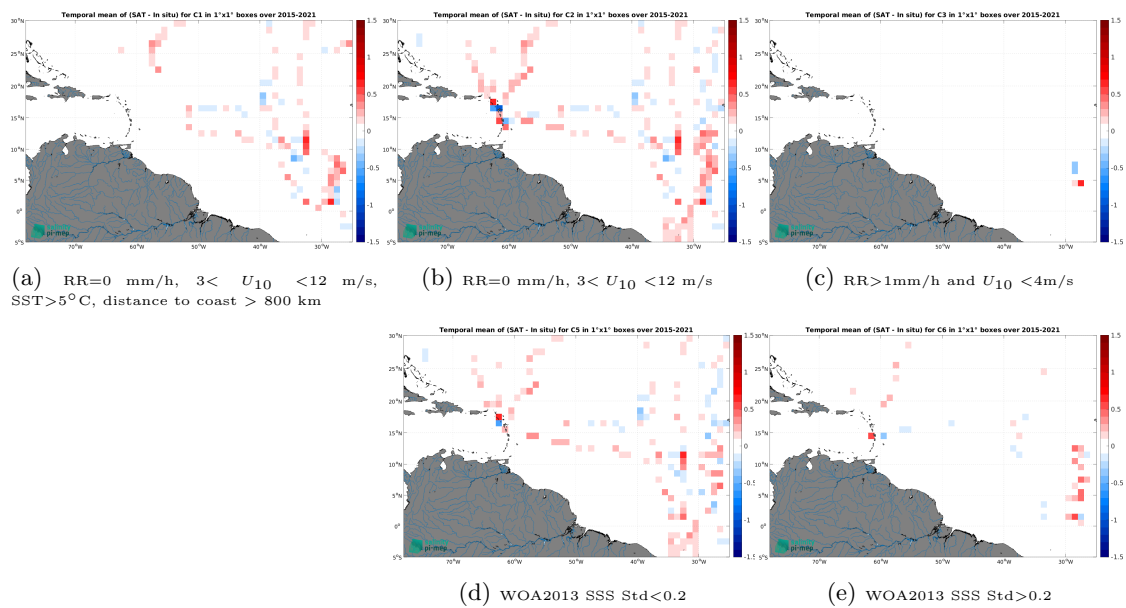
Figure 14: Temporal mean gridded over spatial boxes of size 1^\circ \times 1^\circ of \Delta SSS (SMAP SSS L3 v5.0 - Monthly (JPL) - TSG (GOSUD-Sailing-ship)) for 5 different subdatasets corresponding to:RR=0 mm/h, 3 < U_{10} < 12 m/s, SST >5^\circ C, distance to coast > 800 km (a), RR=0 mm/h, 3 < U_{10} < 12 m/s (b), RR >1 mm/h and U_{10} < 4 m/s (c), WOA2013 SSS Std <0.2 (d), WOA2013 SSS Std >0.2 (e).
