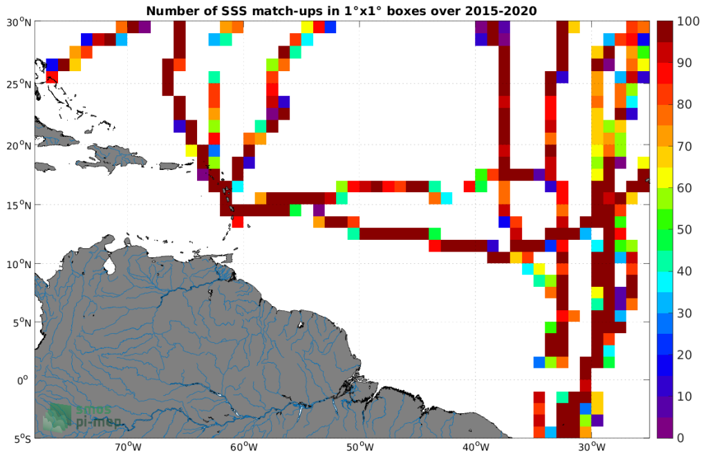
Figure 4: Number of SSS match-ups between TSG (GOSUD-Sailing-ship) SSS and the SMAP SSS L3 v5.0 - Monthly (JPL) SSS product for the Amazon and Orinoco river plumes Pi-MEP region over 1^\circ \times 1^\circ boxes and for the full satellite product period.
