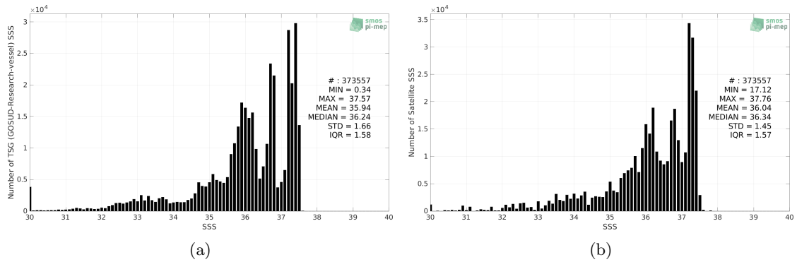
Figure 2: Histograms of SSS from TSG (GOSUD-Research-vessel) (a) and SMAP SSS L3 v5.0 - Monthly (JPL) (b) considering all match-up pairs per bins of 0.1 over the Amazon and Orinoco river plumes Pi-MEP region and for the full satellite product period.
