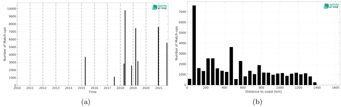
Figure 2: Number of match-ups between TSG (CSIC-UTM) and SMAP SSS L3 v5.0 - Monthly (JPL) SSS as a function of time (a) and as function of the distance to coast (b) over the Amazon and Orinoco river plumes Pi-MEP region and for the full satellite product period.
