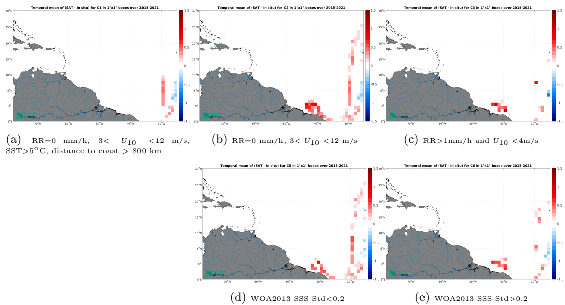
Figure 14: Temporal mean gridded over spatial boxes of size 1^\circ \times 1^\circ of \Delta SSS (SMAP SSS L3 v5.0 - Monthly (JPL) - TSG (CSIC-UTM)) for 5 different subdatasets corresponding to:RR=0 mm/h, 3 < U_{10} < 12 m/s, SST >5^\circ\text{C} , distance to coast > 800 km (a), RR=0 mm/h, 3 < U_{10} < 12 m/s (b), RR >1 mm/h and U_{10} < 4 m/s (c), WOA2013 SSS Std <0.2 (d), WOA2013 SSS Std >0.2 (e).
