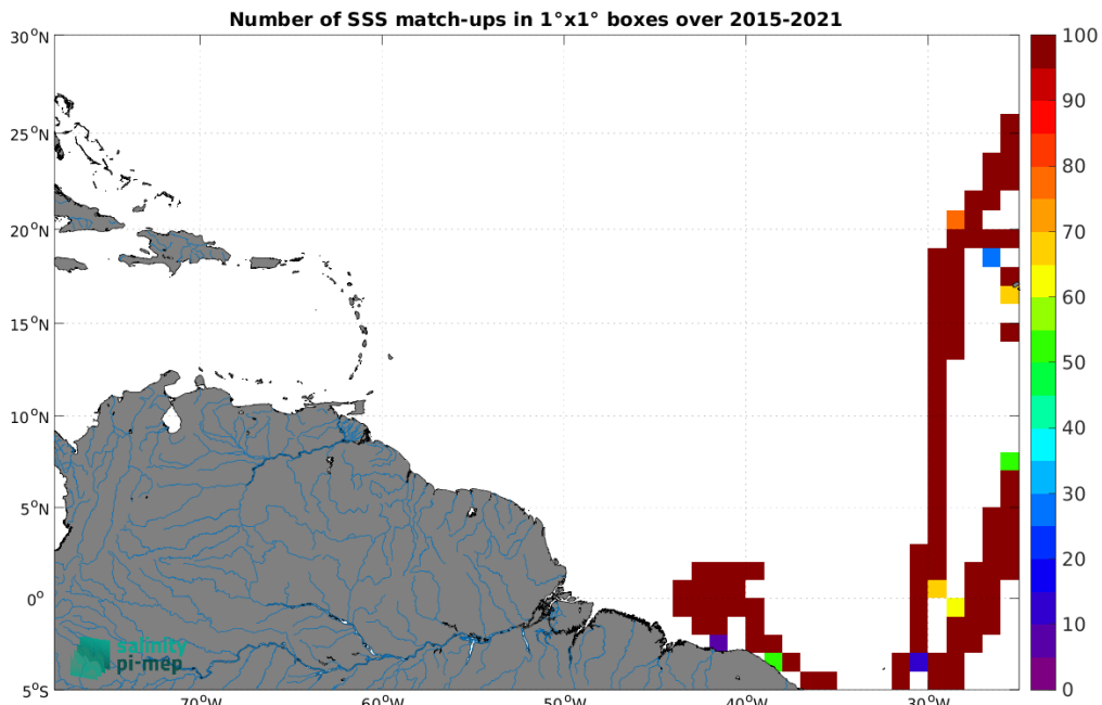
Figure 5: Number of SSS match-ups between TSG (CSIC-UTM) SSS and the SMAP SSS L3 v5.0 - Monthly (JPL) SSS product for the Amazon and Orinoco river plumes Pi-MEP region over 1^\circ \times 1^\circ boxes and for the full satellite product period.
