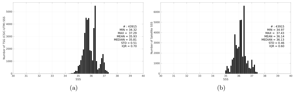
Figure 3: Histograms of SSS from TSG (CSIC-UTM) (a) and SMAP SSS L3 v5.0 - Monthly (JPL) (b) considering all match-up pairs per bins of 0.1 over the Amazon and Orinoco river plumes Pi-MEP region and for the full satellite product period.
