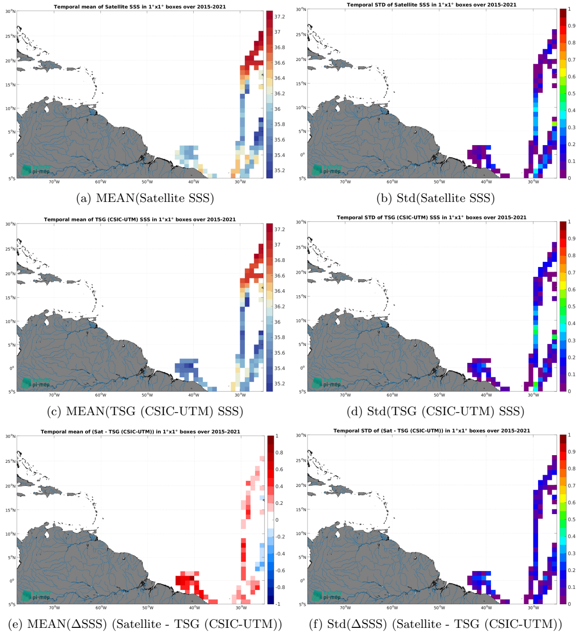
Figure 7: Temporal mean (left) and Std (right) of SSS from SMAP SSS L3 v5.0 - Monthly (JPL) (top), TSG (CSIC-UTM) (middle), and of \Delta SSS (Satellite - TSG (CSIC-UTM)). Only match-up pairs are used to generate these maps.
