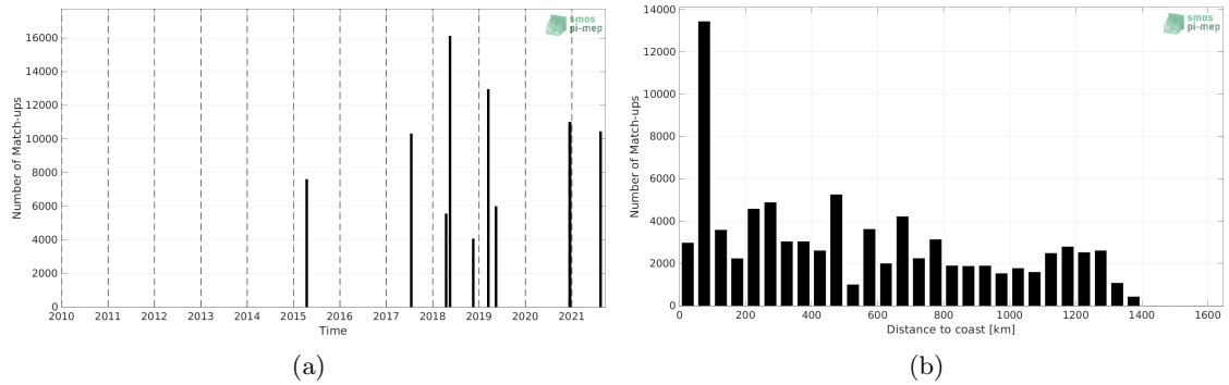
Figure 1: Number of match-ups between TSG (CSIC-UTM) and SMAP SSS L3 v5.0 - Monthly (JPL) SSS as a function of time (a) and as function of the distance to coast (b) over the Amazon and Orinoco river plumes Pi-MEP region and for the full satellite product period.
