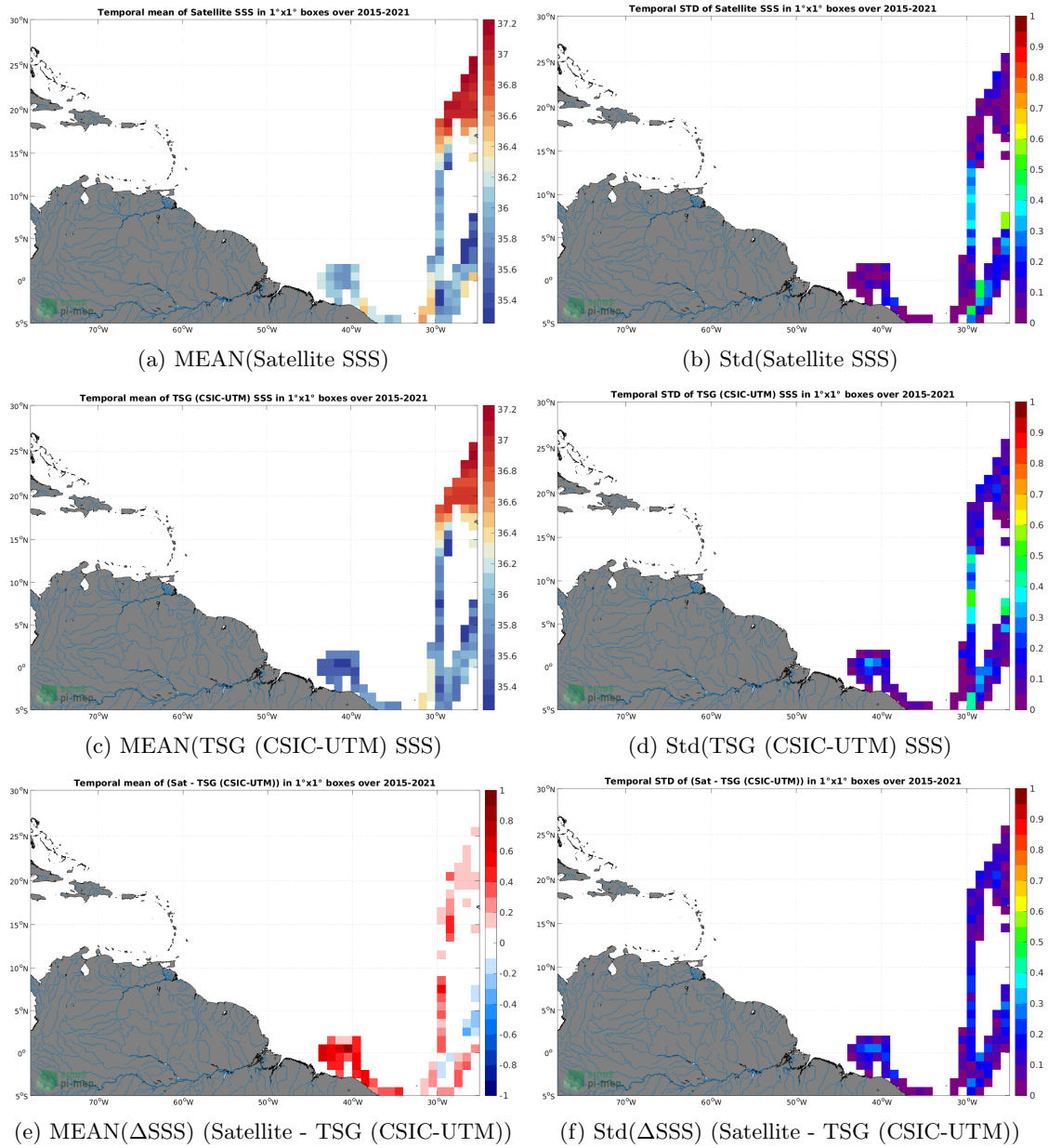
Figure 6: Temporal mean (left) and Std (right) of SSS from SMAP SSS L3 v5.0 - Monthly (JPL) (top), TSG (CSIC-UTM) (middle), and of \Delta SSS (Satellite - TSG (CSIC-UTM)). Only match-up pairs are used to generate these maps.
