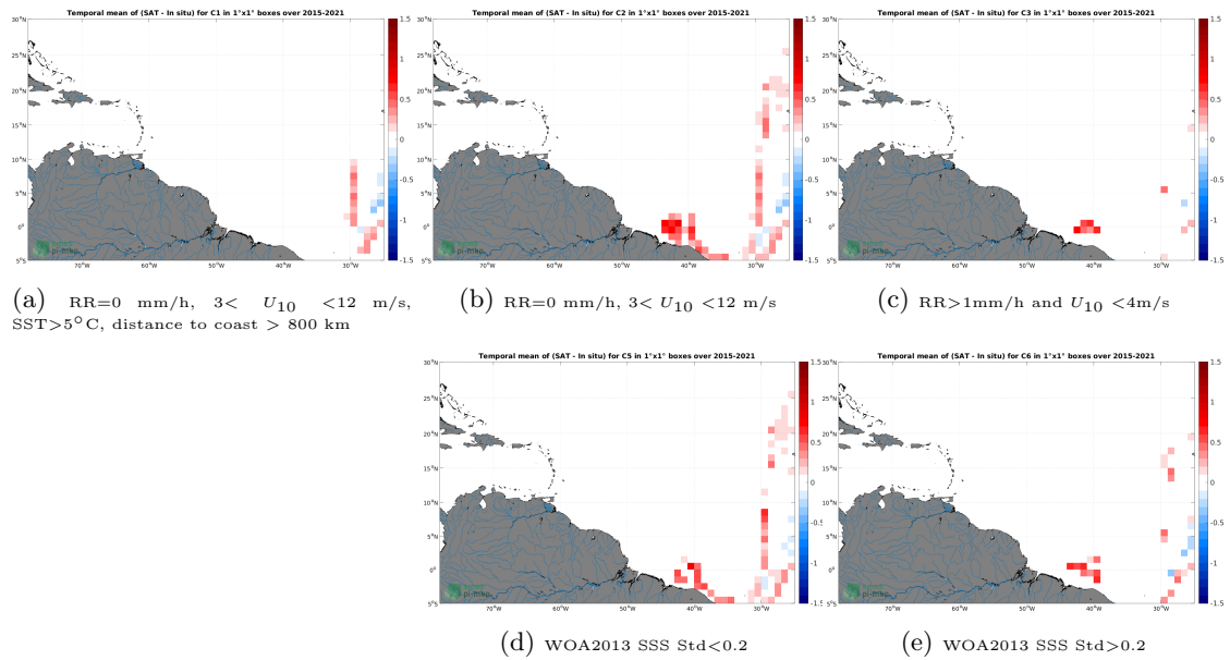
Figure 12: Temporal mean gridded over spatial boxes of size 1^\circ \times 1^\circ of \Delta SSS (SMAP SSS L3 v5.0 - Monthly (JPL) - TSG (CSIC-UTM)) for 5 different subdatasets corresponding to:RR=0 mm/h, 3 < U_{10} < 12 m/s, SST >5^\circ\text{C} , distance to coast > 800 km (a), RR=0 mm/h, 3 < U_{10} < 12 m/s (b), RR >1 mm/h and U_{10} < 4 m/s (c), WOA2013 SSS Std <0.2 (d), WOA2013 SSS Std >0.2 (e).
