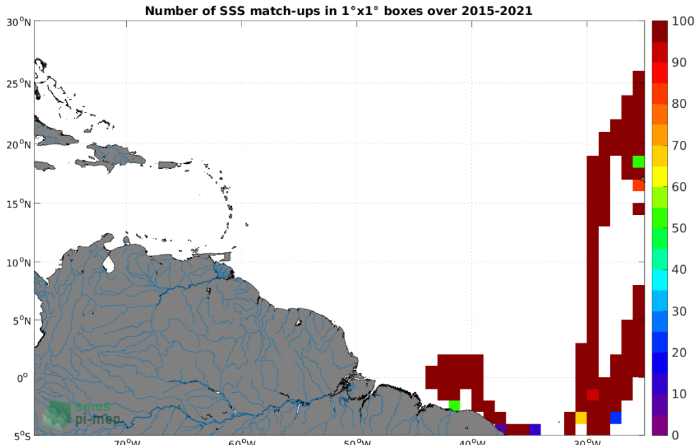
Figure 4: Number of SSS match-ups between TSG (CSIC-UTM) SSS and the SMAP SSS L3 v5.0 - Monthly (JPL) SSS product for the Amazon and Orinoco river plumes Pi-MEP region over 1^\circ \times 1^\circ boxes and for the full satellite product period.
