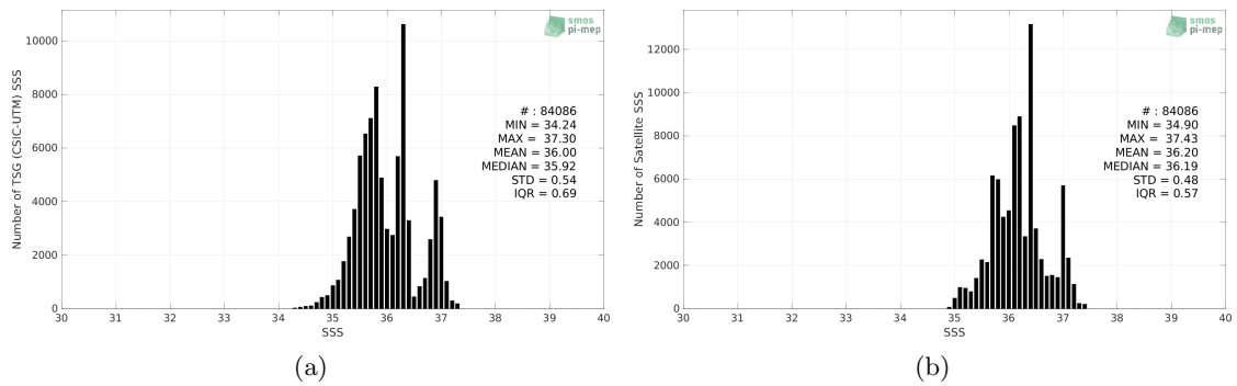
Figure 2: Histograms of SSS from TSG (CSIC-UTM) (a) and SMAP SSS L3 v5.0 - Monthly (JPL) (b) considering all match-up pairs per bins of 0.1 over the Amazon and Orinoco river plumes Pi-MEP region and for the full satellite product period.
