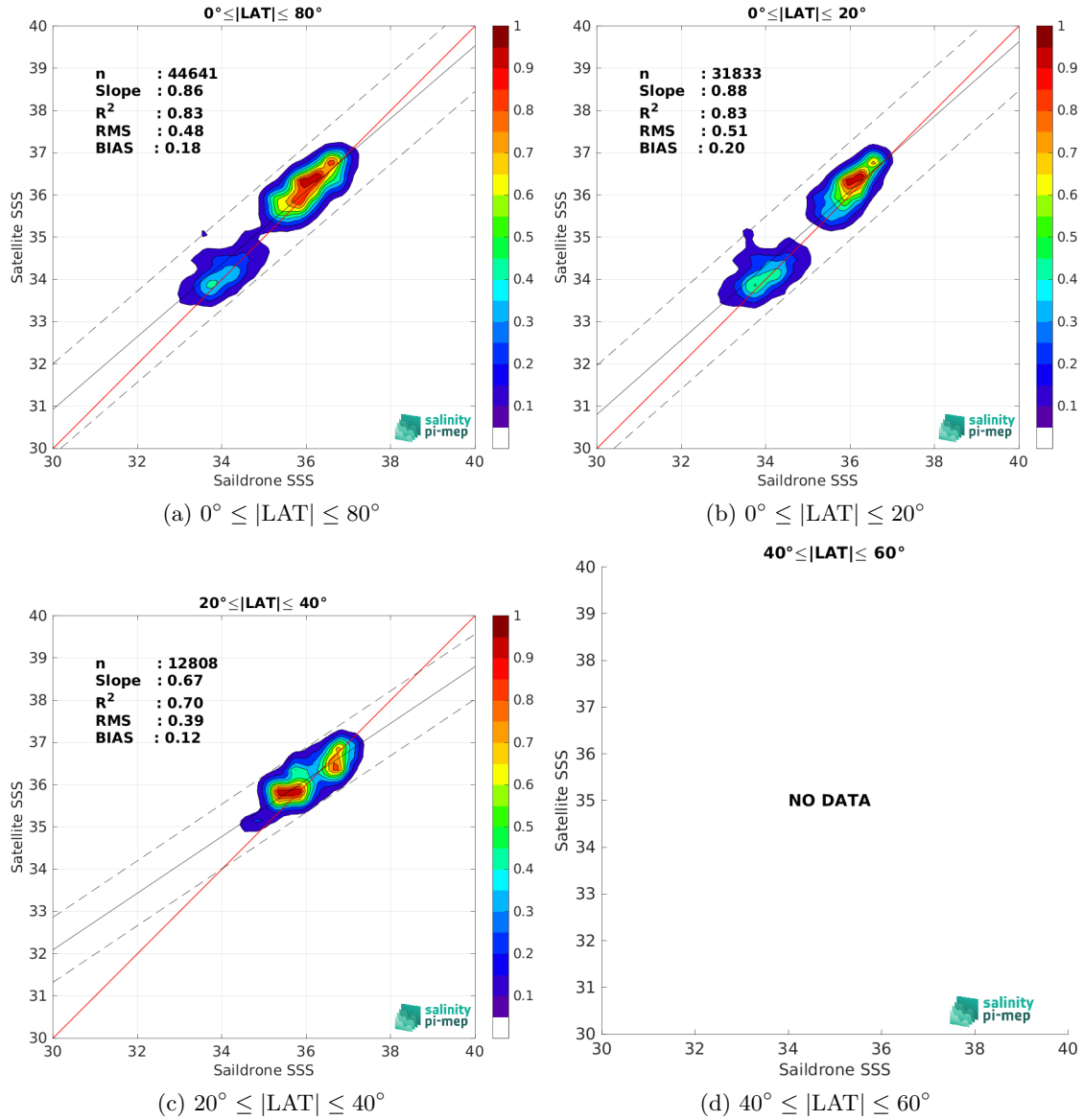
Figure 10: Contour maps of the concentration of SMAP SSS L3 v5.0 - Monthly (JPL) SSS (y-axis) versus Saildrone SSS (x-axis) at match-up pairs for different latitude bands. For each plot, the red line shows x=y . The black thin and dashed lines indicate a linear fit through the data cloud and the \pm 95\% confidence levels, respectively. The number match-up pairs n , the slope and R^2 coefficient of the linear fit, the root mean square (RMS) and the mean bias between satellite and in situ data are indicated for each latitude band in each plots.
