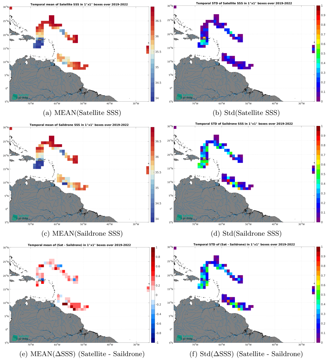
Figure 7: Temporal mean (left) and Std (right) of SSS from SMAP SSS L3 v5.0 - Monthly (JPL) (top), Saildrone (middle), and of \Delta SSS (Satellite - Saildrone). Only match-up pairs are used to generate these maps.
