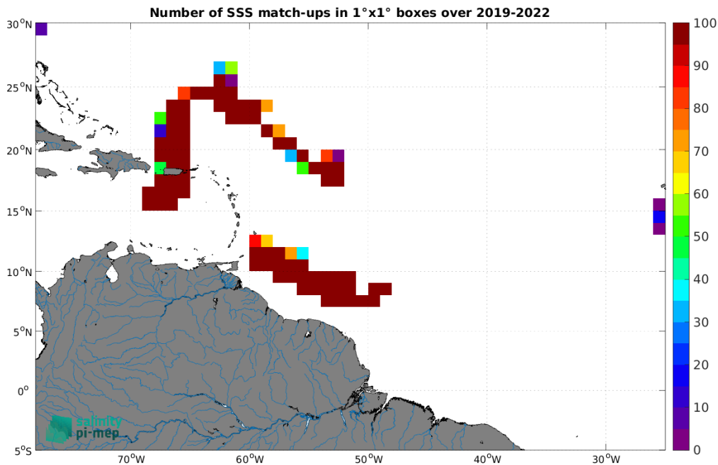
Figure 5: Number of SSS match-ups between Saildrone SSS and the SMAP SSS L3 v5.0 - Monthly (JPL) SSS product for the Amazon and Orinoco river plumes Pi-MEP region over 1^\circ \times 1^\circ boxes and for the full satellite product period.
