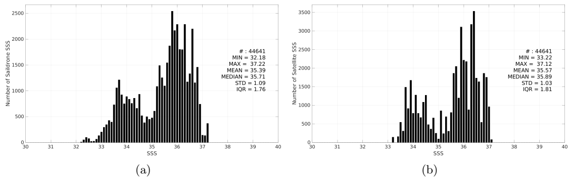
Figure 3: Histograms of SSS from Saildrone (a) and SMAP SSS L3 v5.0 - Monthly (JPL) (b) considering all match-up pairs per bins of 0.1 over the Amazon and Orinoco river plumes Pi-MEP region and for the full satellite product period.
