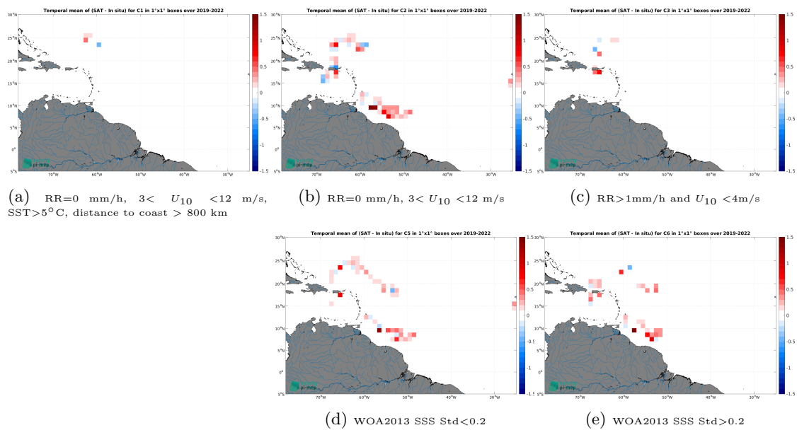
Figure 14: Temporal mean gridded over spatial boxes of size 1^\circ \times 1^\circ of \Delta SSS (SMAP SSS L3 v5.0 - Monthly (JPL) - Saildrone) for 5 different subdatasets corresponding to:RR=0 mm/h, 3 < U_{10} < 12 m/s, SST >5^\circ\text{C} , distance to coast > 800 km (a), RR=0 mm/h, 3 < U_{10} < 12 m/s (b), RR >1 mm/h and U_{10} < 4 m/s (c), WOA2013 SSS Std <0.2 (d), WOA2013 SSS Std >0.2 (e).
