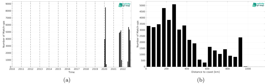
Figure 2: Number of match-ups between Saildrone and SMAP SSS L3 v5.0 - Monthly (JPL) SSS as a function of time (a) and as function of the distance to coast (b) over the Amazon and Orinoco river plumes Pi-MEP region and for the full satellite product period.
