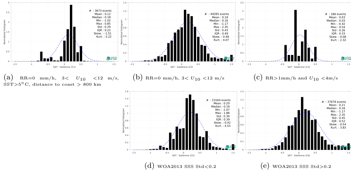
Figure 13: Normalized histogram of \Delta SSS (SMAP SSS L3 v5.0 - Monthly (JPL) - Saldrone) for 5 different subdatasets corresponding to: RR=0 mm/h, 3 < U_{10} < 12 m/s, SST>5°C, distance to coast > 800 km (a), RR=0 mm/h, 3 < U_{10} < 12 m/s (b), RR>1mm/h and U_{10} < 4 m/s (c), WOA2013 SSS Std<0.2 (d), WOA2013 SSS Std>0.2 (e).
