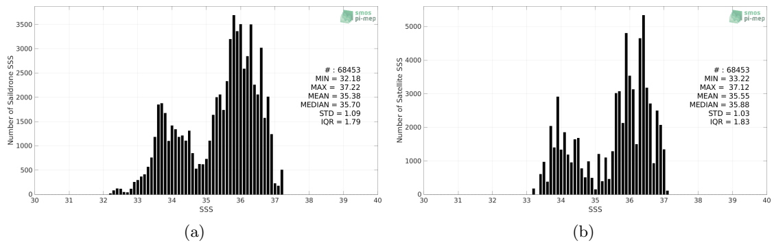
Figure 2: Histograms of SSS from Sairdron (a) and SMAP SSS L3 v5.0 - Monthly (JPL) (b) considering all match-up pairs per bins of 0.1 over the Amazon and Orinoco river plumes Pi-MEP region and for the full satellite product period.
