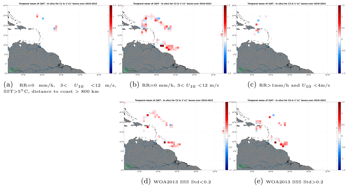
Figure 12: Temporal mean gridded over spatial boxes of size 1^\circ \times 1^\circ of \Delta SSS (SMAP SSS L3 v5.0 - Monthly (JPL) - Saildrone) for 5 different subdatasets corresponding to:RR=0 mm/h, 3 < U_{10} < 12 m/s, SST >5^\circ\text{C} , distance to coast > 800 km (a), RR=0 mm/h, 3 < U_{10} < 12 m/s (b), RR >1 mm/h and U_{10} < 4 m/s (c), WOA2013 SSS Std <0.2 (d), WOA2013 SSS Std >0.2 (e).
