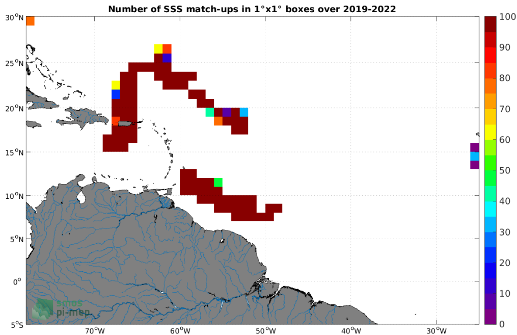
Figure 4: Number of SSS match-ups between Saildrone SSS and the SMAP SSS L3 v5.0 - Monthly (JPL) SSS product for the Amazon and Orinoco river plumes Pi-MEP region over 1^\circ \times 1^\circ boxes and for the full satellite product period.
