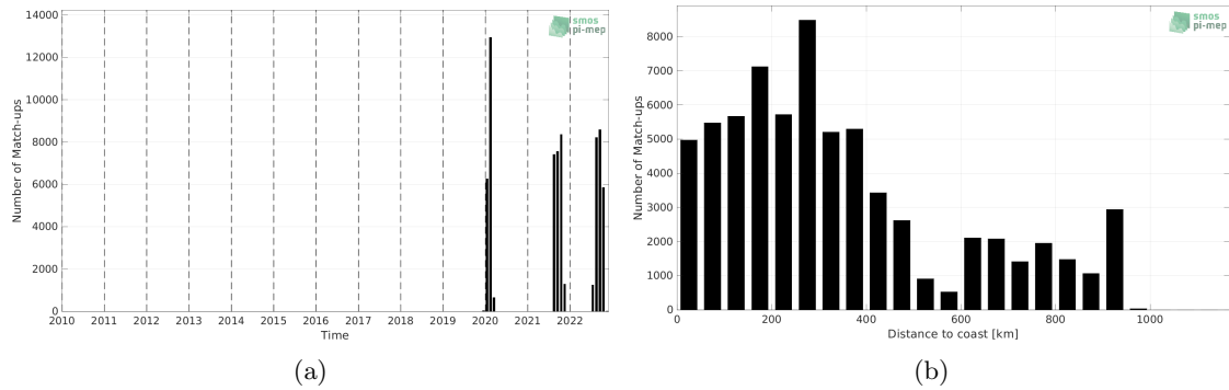
Figure 1: Number of match-ups between Sairdron and SMAP SSS L3 v5.0 - Monthly (JPL) SSS as a function of time (a) and as function of the distance to coast (b) over the Amazon and Orinoco river plumes Pi-MEP region and for the full satellite product period.
