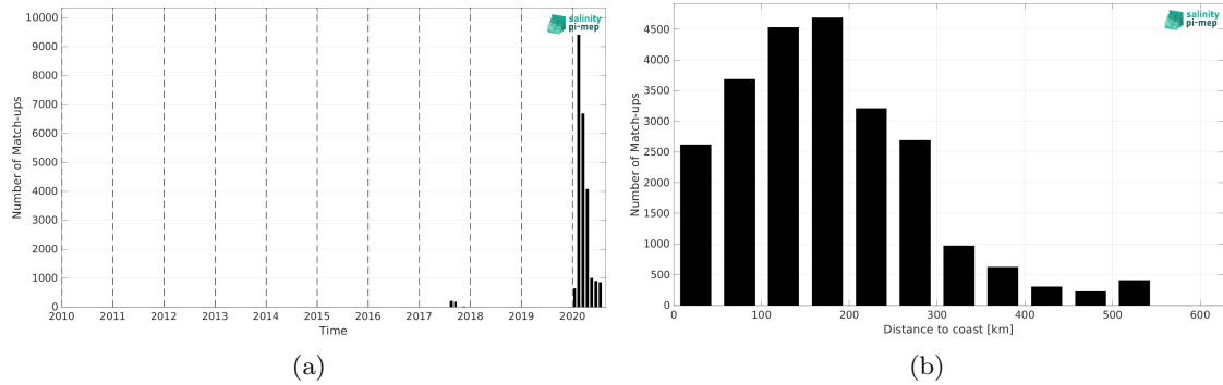
Figure 2: Number of match-ups between Surface drifters and SMAP SSS L3 v5.0 - Monthly (JPL) SSS as a function of time (a) and as function of the distance to coast (b) over the Amazon and Orinoco river plumes Pi-MEP region and for the full satellite product period.
