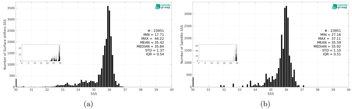
Figure 3: Histograms of SSS from Surface drifters (a) and SMAP SSS L3 v5.0 - Monthly (JPL) (b) considering all match-up pairs per bins of 0.1 over the Amazon and Orinoco river plumes Pi-MEP region and for the full satellite product period.
