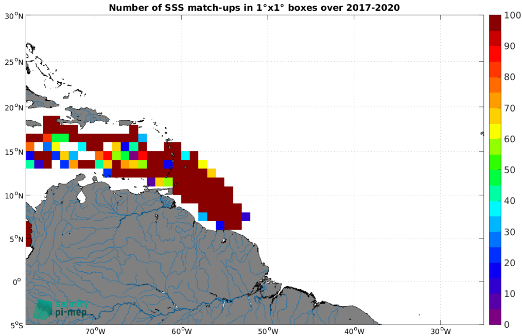
Figure 4: Number of SSS match-ups between Surface drifters SSS and the SMAP SSS L3 v5.0 - Monthly (JPL) SSS product for the Amazon and Orinoco river plumes Pi-MEP region over 1^\circ \times 1^\circ boxes and for the full satellite product period.
