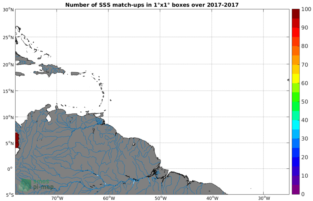
Figure 3: Number of SSS match-ups between Surface drifters SSS and the SMAP-L3-JPL-V4.3-MONTHLY-60KM SSS product for the Amazon and Orinoco river plumes Pi-MEP region over 1°x1° boxes and for the full satellite product period.
