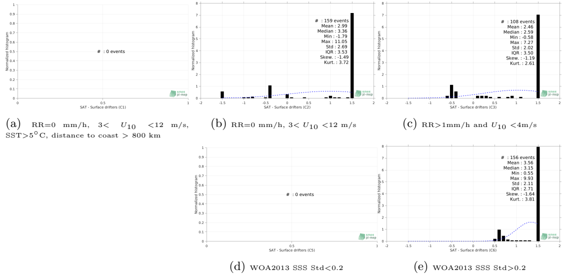
Figure 12: Normalized histogram of \Delta SSS (SMAP-L3-JPL-V4.3-MONTHLY-60KM - Surface drifters) for 5 different subdatasets corresponding to: RR=0 mm/h, 3 < U_{10} < 12 m/s, SST>5°C, distance to coast > 800 km (a), RR=0 mm/h, 3 < U_{10} < 12 m/s (b), RR>1mm/h and U_{10} < 4 m/s (c), WOA2013 SSS Std<0.2 (d), WOA2013 SSS Std>0.2 (e).
