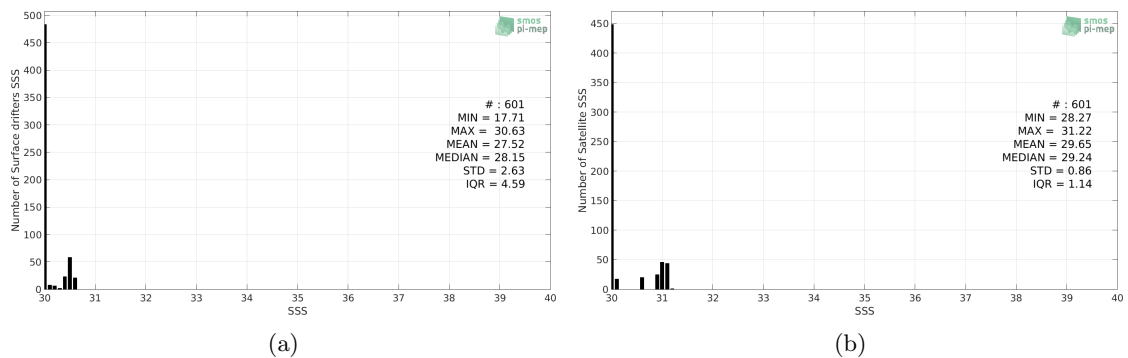
Figure 2: Histograms of SSS from Surface drifters (a) and SMAP-L3-JPL-V4.3-MONTHLY-60KM (b) considering all match-up pairs per bins of 0.1 over the Amazon and Orinoco river plumes Pi-MEP region and for the full satellite product period.
