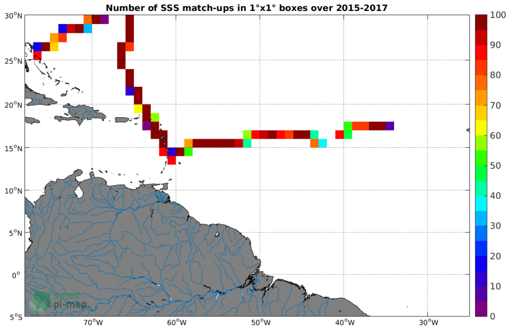
Figure 4: Number of SSS match-ups between TSG-GOSUD-Sailing-ship SSS and the SMAP-L3-JPL-V4.2-8DAY-RUNNING-60KM SSS product for the Amazon and Orinoco river plumes Pi-MEP region over 1^{\circ} \times 1^{\circ} boxes and for the full satellite product period.
