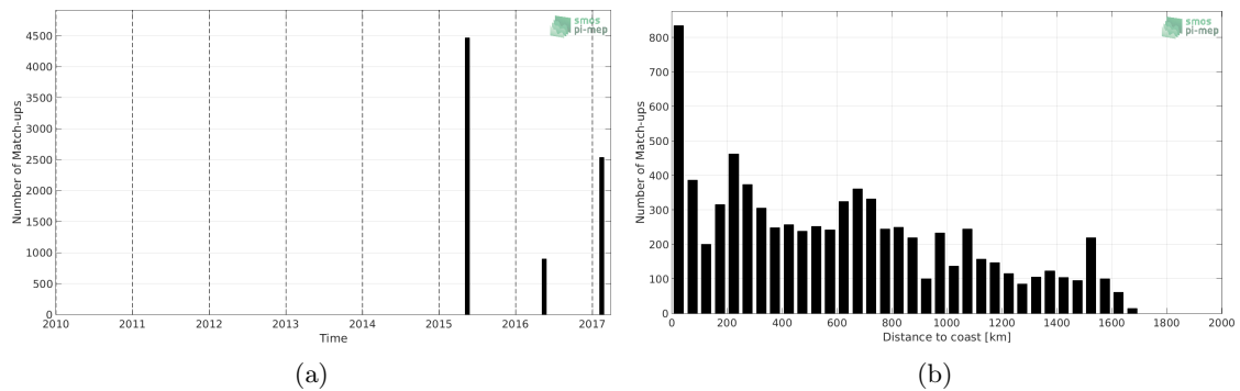
Figure 1: Number of match-ups between TSG-GOSUD-Sailing-ship and SMAP-L3-JPL-V4.2-8DAY-RUNNING-60KM SSS as a function of time (a) and as function of the distance to coast (b) over the Amazon and Orinoco river plumes Pi-MEP region and for the full satellite product period.
