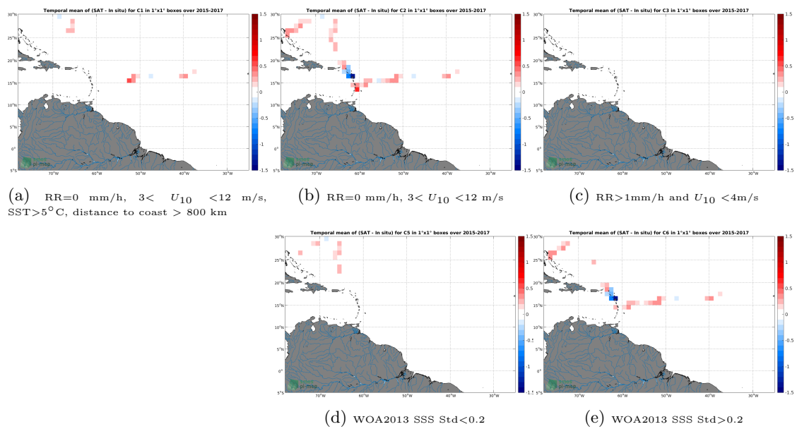
Figure 12: Temporal mean gridded over spatial boxes of size 1^\circ \times 1^\circ of \Delta SSS (SMAP-L3-JPL-V4.2-8DAY-RUNNING-60KM - TSG-GOSUD-Sailing-ship) for 5 different subdatasets corresponding to:RR=0 mm/h, 3 < U_{10} < 12 m/s, SST >5^\circ C, distance to coast > 800 km (a), RR=0 mm/h, 3 < U_{10} < 12 m/s (b), RR >1 mm/h and U_{10} < 4 m/s (c), WOA2013 SSS Std <0.2 (d), WOA2013 SSS Std >0.2 (e).
