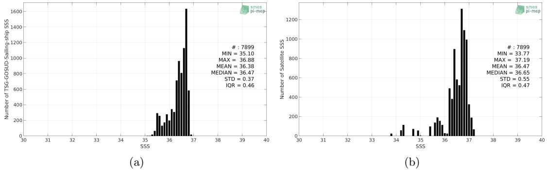
Figure 2: Histograms of SSS from TSG-GOSUD-Sailing-ship (a) and SMAP-L3-JPL-V4.2-8DAY-RUNNING-60KM (b) considering all match-up pairs per bins of 0.1 over the Amazon and Orinoco river plumes Pi-MEP region and for the full satellite product period.
