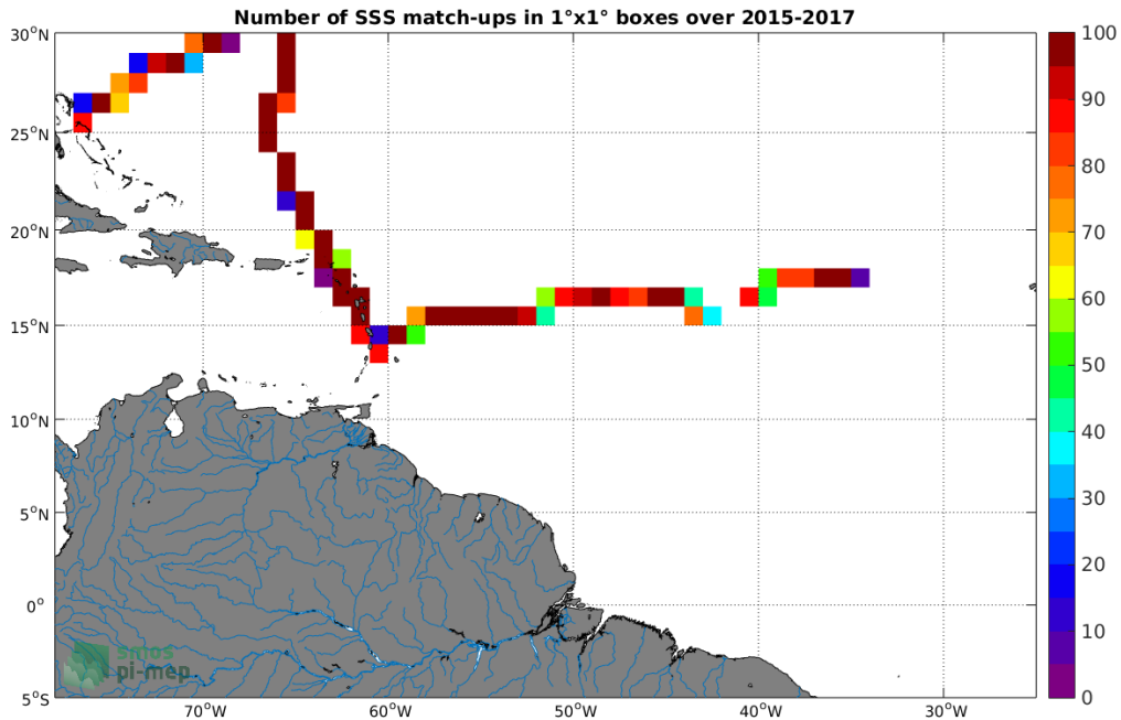
Figure 4: Number of SSS match-ups between TSG-GOSUD-Sailing-ship SSS and the SMAP-L3-JPL-V4.2-8DAY-RUNNING-60KM SSS product for the Amazon and Orinoco river plumes Pi-MEP region over 1^\circ \times 1^\circ boxes and for the full satellite product period.
