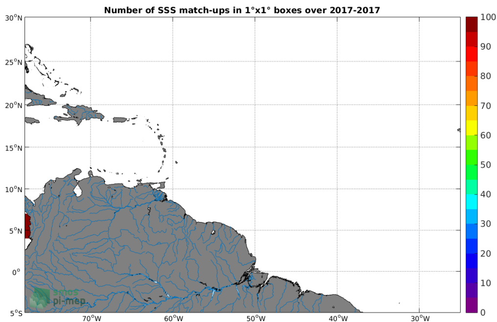
Figure 3: Number of SSS match-ups between Surface drifters SSS and the SMAP-L3-JPL-V4.2-8DAY-RUNNING-60KM SSS product for the Amazon and Orinoco river plumes Pi-MEP region over 1^\circ \times 1^\circ boxes and for the full satellite product period.
