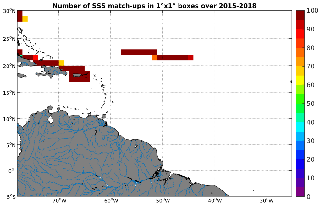
Figure 4: Number of SSS match-ups between TSG-SAMOS SSS and the SMAP-L3-JPL-V4-8DAY-RUNNING-60KM SSS product for the Amazon and Orinoco river plumes Pi-MEP region over 1°x1° boxes and for the full satellite product period.
