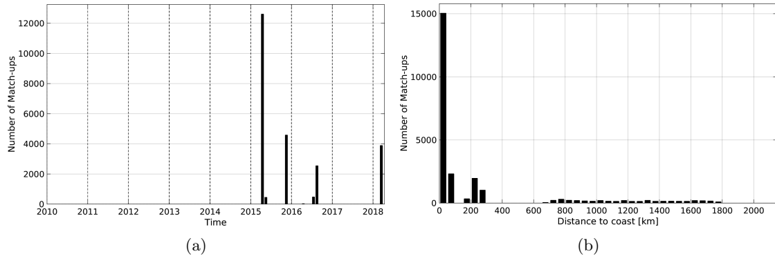
Figure 1: Number of match-ups between TSG-SAMOS and SMAP-L3-JPL-V4-8DAY-RUNNING-60KM SSS as a function of time (a) and as function of the distance to coast (b) over the Amazon and Orinoco river plumes Pi-MEP region and for the full satellite product period.
