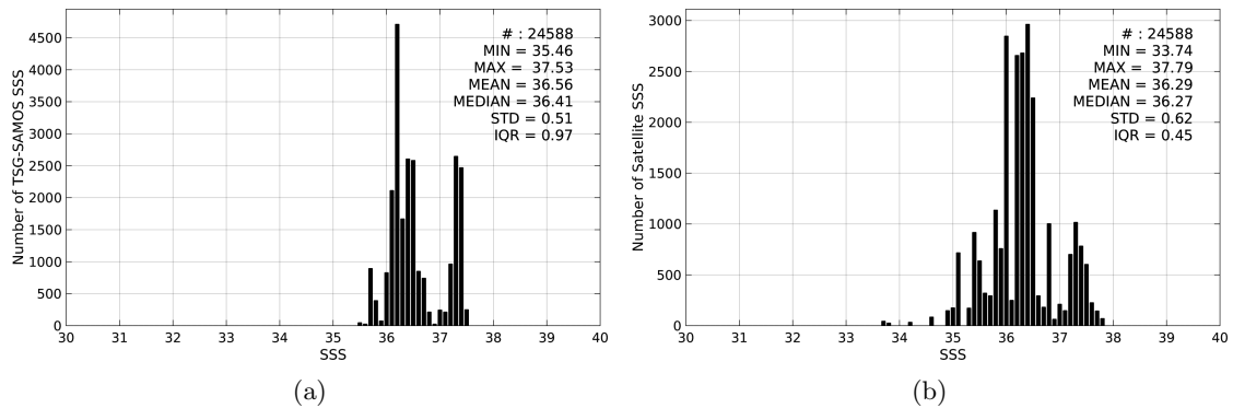
Figure 2: Histograms of SSS from TSG-SAMOS (a) and SMAP-L3-JPL-V4-8DAY-RUNNING-60KM (b) considering all match-up pairs per bins of 0.1 over the Amazon and Orinoco river plumes Pi-MEP region and for the full satellite product period.
