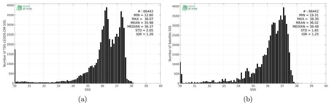
Figure 2: Histograms of SSS from TSG-LEGOS-DM (a) and SMAP-L3-JPL-V4-8DAY-RUNNING-60KM (b) considering all match-up pairs per bins of 0.1 over the Amazon and Orinoco river plumes Pi-MEP region and for the full satellite product period.
