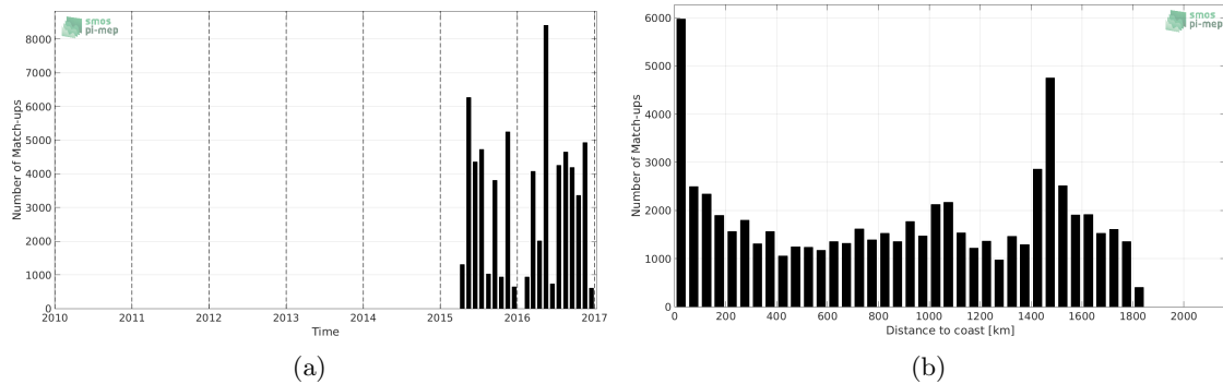
Figure 1: Number of match-ups between TSG-LEGOS-DM and SMAP-L3-JPL-V4-8DAY-RUNNING-60KM SSS as a function of time (a) and as function of the distance to coast (b) over the Amazon and Orinoco river plumes Pi-MEP region and for the full satellite product period.
