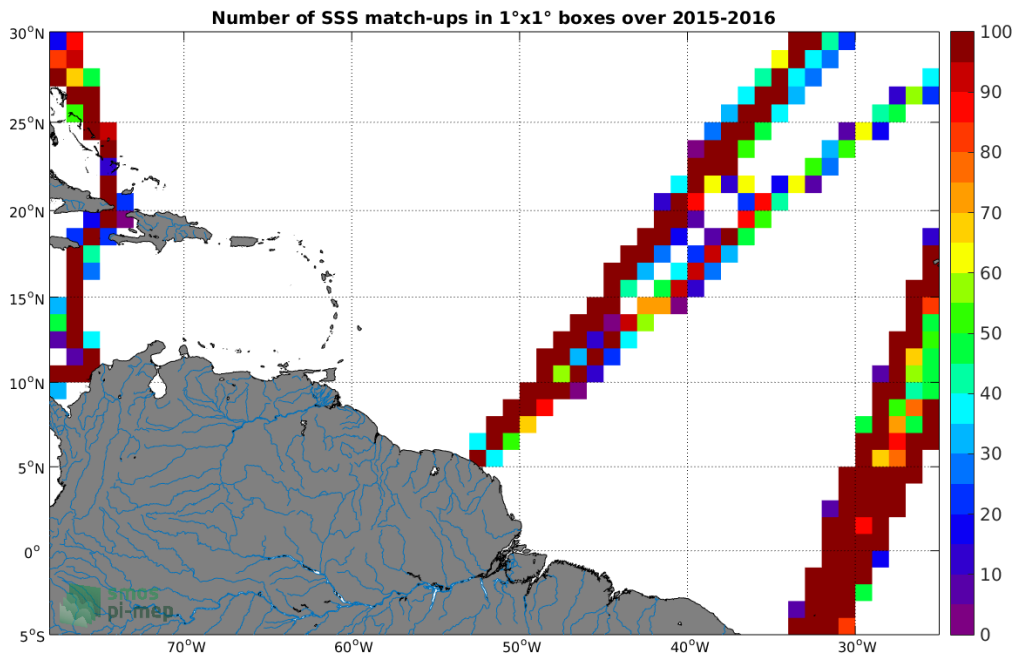
Figure 4: Number of SSS match-ups between TSG-LEGOS-DM SSS and the SMAP-L3-JPL-V4-8DAY-RUNNING-60KM SSS product for the Amazon and Orinoco river plumes Pi-MEP region over 1^\circ \times 1^\circ boxes and for the full satellite product period.
