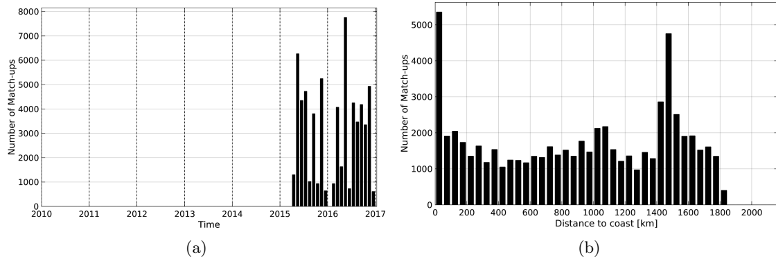
Figure 1: Number of match-ups between TSG-LEGOS-DM and SMAP-L3-JPL-V4-8DAY-RUNNING-60KM SSS as a function of time (a) and as function of the distance to coast (b) over the Amazon and Orinoco river plumes Pi-MEP region and for the full satellite product period.
