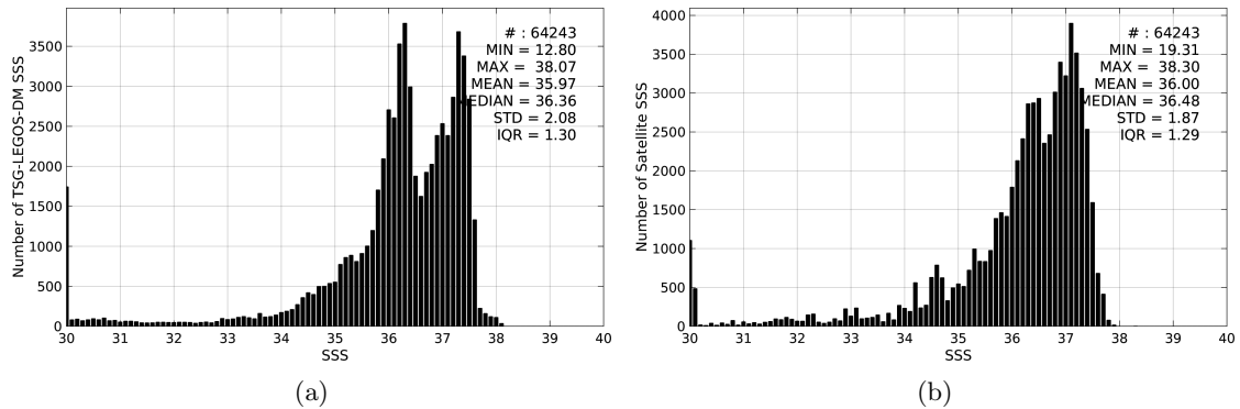
Figure 2: Histograms of SSS from TSG-LEGOS-DM (a) and SMAP-L3-JPL-V4-8DAY-RUNNING-60KM (b) considering all match-up pairs per bins of 0.1 over the Amazon and Orinoco river plumes Pi-MEP region and for the full satellite product period.
