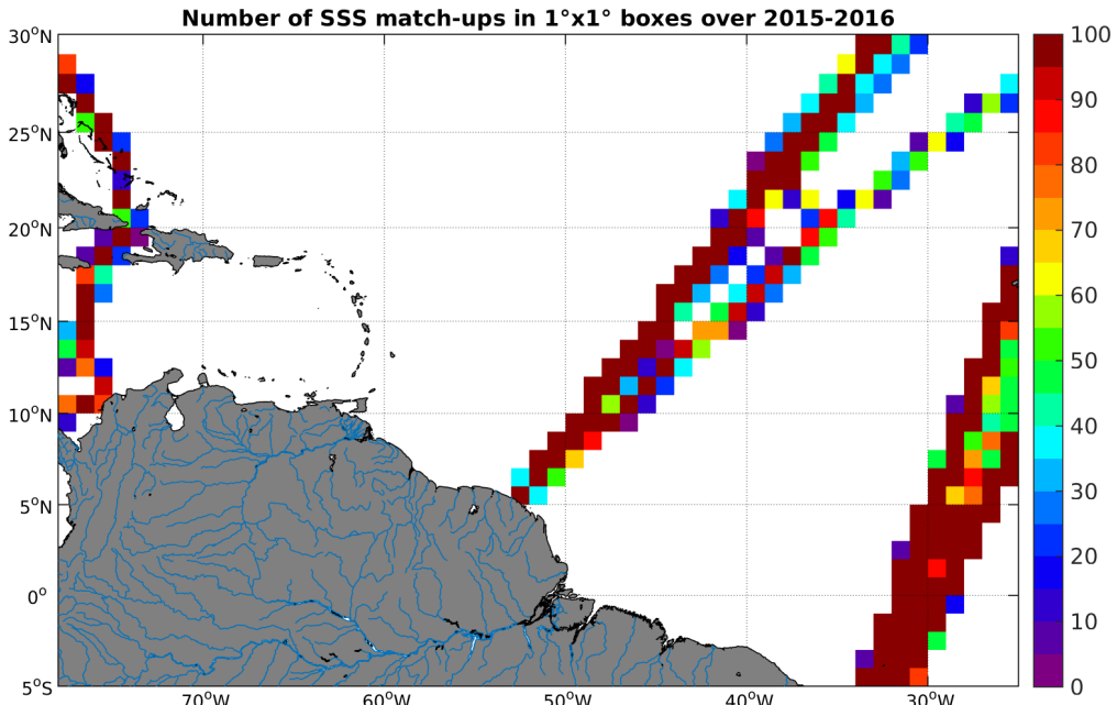
Figure 4: Number of SSS match-ups between TSG-LEGOS-DM SSS and the SMAP-L3-JPL-V4-8DAY-RUNNING-60KM SSS product for the Amazon and Orinoco river plumes Pi-MEP region over 1°x1° boxes and for the full satellite product period.
