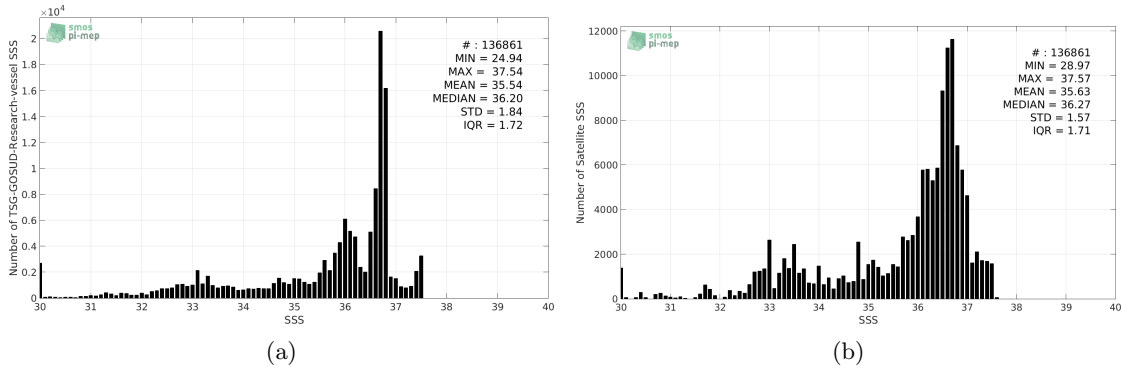
Figure 2: Histograms of SSS from TSG-GOSUD-Research-vessel (a) and SMAP-L3-JPL-V4-8DAY-RUNNING-60KM (b) considering all match-up pairs per bins of 0.1 over the Amazon and Orinoco river plumes Pi-MEP region and for the full satellite product period.
