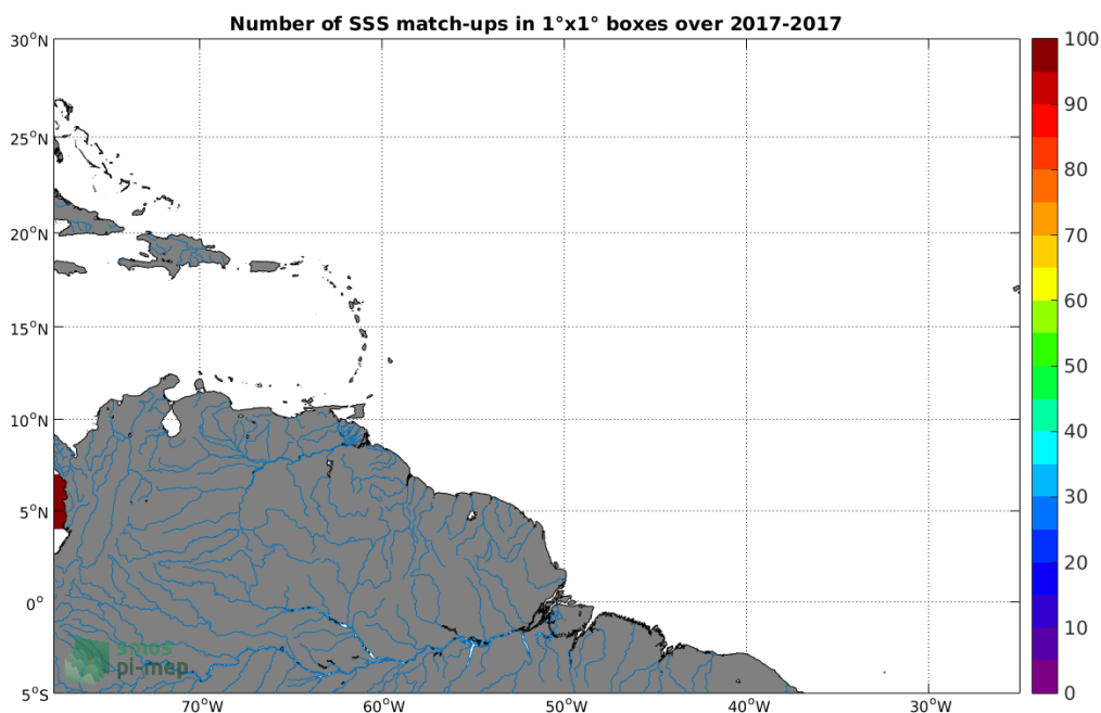
Figure 3: Number of SSS match-ups between Surface drifters SSS and the SMAP-L3-JPL-V4-8DAY-RUNNING-60KM SSS product for the Amazon and Orinoco river plumes Pi-MEP region over 1^\circ \times 1^\circ boxes and for the full satellite product period.
