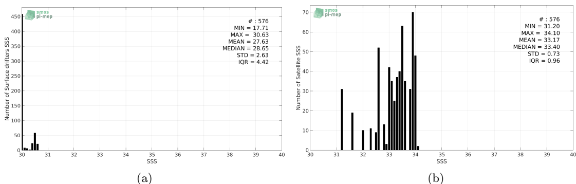
Figure 2: Histograms of SSS from Surface drifters (a) and SMAP-L3-JPL-V4-8DAY-RUNNING-60KM (b) considering all match-up pairs per bins of 0.1 over the Amazon and Orinoco river plumes Pi-MEP region and for the full satellite product period.
