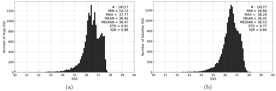
Figure 2: Histograms of SSS from Argo (a) and SMAP-L3-JPL-V4-8DAY-RUNNING-60KM (b) considering all match-up pairs per bins of 0.1 over the Amazon and Orinoco river plumes Pi-MEP region and for the full satellite product period.
