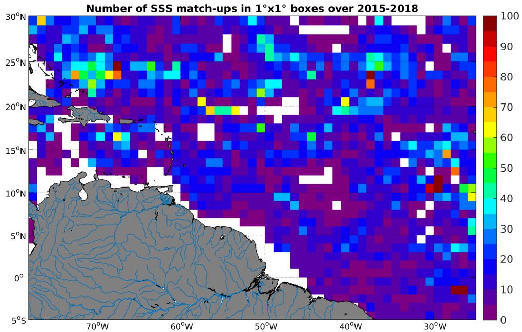
Figure 4: Number of SSS match-ups between Argo SSS and the SMAP-L3-JPL-V4-8DAY-RUNNING-60KM SSS product for the Amazon and Orinoco river plumes Pi-MEP region over 1^\circ \times 1^\circ boxes and for the full satellite product period.
