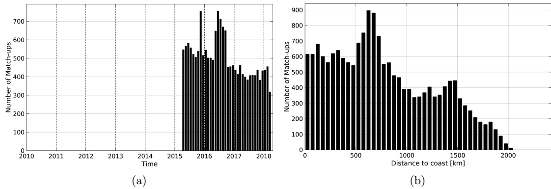
Figure 1: Number of match-ups between Argo and SMAP-L3-JPL-V4-8DAY-RUNNING-60KM SSS as a function of time (a) and as function of the distance to coast (b) over the Amazon and Orinoco river plumes Pi-MEP region and for the full satellite product period.
