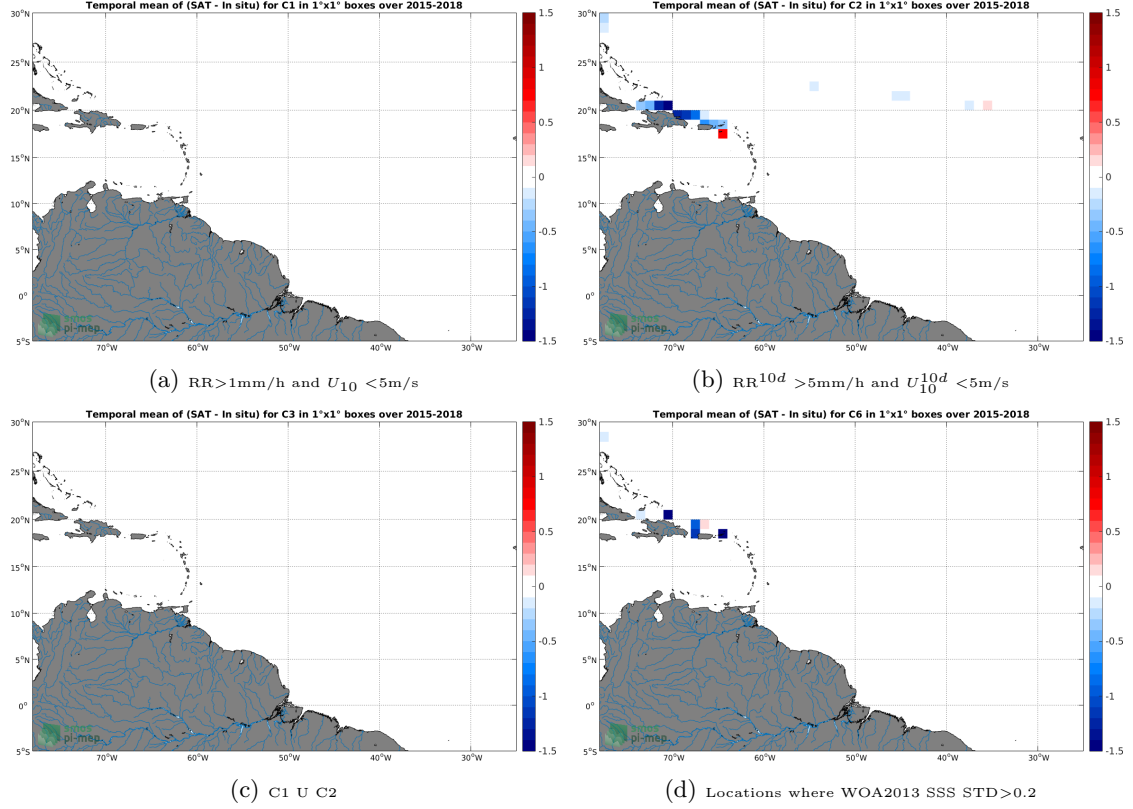
Figure 12: Temporal mean gridded over spatial boxes of size 1^\circ \times 1^\circ of \Delta SSS (SMAP-L3-JPL-V4-MONTHLY-60KM - TSG-SAMOS) for 4 different subdatasets corresponding to: RR > 1\text{mm/h} and U_{10} < 5\text{m/s} (a), RR^{10d} > 5\text{mm/h} and U_{10}^{10d} < 5\text{m/s} (b), C1 U C2 (c), Locations where WOA2013 SSS STD > 0.2 (d).
