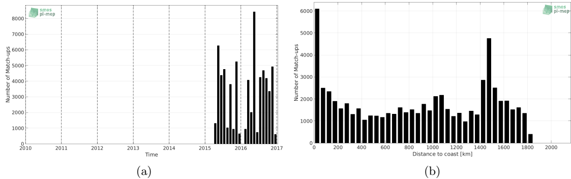
Figure 1: Number of match-ups between TSG-LEGOS-DM and SMAP-L3-JPL-V4-MONTHLY-60KM SSS as a function of time (a) and as function of the distance to coast (b) over the Amazon and Orinoco river plumes Pi-MEP region and for the full satellite product period.
