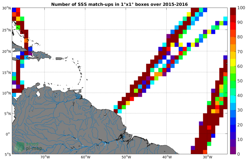
Figure 4: Number of SSS match-ups between TSG-LEGOS-DM SSS and the SMAP-L3-JPL-V4-MONTHLY-60KM SSS product for the Amazon and Orinoco river plumes Pi-MEP region over 1^\circ \times 1^\circ boxes and for the full satellite product period.
