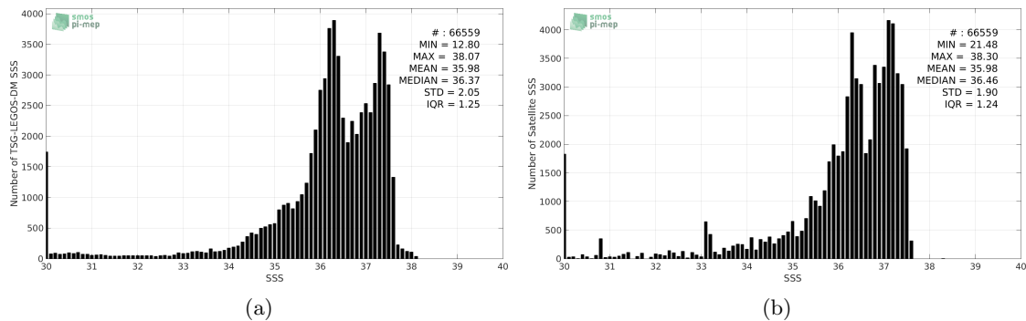
Figure 2: Histograms of SSS from TSG-LEGOS-DM (a) and SMAP-L3-JPL-V4-MONTHLY-60KM (b) considering all match-up pairs per bins of 0.1 over the Amazon and Orinoco river plumes Pi-MEP region and for the full satellite product period.
