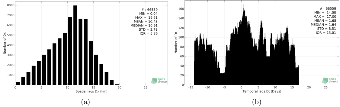
Figure 5: Histograms of the spatial (a) and temporal (b) lags between the time of the TSG-LEGOS-DM measurements and the date of the corresponding SMAP-L3-JPL-V4-MONTHLY-60KM SSS product.
