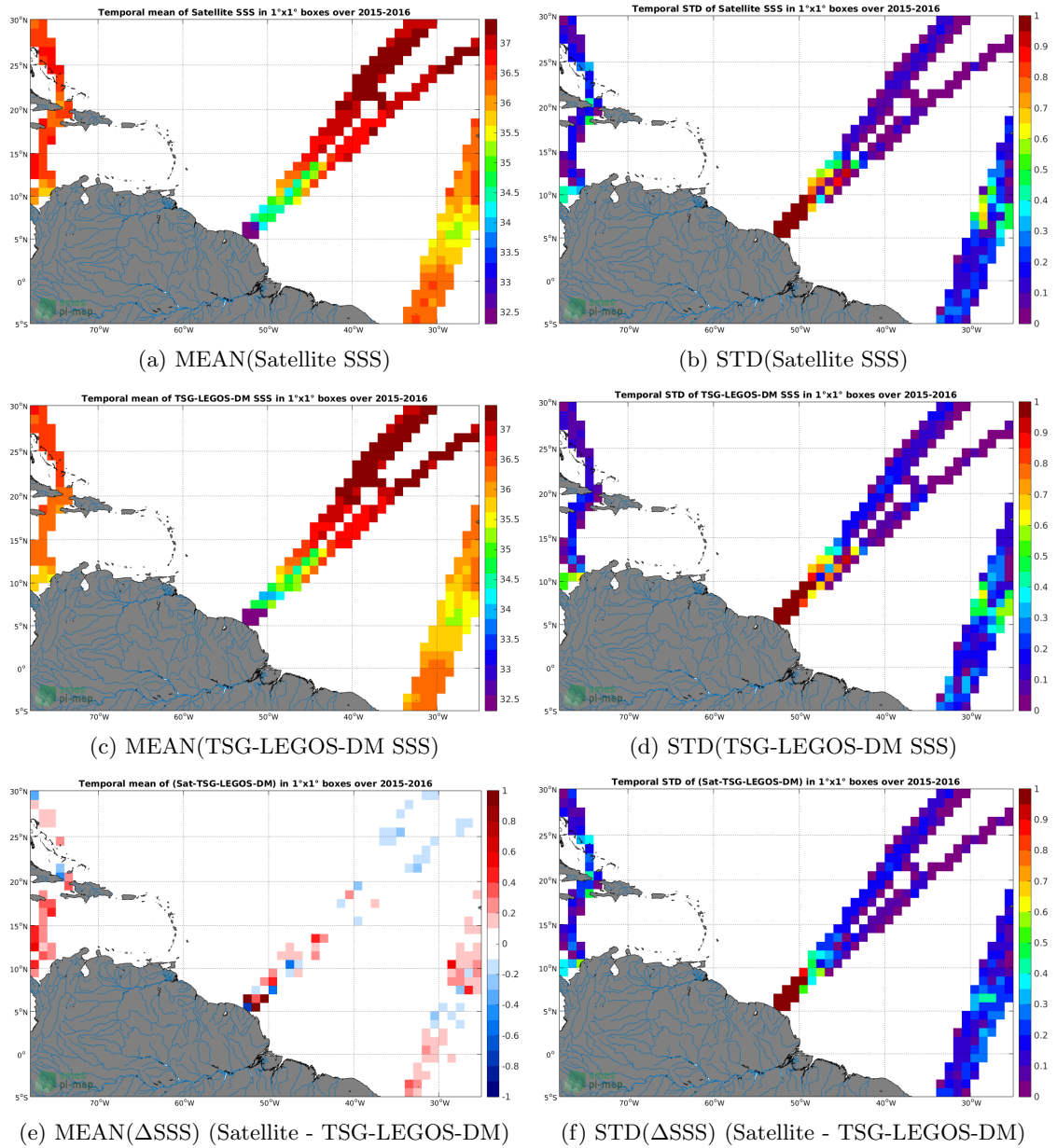
Figure 6: Temporal mean (left) and STD (right) of SSS from SMAP-L3-JPL-V4-MONTHLY-60KM (top), TSG-LEGOS-DM (middle), and of \Delta SSS (Satellite - TSG-LEGOS-DM). Only match-up pairs are used to generate these maps.
