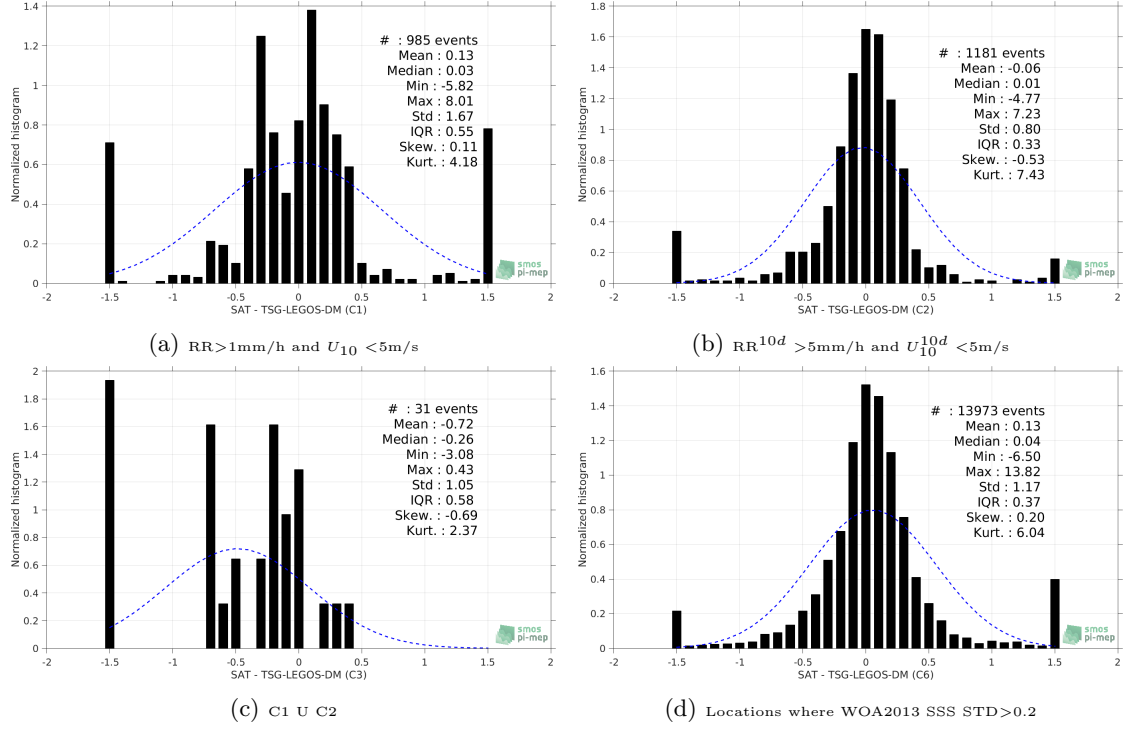
Figure 13: Normalized histogram of \Delta SSS (SMAP-L3-JPL-V4-MONTHLY-60KM - TSG-LEGOS-DM) for 6 different subdatasets corresponding to: RR > 1mm/h and U_{10} < 5 m/s (a), RR^{10d} > 5 mm/h and U_{10}^{10d} < 5 m/s (b), C1 U C2 (c), Locations where WOA2013 SSS STD > 0.2 (d).
