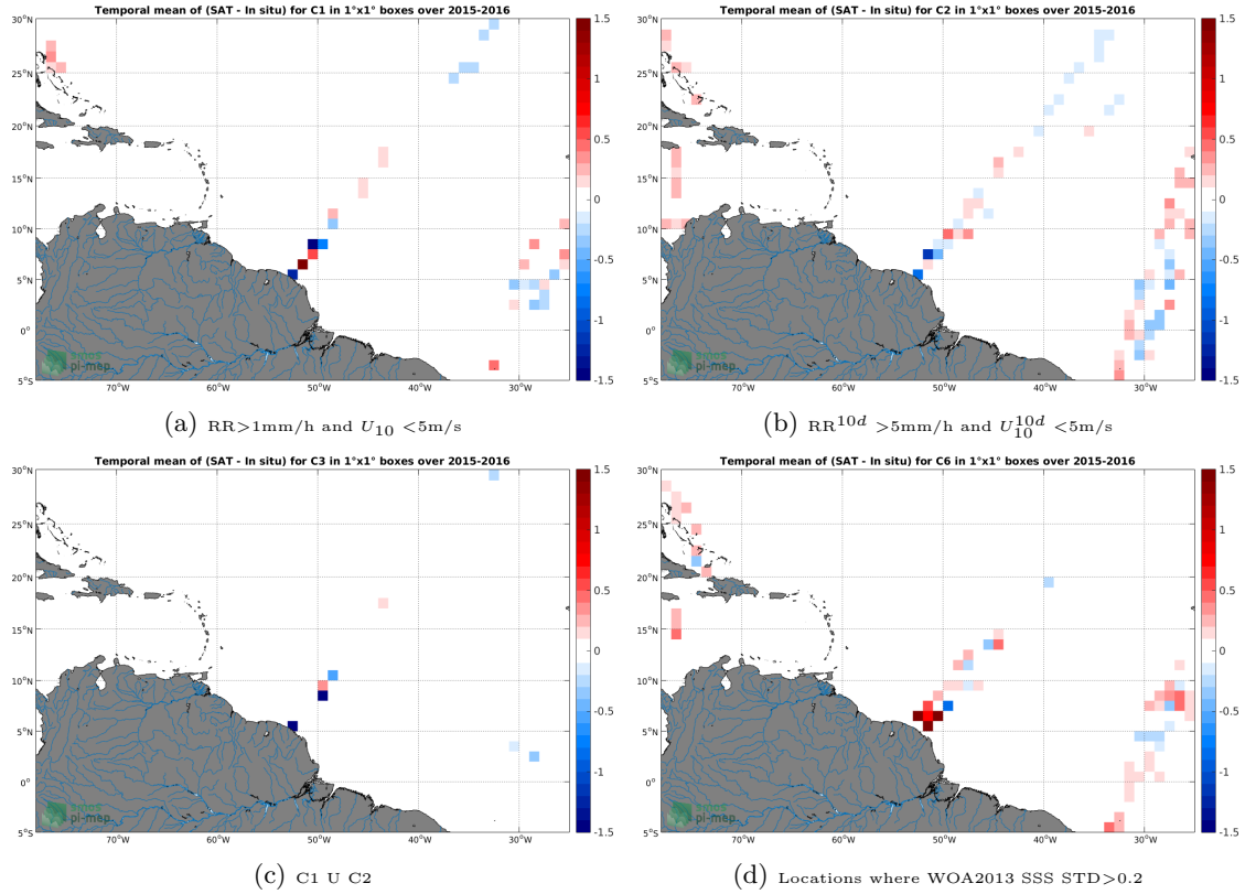
Figure 12: Temporal mean gridded over spatial boxes of size 1^\circ \times 1^\circ of \Delta SSS (SMAP-L3-JPL-V4-MONTHLY-60KM - TSG-LEGOS-DM) for 4 different subdatasets corresponding to: RR > 1\text{mm/h} and U_{10} < 5\text{m/s} (a), RR^{10d} > 5\text{mm/h} and U_{10}^{10d} < 5\text{m/s} (b), C1 U C2 (c), Locations where WOA2013 SSS STD > 0.2 (d).
