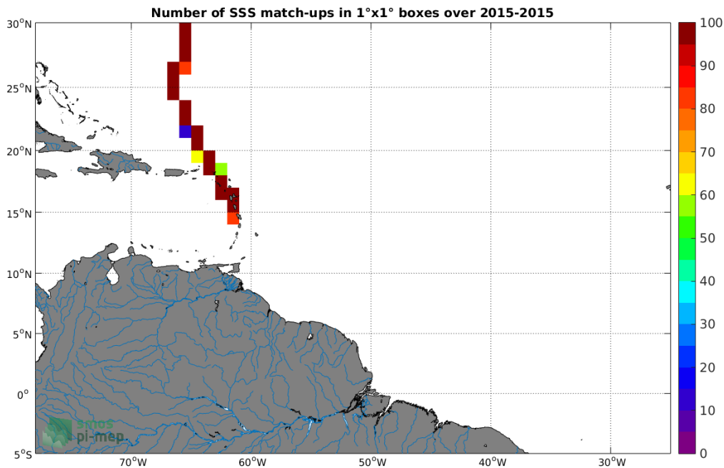
Figure 4: Number of SSS match-ups between TSG-GOSUD-Sailing-ship SSS and the SMAP-L3-JPL-V4-MONTHLY-60KM SSS product for the Amazon and Orinoco river plumes Pi-MEP region over 1^{\circ} \times 1^{\circ} boxes and for the full satellite product period.
