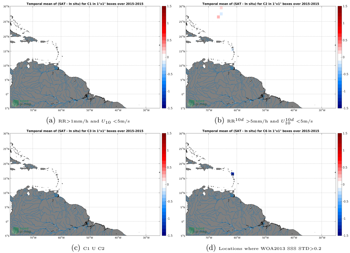
Figure 12: Temporal mean gridded over spatial boxes of size 1^\circ \times 1^\circ of \Delta SSS (SMAP-L3-JPL-V4-MONTHLY-60KM - TSG-GOSUD-Sailing-ship) for 4 different subdatasets corresponding to: RR > 1\text{mm/h} and U_{10} < 5\text{m/s} (a), RR^{10d} > 5\text{mm/h} and U_{10}^{10d} < 5\text{m/s} (b), C1 U C2 (c), Locations where WOA2013 SSS STD > 0.2 (d).
