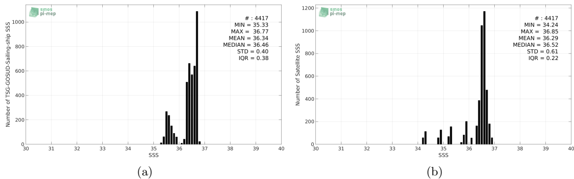
Figure 2: Histograms of SSS from TSG-GOSUD-Sailing-ship (a) and SMAP-L3-JPL-V4-MONTHLY-60KM (b) considering all match-up pairs per bins of 0.1 over the Amazon and Orinoco river plumes Pi-MEP region and for the full satellite product period.
