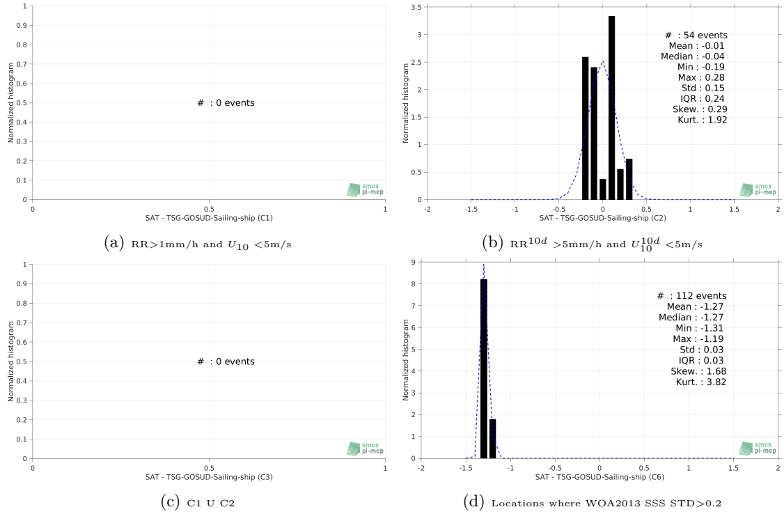
Figure 13: Normalized histogram of \Delta\text{SSS} (SMAP-L3-JPL-V4-MONTHLY-60KM - TSG-GOSUD-Sailing-ship) for 6 different subdatasets corresponding to: RR > 1\text{mm/h} and U_{10} < 5\text{m/s} (a), RR^{10d} > 5\text{mm/h} and U_{10}^{10d} < 5\text{m/s} (b), C1 U C2 (c), Locations where WOA2013 SSS STD > 0.2 (d).
