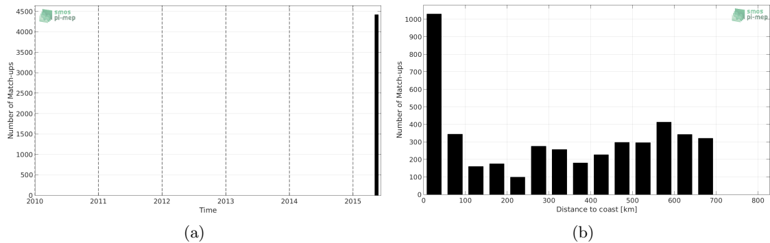
Figure 1: Number of match-ups between TSG-GOSUD-Sailing-ship and SMAP-L3-JPL-V4-MONTHLY-60KM SSS as a function of time (a) and as function of the distance to coast (b) over the Amazon and Orinoco river plumes Pi-MEP region and for the full satellite product period.
