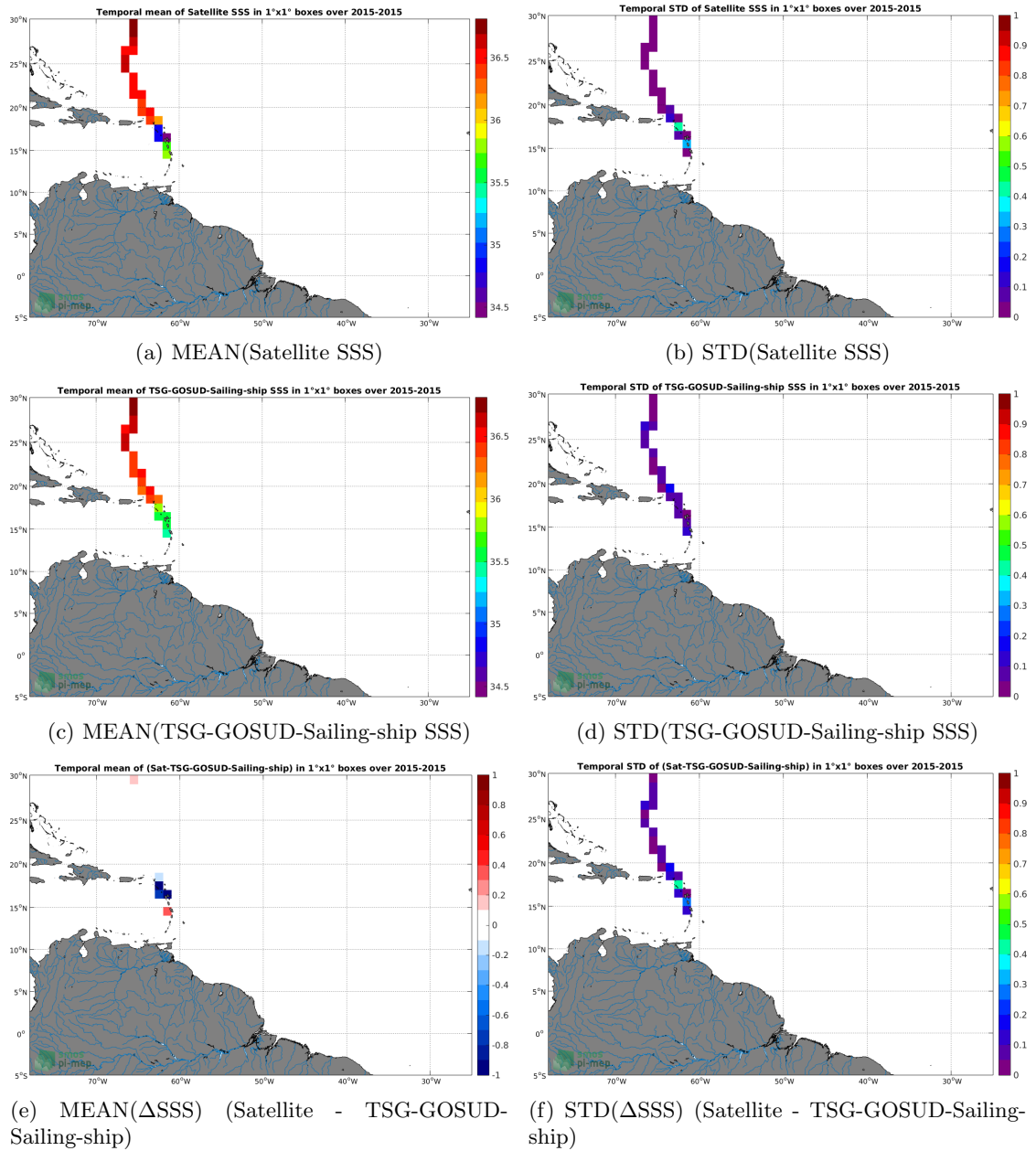
Figure 6: Temporal mean (left) and STD (right) of SSS from SMAP-L3-JPL-V4-MONTHLY-60KM (top), TSG-GOSUD-Sailing-ship (middle), and of \Delta SSS (Satellite - TSG-GOSUD-Sailing-ship). Only match-up pairs are used to generate these maps.
