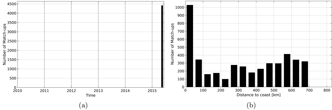
Figure 1: Number of match-ups between TSG-GOSUD-Sailing-ship and SMAP-L3-JPL-V4-MONTHLY-60KM SSS as a function of time (a) and as function of the distance to coast (b) over the Amazon and Orinoco river plumes Pi-MEP region and for the full satellite product period.
