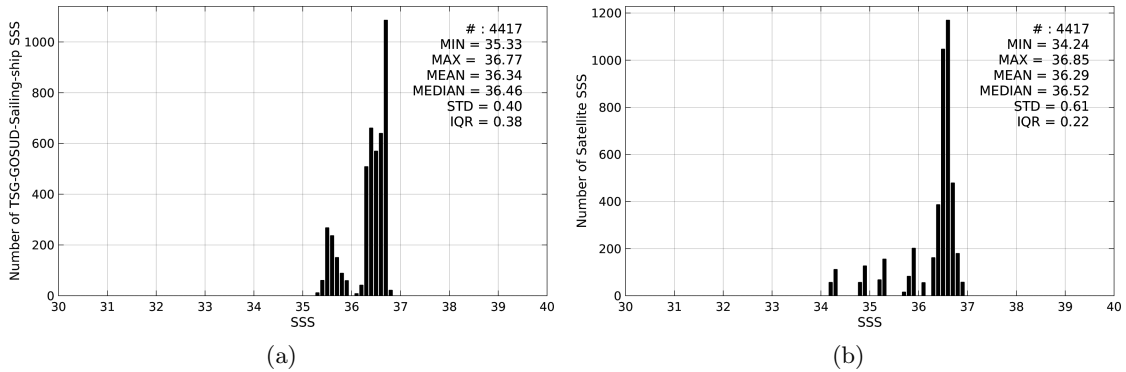
Figure 2: Histograms of SSS from TSG-GOSUD-Sailing-ship (a) and SMAP-L3-JPL-V4-MONTHLY-60KM (b) considering all match-up pairs per bins of 0.1 over the Amazon and Orinoco river plumes Pi-MEP region and for the full satellite product period.
