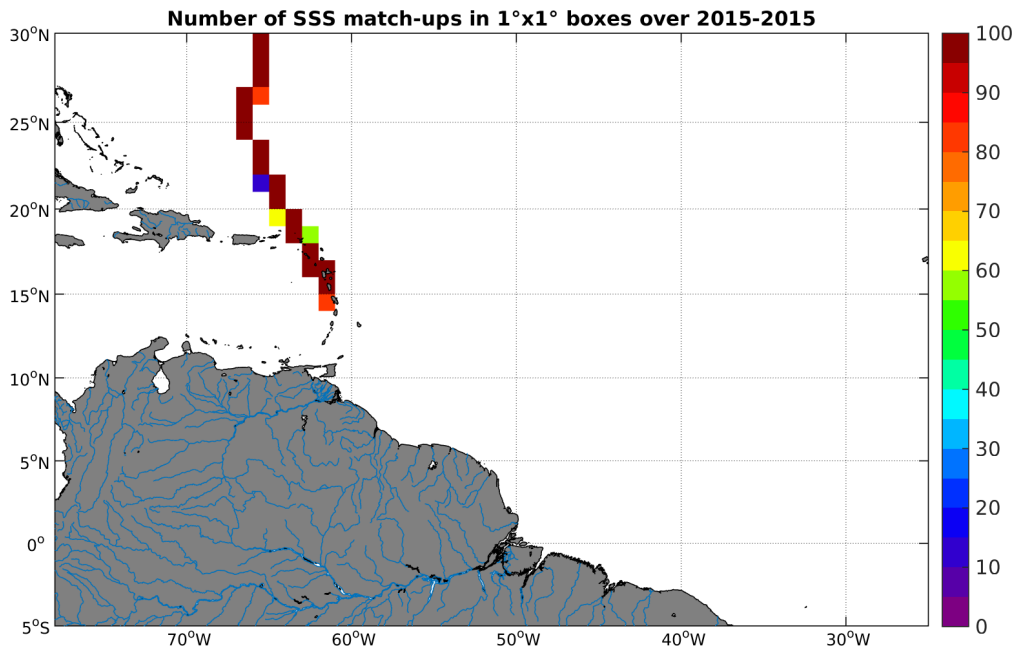
Figure 4: Number of SSS match-ups between TSG-GOSUD-Sailing-ship SSS and the SMAP-L3-JPL-V4-MONTHLY-60KM SSS product for the Amazon and Orinoco river plumes Pi-MEP region over 1^\circ \times 1^\circ boxes and for the full satellite product period.
