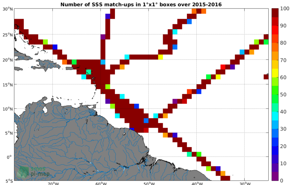
Figure 4: Number of SSS match-ups between TSG-GOSUD-Research-vessel SSS and the SMAP-L3-JPL-V4-MONTHLY-60KM SSS product for the Amazon and Orinoco river plumes Pi-MEP region over 1°x1° boxes and for the full satellite product period.
