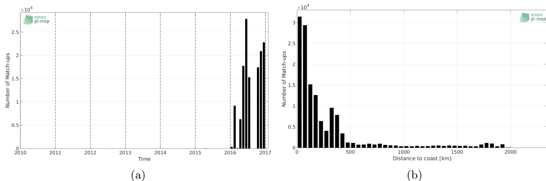
Figure 1: Number of match-ups between TSG-GOSUD-Research-vessel and SMAP-L3-JPL-V4-MONTHLY-60KM SSS as a function of time (a) and as function of the distance to coast (b) over the Amazon and Orinoco river plumes Pi-MEP region and for the full satellite product period.
