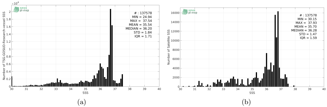
Figure 2: Histograms of SSS from TSG-GOSUD-Research-vessel (a) and SMAP-L3-JPL-V4-MONTHLY-60KM (b) considering all match-up pairs per bins of 0.1 over the Amazon and Orinoco river plumes Pi-MEP region and for the full satellite product period.
