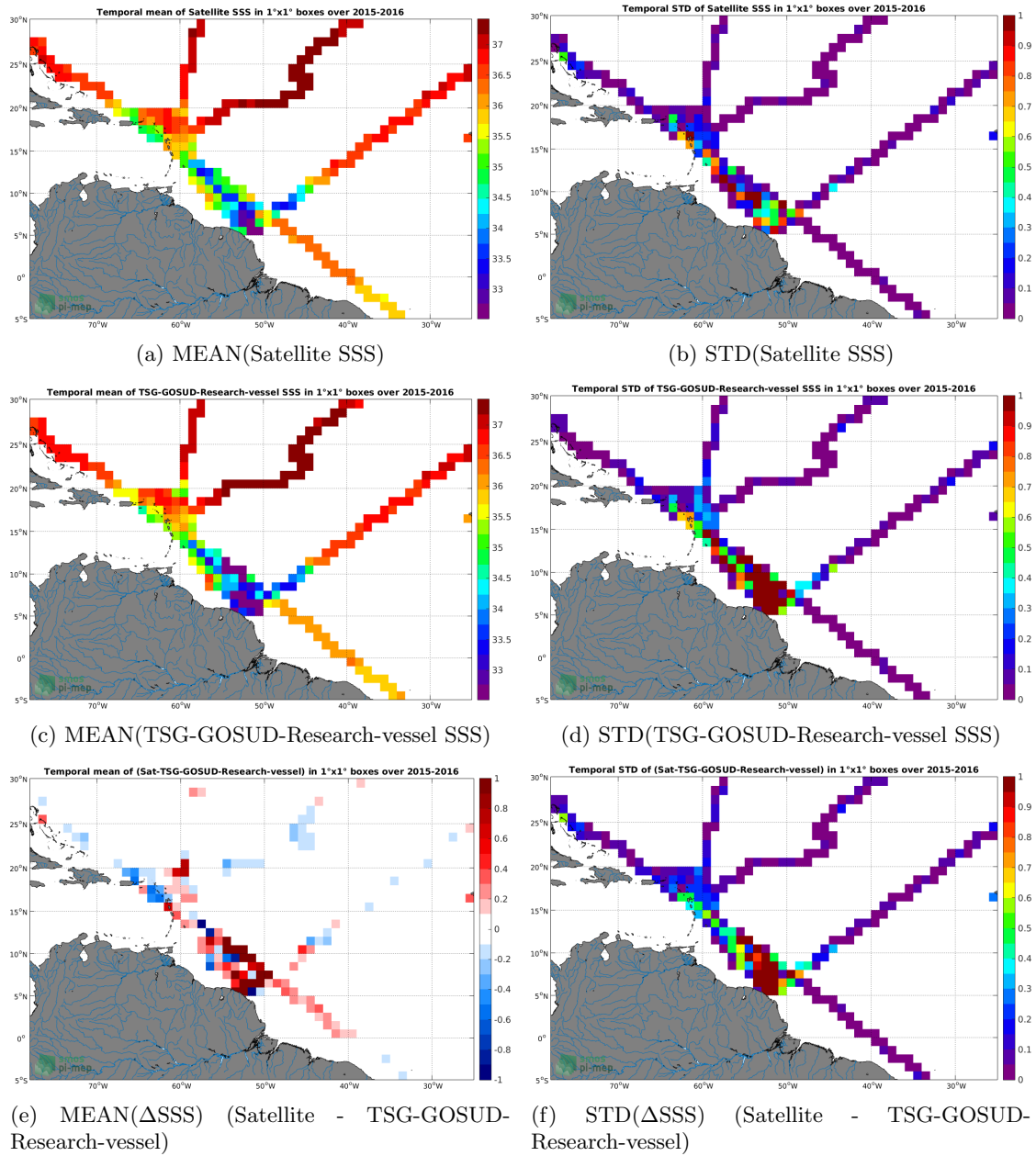
Figure 6: Temporal mean (left) and STD (right) of SSS from SMAP-L3-JPL-V4-MONTHLY-60KM (top), TSG-GOSUD-Research-vessel (middle), and of \Delta SSS (Satellite - TSG-GOSUD-Research-vessel). Only match-up pairs are used to generate these maps.
