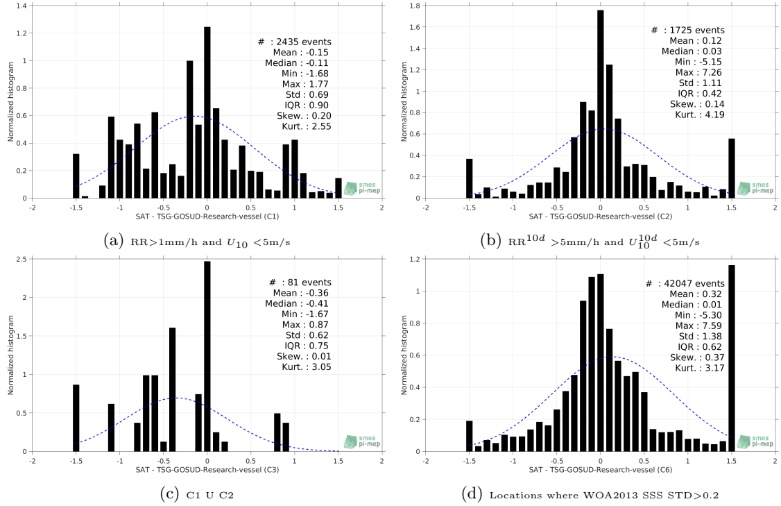
Figure 13: Normalized histogram of \Delta SSS (SMAP-L3-JPL-V4-MONTHLY-60KM - TSG-GOSUD-Research-vessel) for 6 different subdatasets corresponding to: RR > 1\text{mm/h} and U_{10} < 5\text{m/s} (a), RR^{10d} > 5\text{mm/h} and U_{10}^{10d} < 5\text{m/s} (b), C1 U C2 (c), Locations where WOA2013 SSS STD > 0.2 (d).
