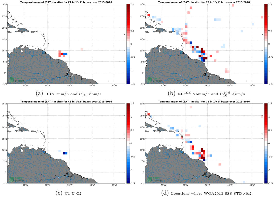
Figure 12: Temporal mean gridded over spatial boxes of size 1^\circ \times 1^\circ of \Delta SSS (SMAP-L3-JPL-V4-MONTHLY-60KM - TSG-GOSUD-Research-vessel) for 4 different subdatasets corresponding to: RR > 1\text{mm/h} and U_{10} < 5\text{m/s} (a), RR^{10d} > 5\text{mm/h} and U_{10}^{10d} < 5\text{m/s} (b), C1 U C2 (c), Locations where WOA2013 SSS STD > 0.2 (d).
