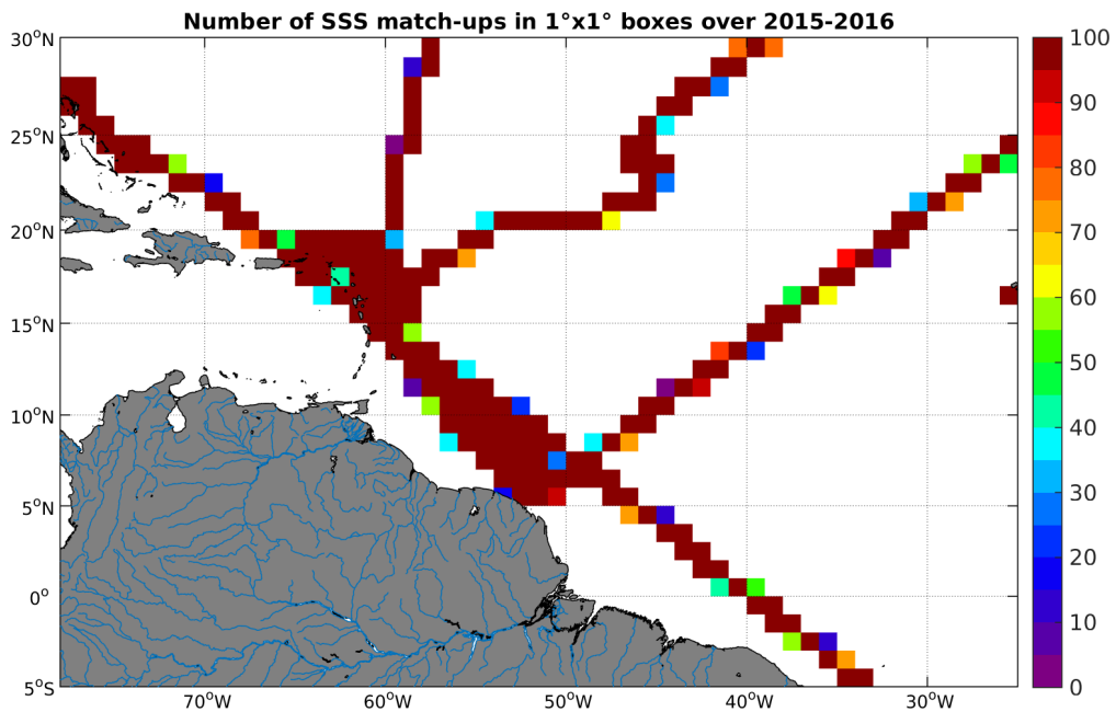
Figure 4: Number of SSS match-ups between TSG-GOSUD-Research-vessel SSS and the SMAP-L3-JPL-V4-MONTHLY-60KM SSS product for the Amazon and Orinoco river plumes Pi-MEP region over 1^\circ \times 1^\circ boxes and for the full satellite product period.
