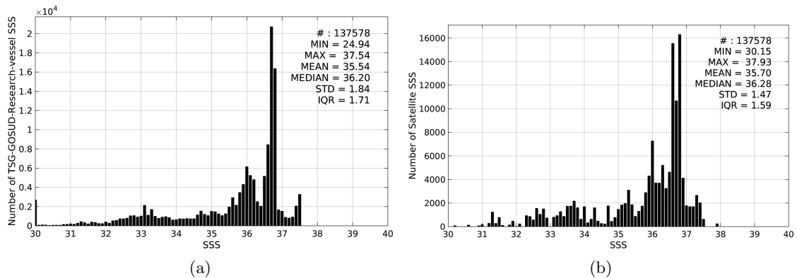
Figure 2: Histograms of SSS from TSG-GOSUD-Research-vessel (a) and SMAP-L3-JPL-V4-MONTHLY-60KM (b) considering all match-up pairs per bins of 0.1 over the Amazon and Orinoco river plumes Pi-MEP region and for the full satellite product period.
