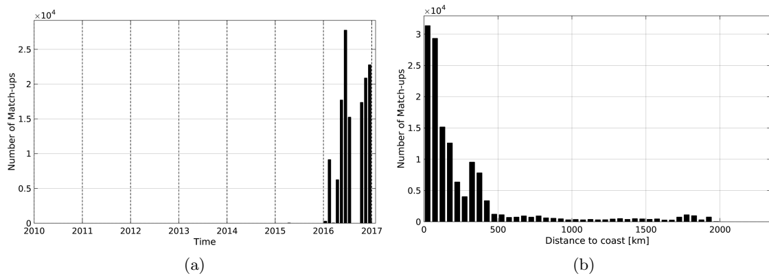
Figure 1: Number of match-ups between TSG-GOSUD-Research-vessel and SMAP-L3-JPL-V4-MONTHLY-60KM SSS as a function of time (a) and as function of the distance to coast (b) over the Amazon and Orinoco river plumes Pi-MEP region and for the full satellite product period.
