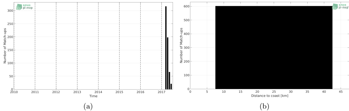
Figure 1: Number of match-ups between Surface drifters and SMAP-L3-JPL-V4-MONTHLY-60KM SSS as a function of time (a) and as function of the distance to coast (b) over the Amazon and Orinoco river plumes Pi-MEP region and for the full satellite product period.
