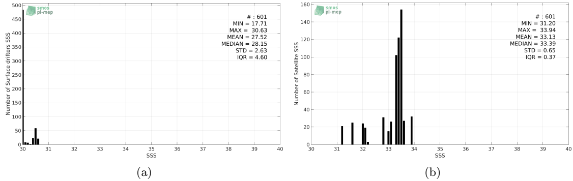
Figure 2: Histograms of SSS from Surface drifters (a) and SMAP-L3-JPL-V4-MONTHLY-60KM (b) considering all match-up pairs per bins of 0.1 over the Amazon and Orinoco river plumes Pi-MEP region and for the full satellite product period.
