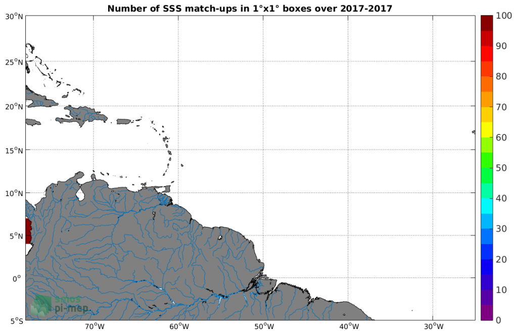
Figure 3: Number of SSS match-ups between Surface drifters SSS and the SMAP-L3-JPL-V4-MONTHLY-60KM SSS product for the Amazon and Orinoco river plumes Pi-MEP region over 1°x1° boxes and for the full satellite product period.
